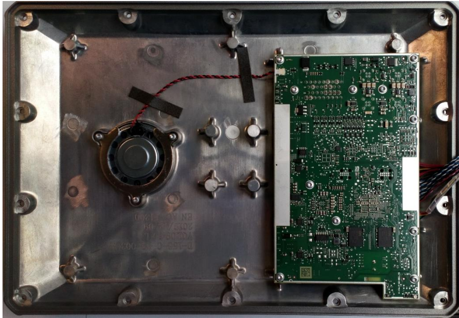
Figure 2: Top view internal I
