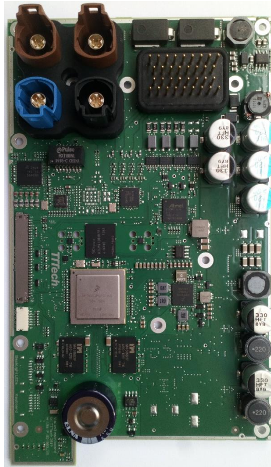
Figure 4: Bottom view PBA Main
