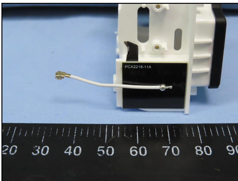
WLAN 2.4GHz+WLAN5GHz+Bluetooth antenna
