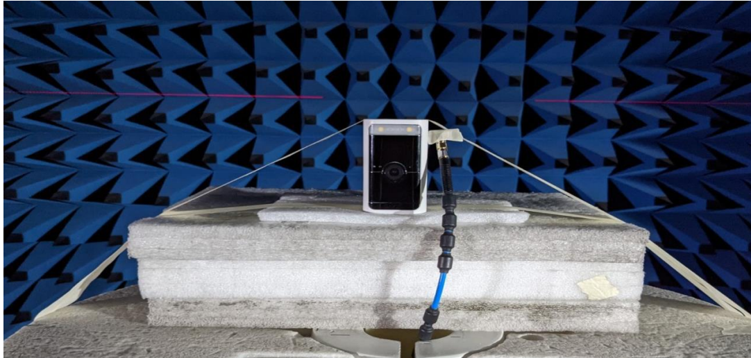
Setup Photo
