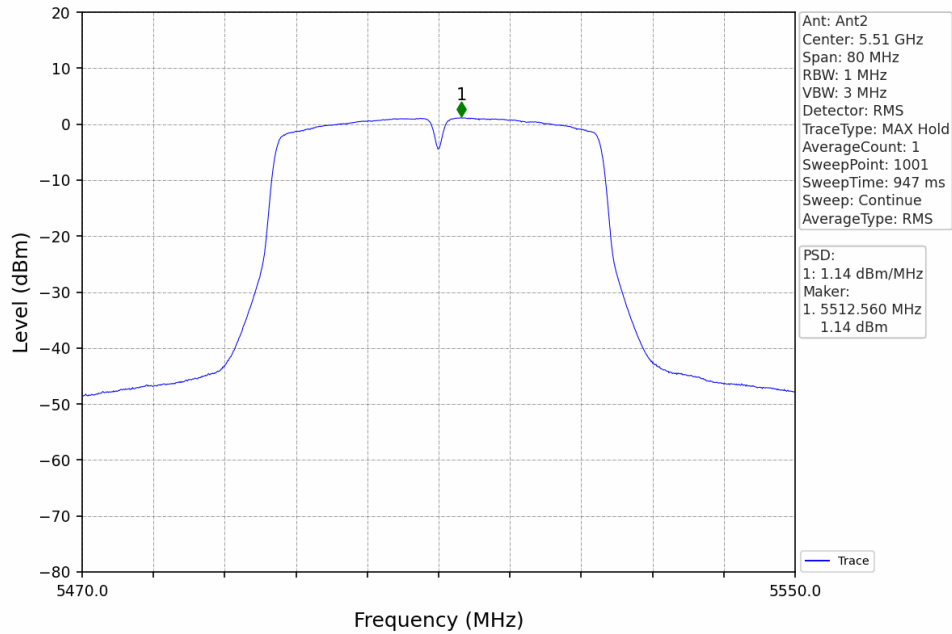
802.11n(HT40)_LCH_5510MHz_MIMO_NTNV
