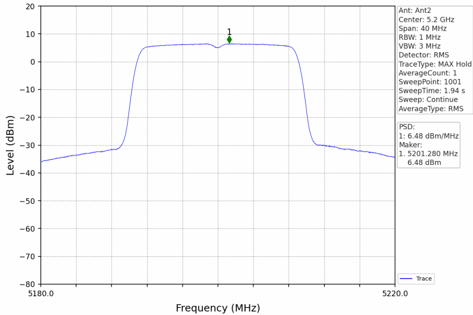
802.11ac(VHT20)_MCH_5200MHz_MIMO_NTNV
