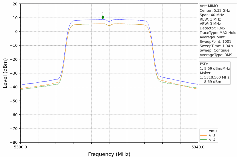
802.11ac(VHT20)_HCH_5320MHz_MIMO_NTNV
