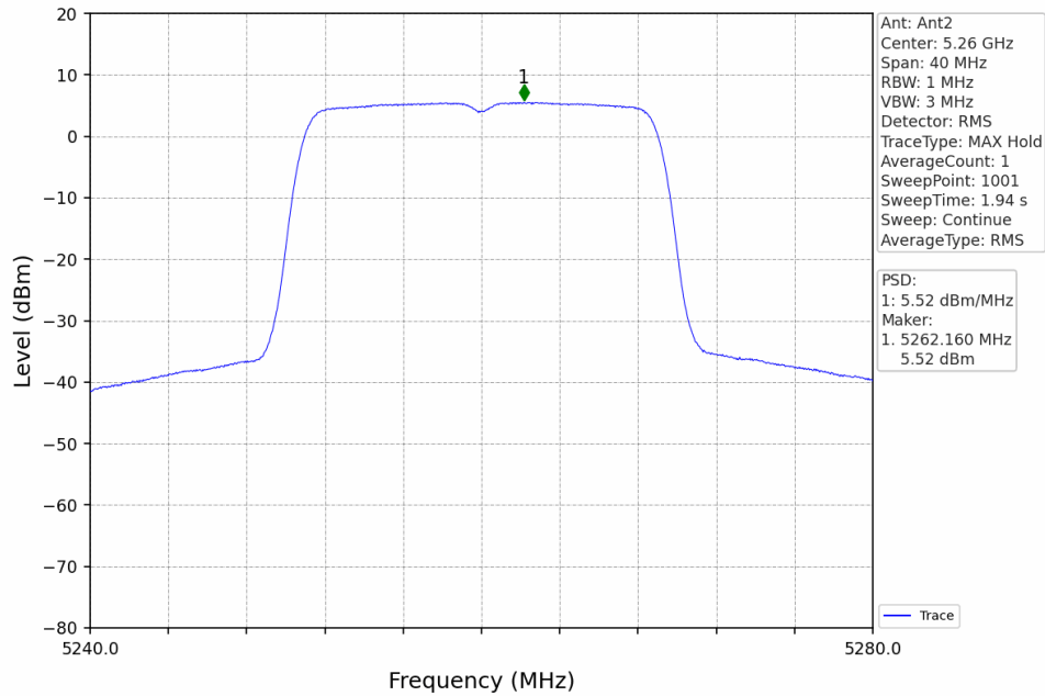
802.11ac(VHT20)_LCH_5260MHz_MIMO_NTNV
