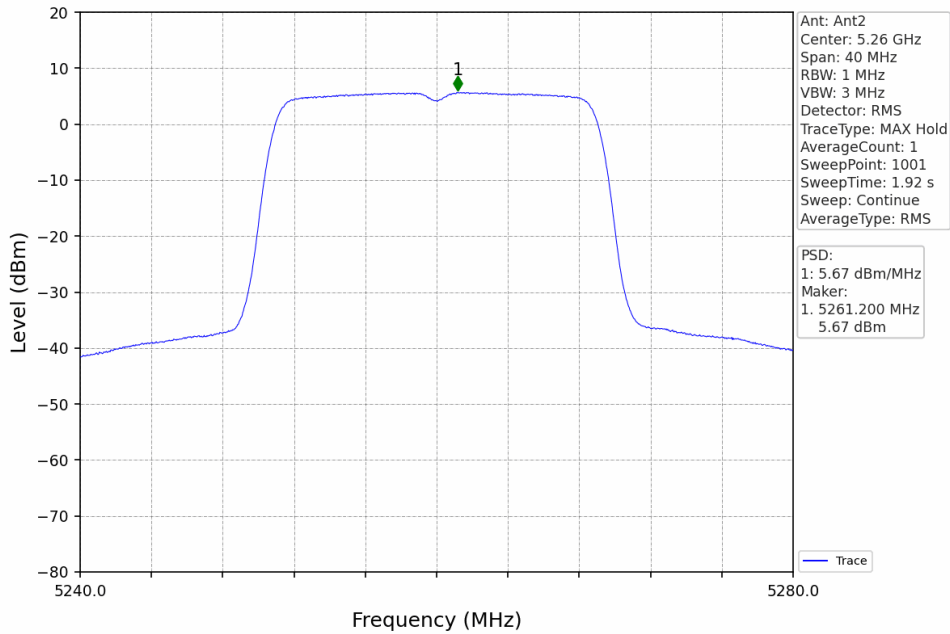
802.11n(HT20)_LCH_5260MHz_MIMO_NTNV
