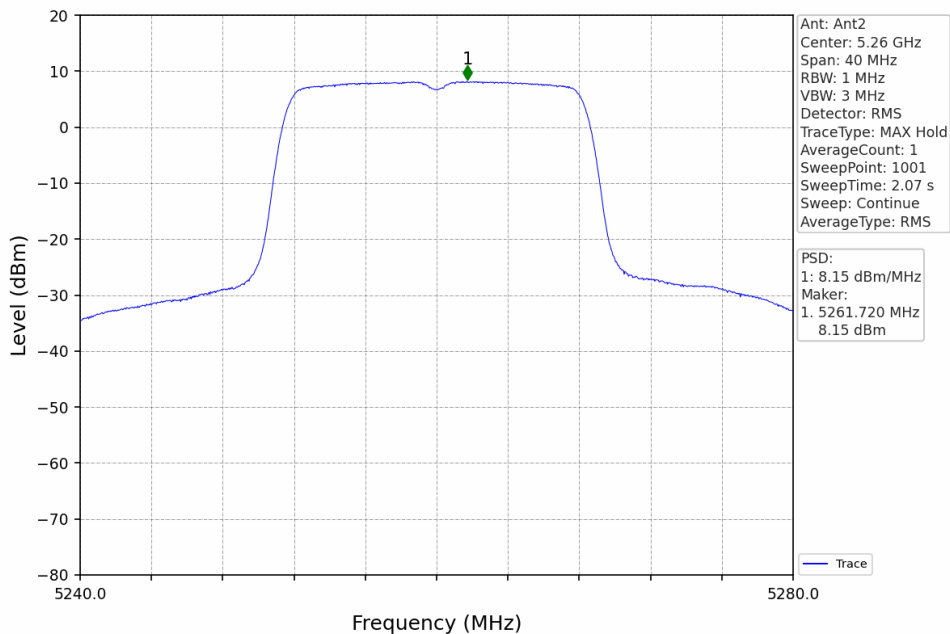
802.11a_LCH_5260MHz_Ant2_NTNV
