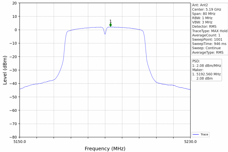
802.11n(HT40)_LCH_5190MHz_MIMO_NTNV
