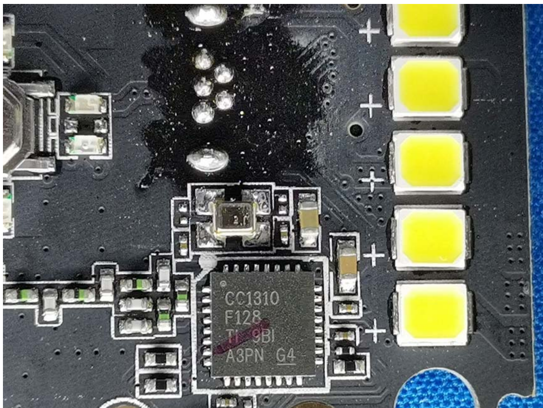
900M Chip
