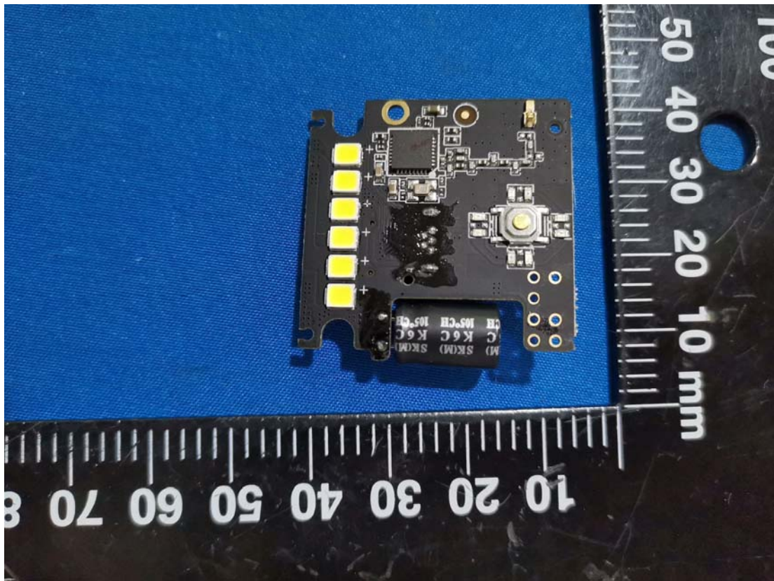
900M Chip
