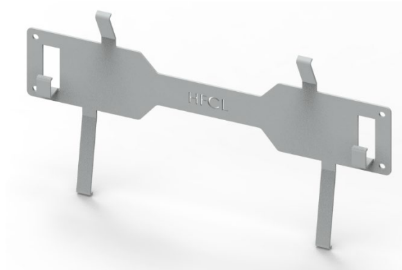
Figure 73: Mounting bracket for indoor AP
