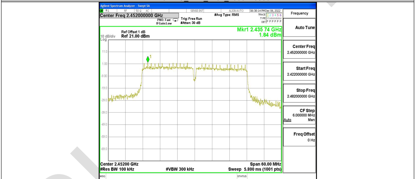
11N40SISO_Ant2_2452_0~Reference
