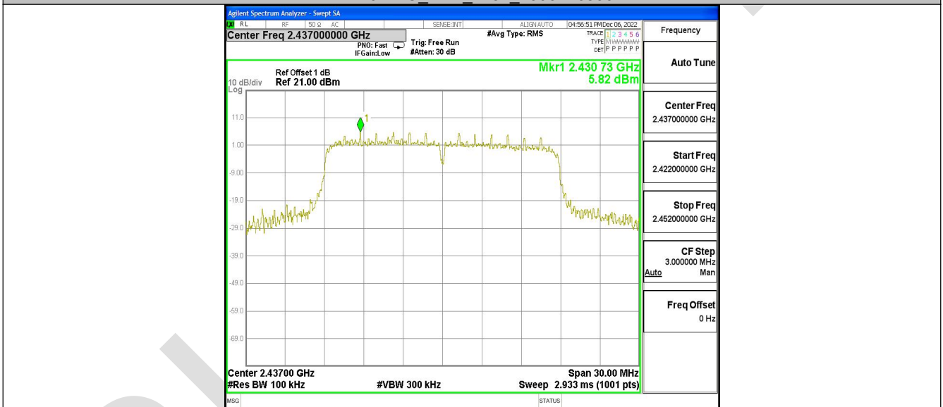
11N20SISO_Ant2_2437_0~Reference
