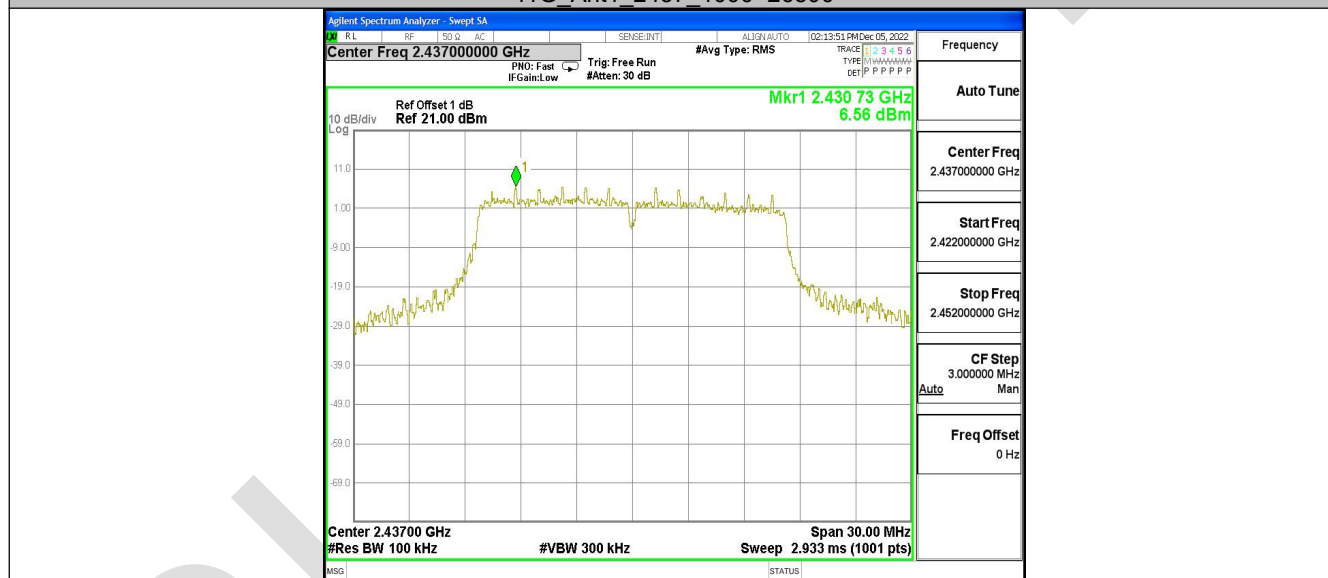
11G_Ant2_2437_0~Reference
