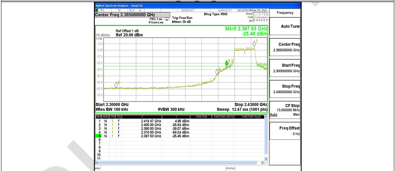
11G_Ant2_Low_2412
