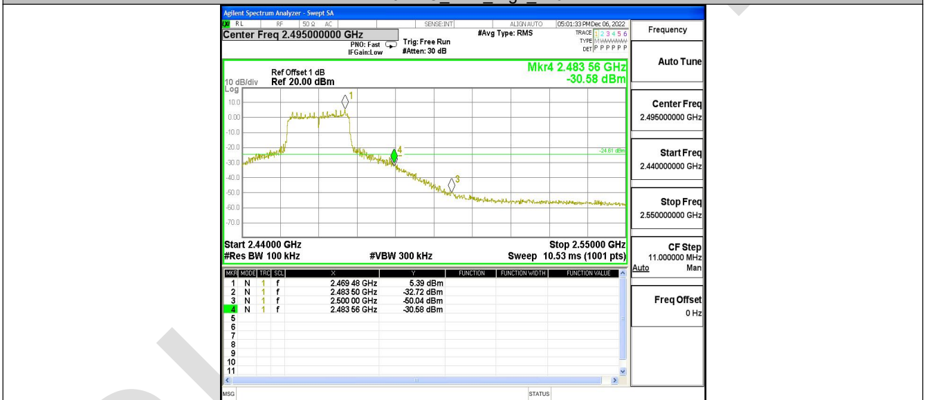
11N20SISO Ant2_High_2462
