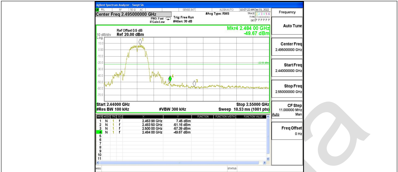
11B_Ant1_High_2462
