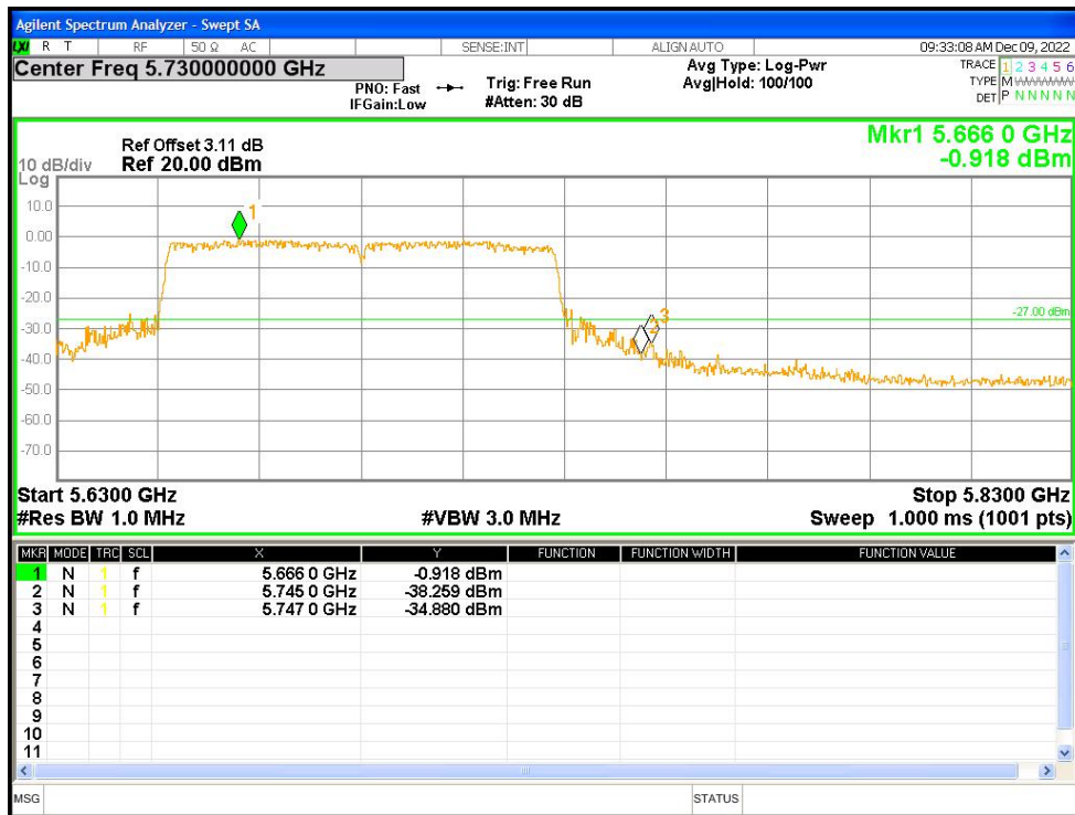
Band Edge NVNT ac80 5690MHz High Ant2
