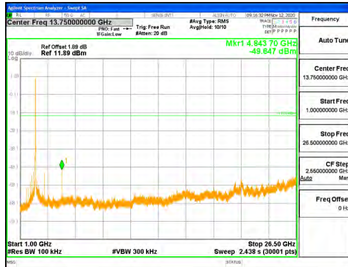
11N40SISO_Ant1_2437_0-Reference
