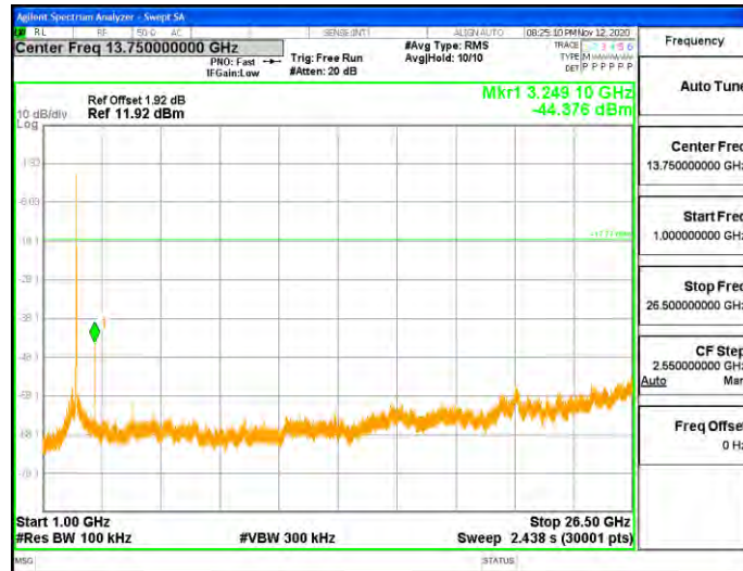
11N20SISO_Ant2_2437_0-Reference
