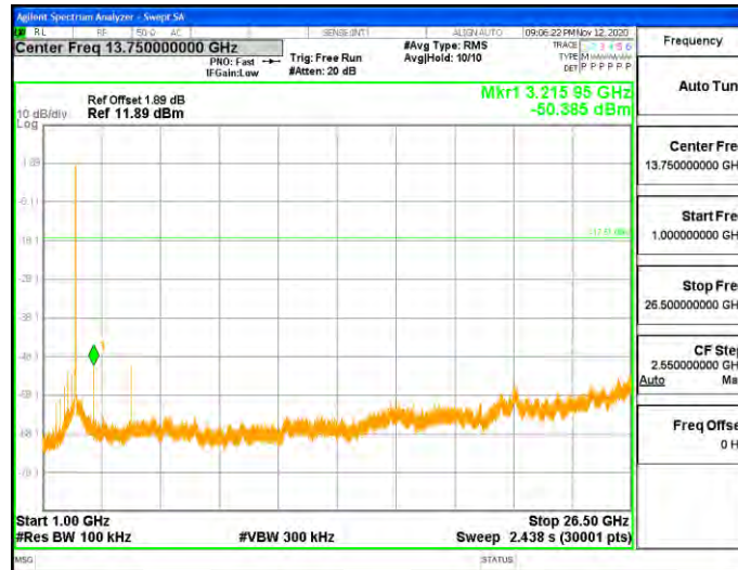
11N20SISO_Ant1_2437_0-Reference
