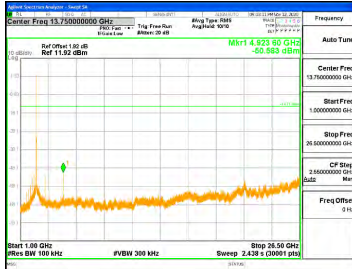
11N20SISO_Ant1_2412_0-Reference
