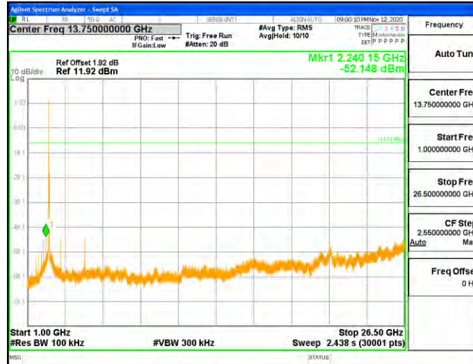
11G_Ant1_2462_0~Reference
