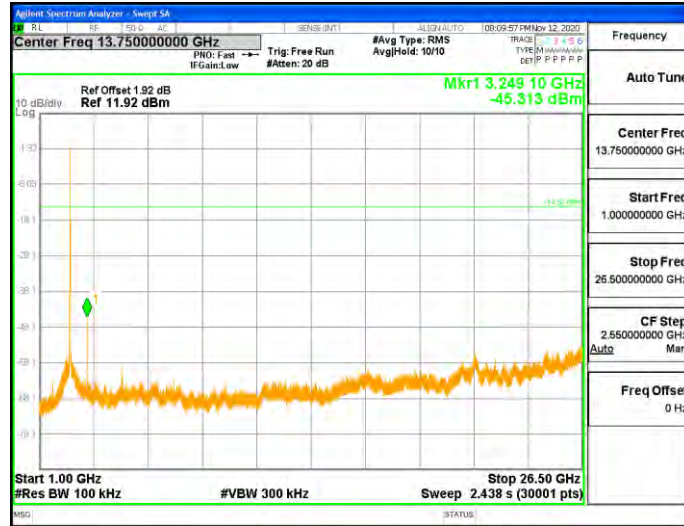
11G_Ant2_2437_0~Reference
