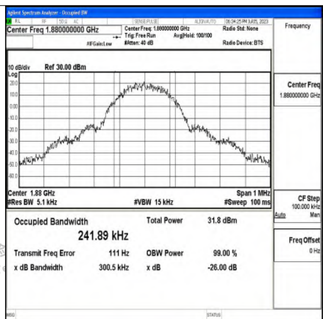
Channel 661 / 1880.0MHz
