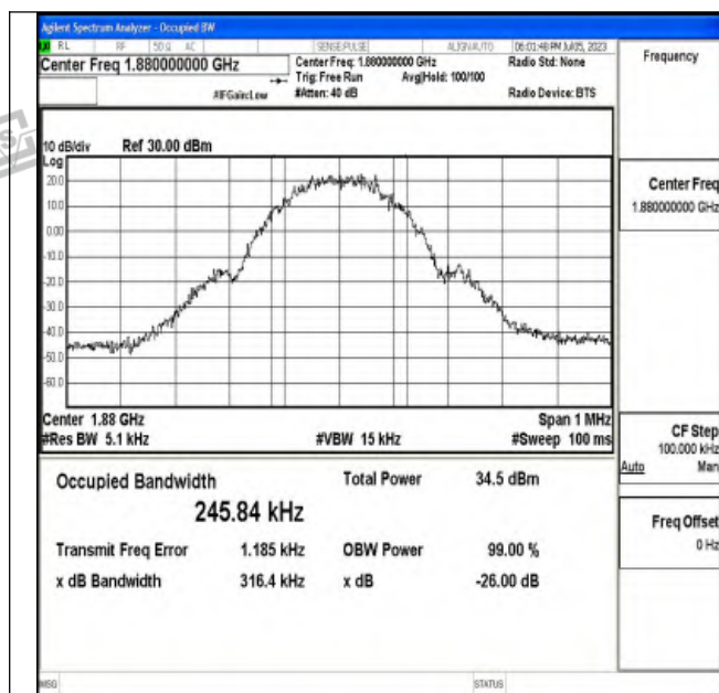
Channel 661 / 1880.0MHz
