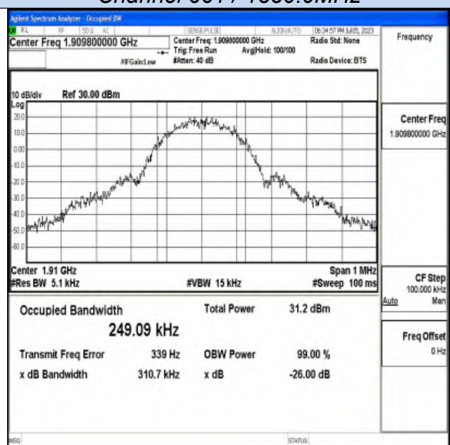
Channel 810 / 1909.8 MHz
