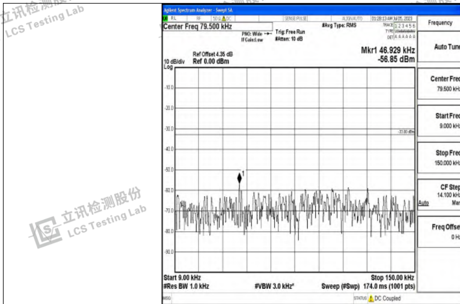
Band12_3MHz_QPSK_23095_1RB#0_0.009~0.15_0.009~0.15
