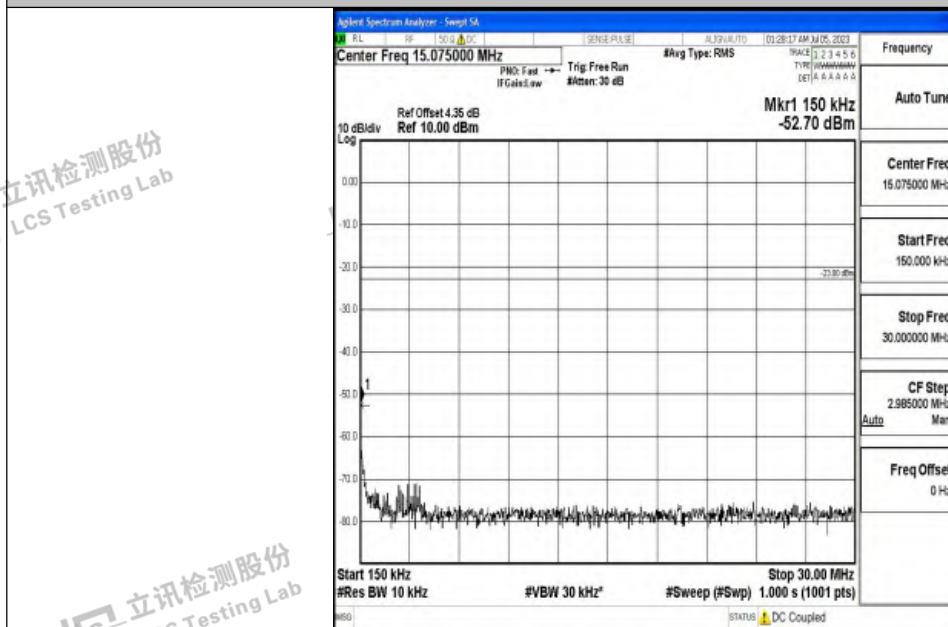
Band12_3MHz_QPSK_23095_1RB#0_0.15~30_0.15~30
