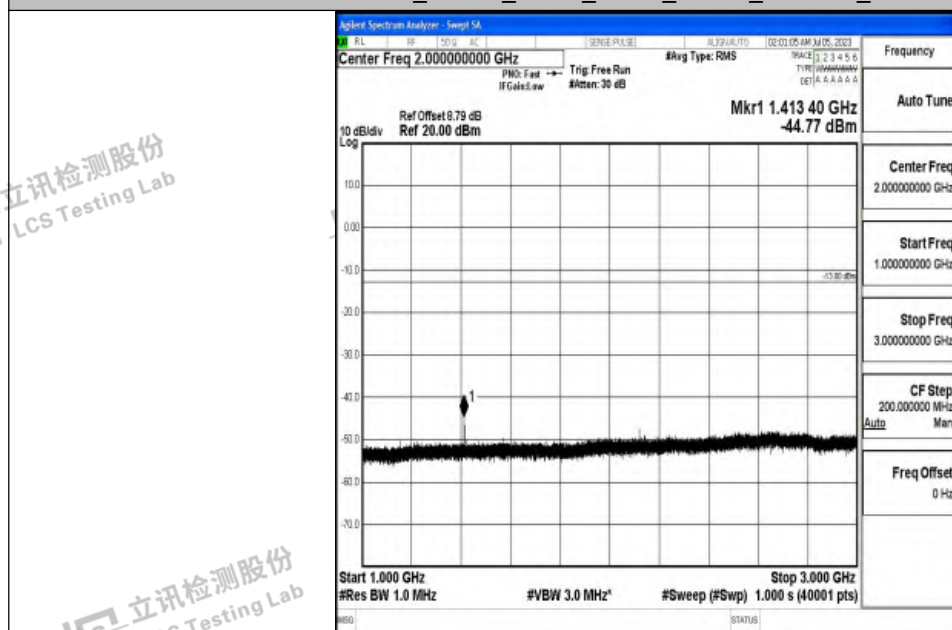
Band12_10MHz_QPSK_23130_1RB#0_1000~3000_1000~3000
