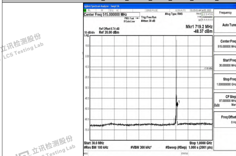
Band12_1.4MHz_16QAM_23173_1RB#0_30~1000_30~1000
