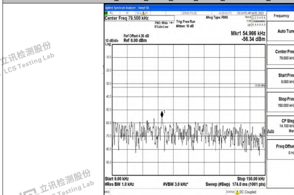
Band12_1.4MHz_16QAM_23173_1RB#0_0.009~0.15_0.009~0.15
