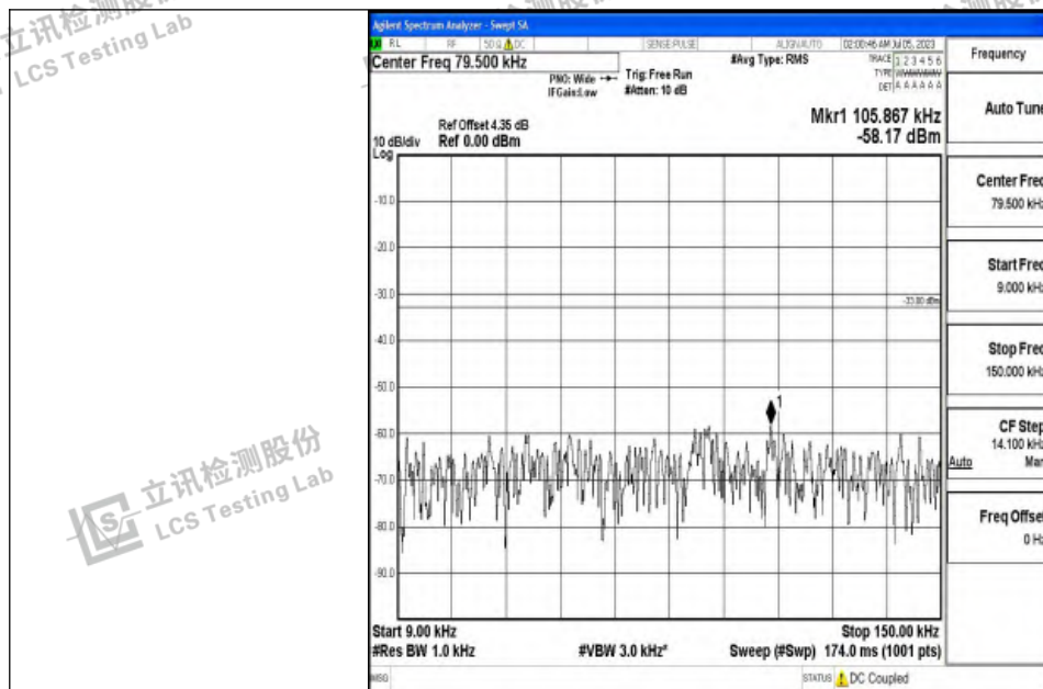
Band12_10MHz_QPSK_23130_1RB#0_0.009~0.15_0.009~0.15
