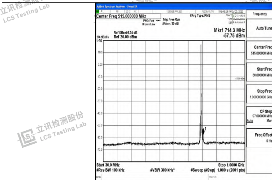
Band12_5MHz_QPSK_23035_1RB#0_30~1000_30~1000
