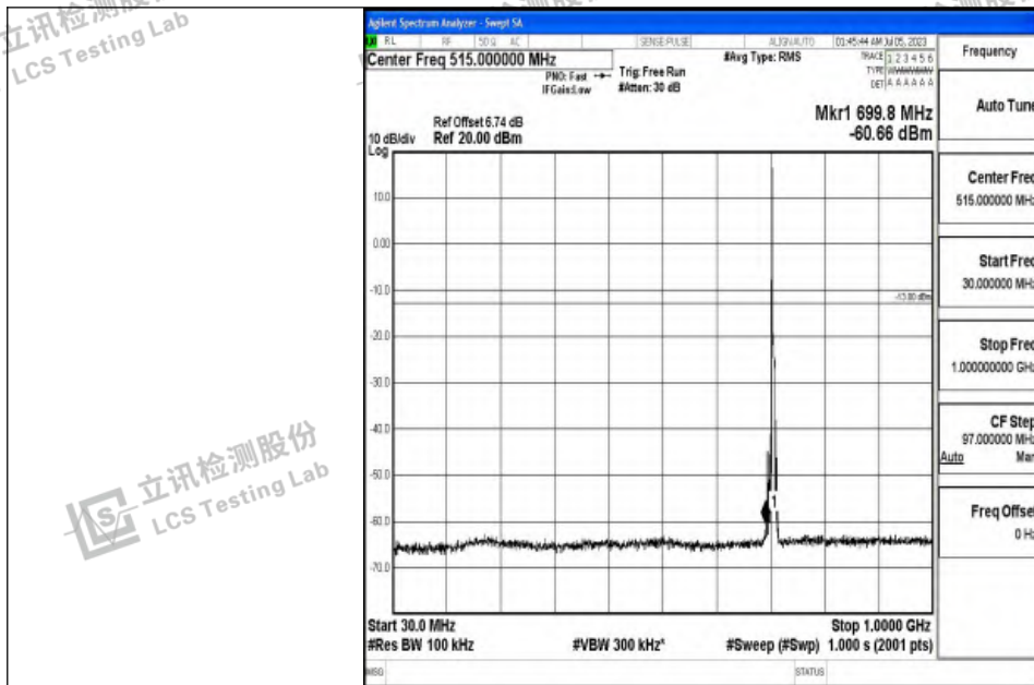
Band12_5MHz_QPSK_23155_1RB#0_30~1000_30~1000
