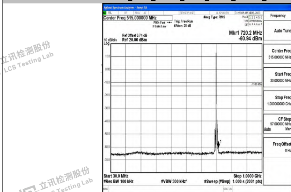
Band12_5MHz_16QAM_23095_1RB#0_30~1000_30~1000
