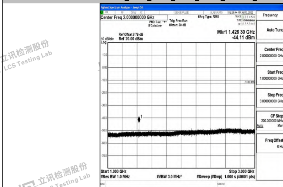
Band12_3MHz_QPSK_23165_1RB#0_1000~3000_1000~3000
