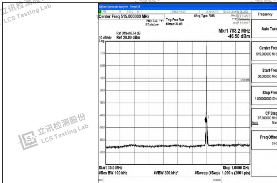
Band12_1.4MHz_QPSK_23095_1RB#0_30~1000_30~1000
