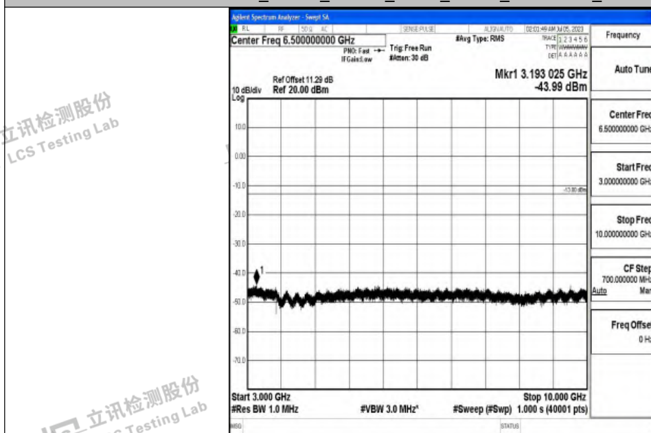
Band12_10MHz_16QAM_23130_1RB#0_3000~10000_3000~10000
