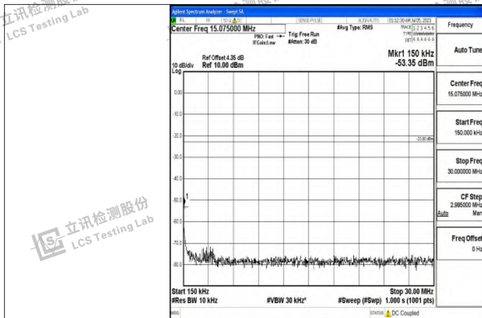
Band12_1.4MHz_16QAM_23017_1RB#0_0.15~30_0.15~30
