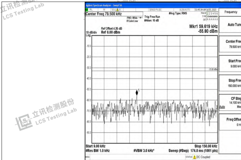
Band12_5MHz_QPSK_23155_1RB#0_0.009~0.15_0.009~0.15
