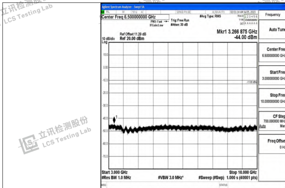
Band12_10MHz_QPSK_23130_1RB#0_3000~10000_3000~10000
