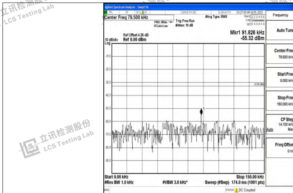
Band12_3MHz_QPSK_23025_1RB#0_0.009~0.15_0.009~0.15
