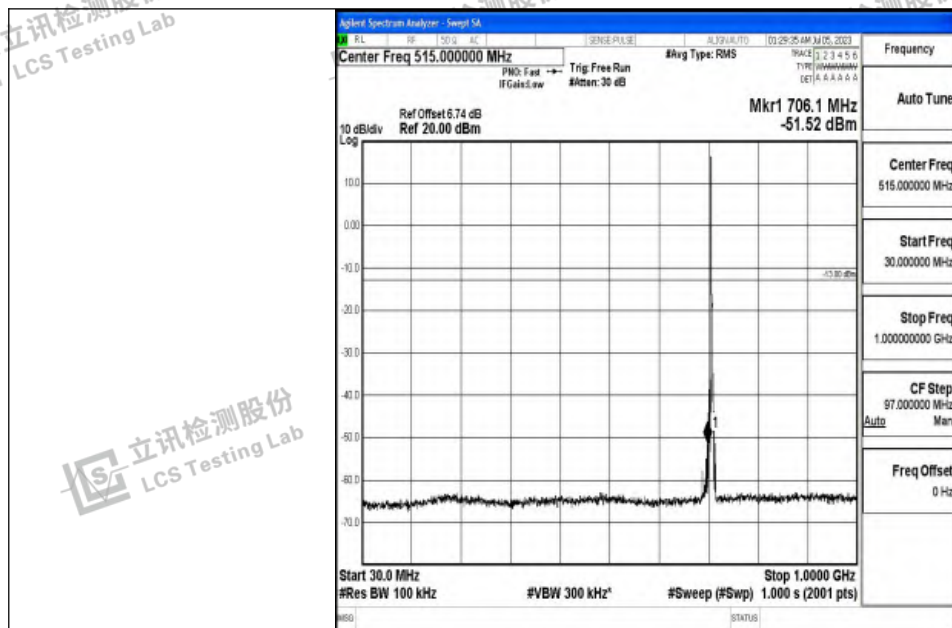
Band12_3MHz_QPSK_23165_1RB#0_30~1000_30~1000
