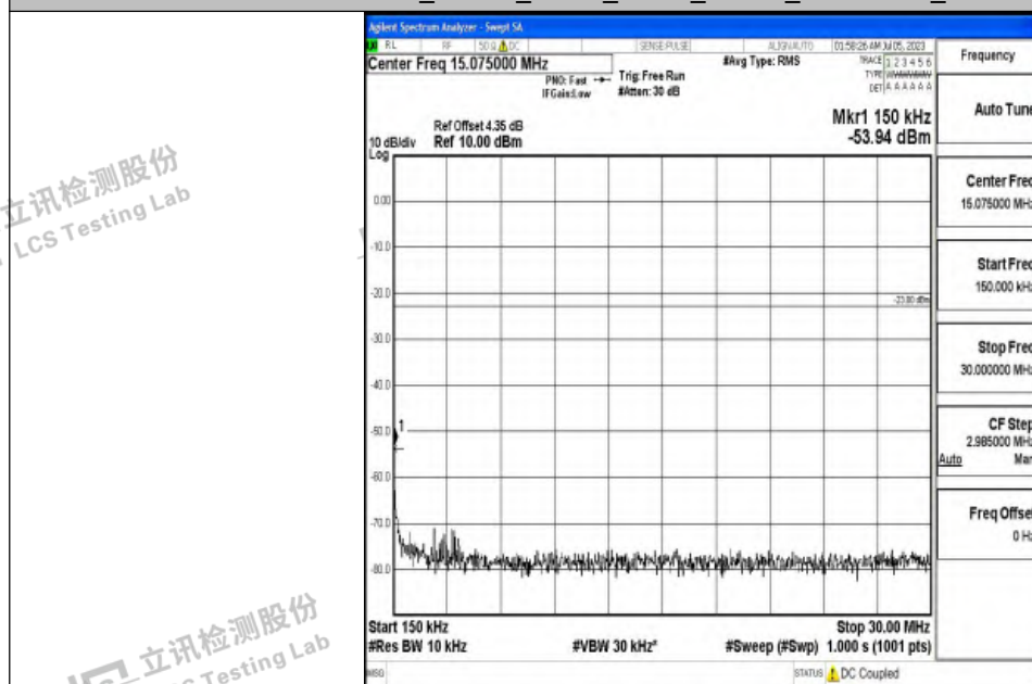
Band12_10MHz_QPSK_23060_1RB#0_0.15~30_0.15~30
