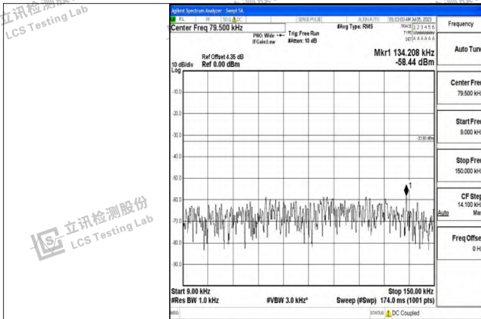
Band12_1.4MHz_QPSK_23095_1RB#0_0.009~0.15_0.009~0.15
