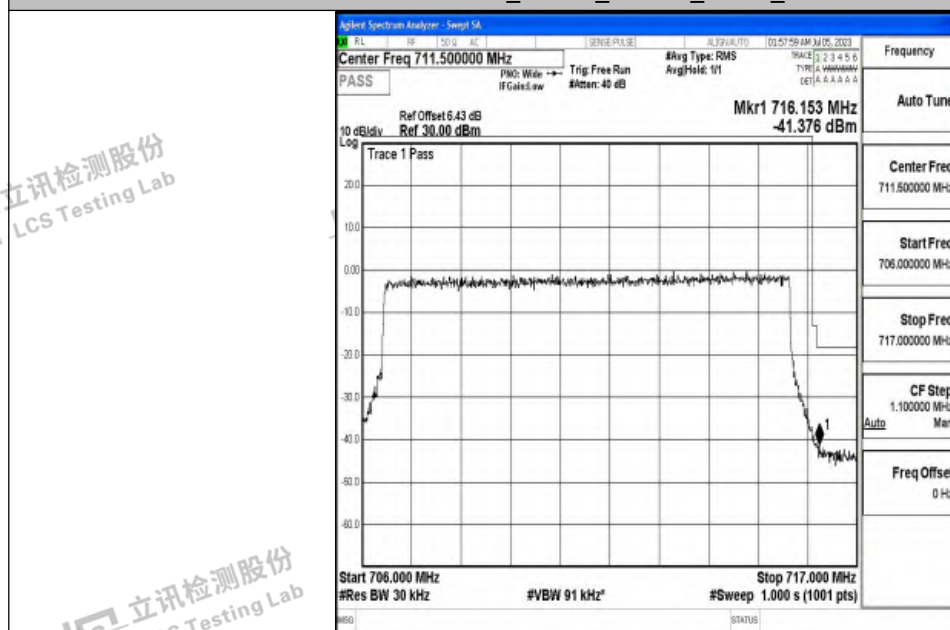
Band12_10MHz_QPSK_23130_50RB#0
