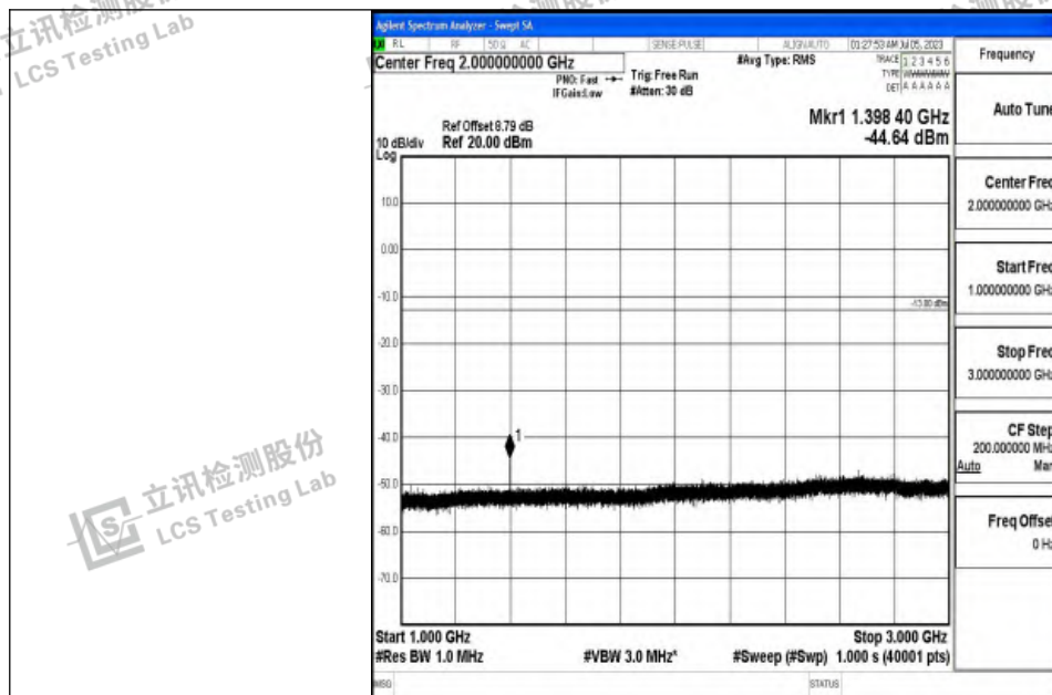
Band12_3MHz_16QAM_23025_1RB#0_1000~3000_1000~3000
