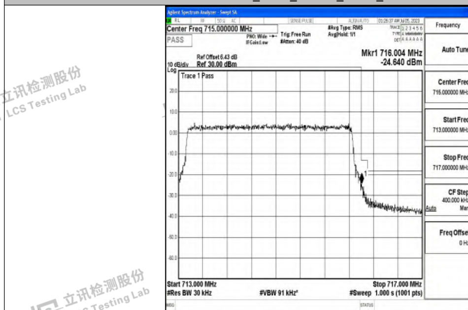
Band12_3MHz_QPSK_23165_15RB#0
