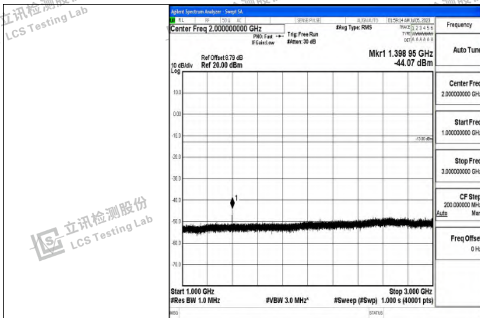
Band12_10MHz_16QAM_23060_1RB#0_1000~3000_1000~3000
