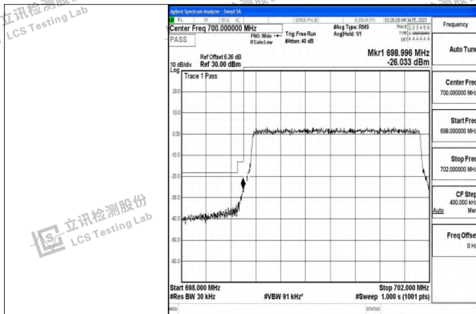
Band12_3MHz_16QAM_23025_15RB#0
