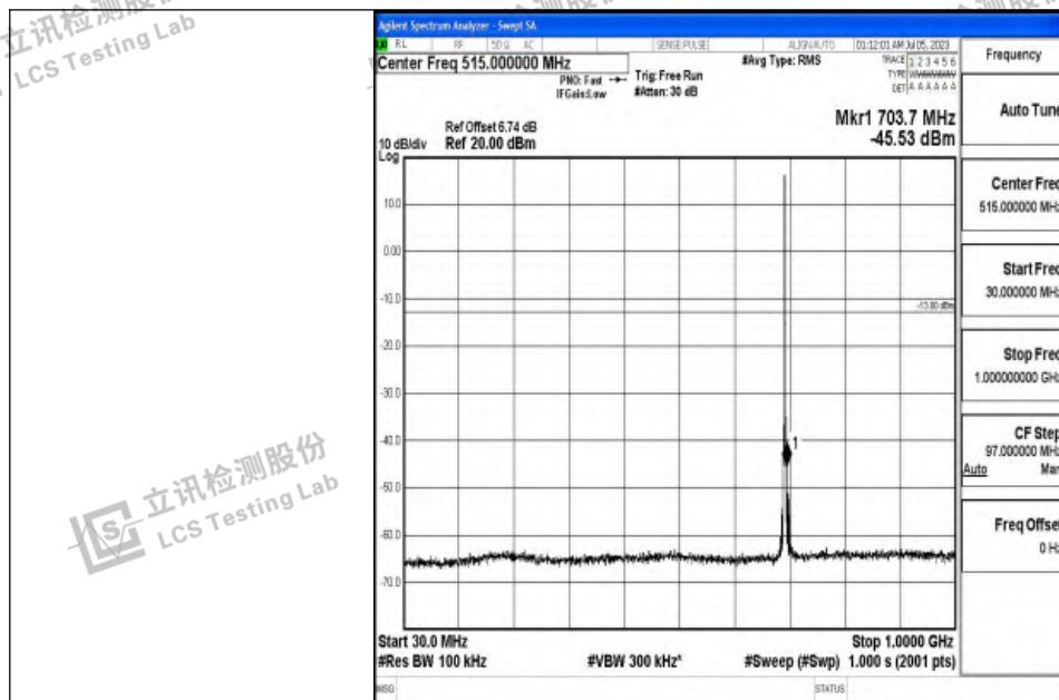
Band12_1.4MHz_QPSK_23017_1RB#0_30~1000_30~1000
