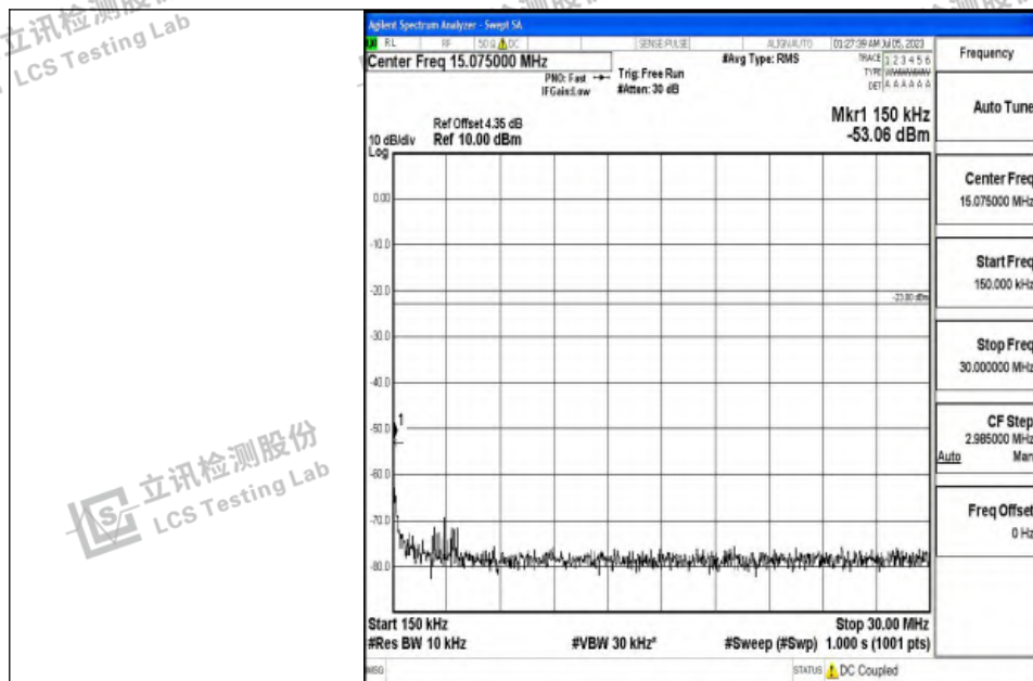
Band12_3MHz_16QAM_23025_1RB#0_0.15~30_0.15~30
