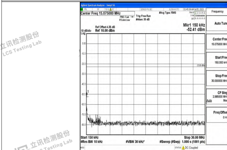
Band12_5MHz_QPSK_23155_1RB#0_0.15~30_0.15~30
