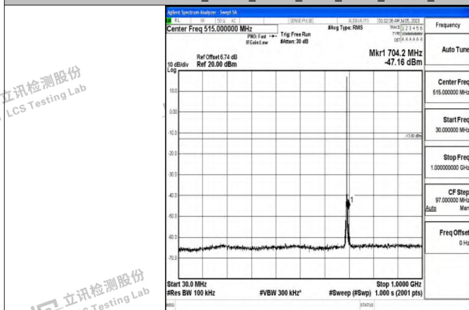
Band12_1.4MHz_16QAM_23017_1RB#0_30~1000_30~1000
