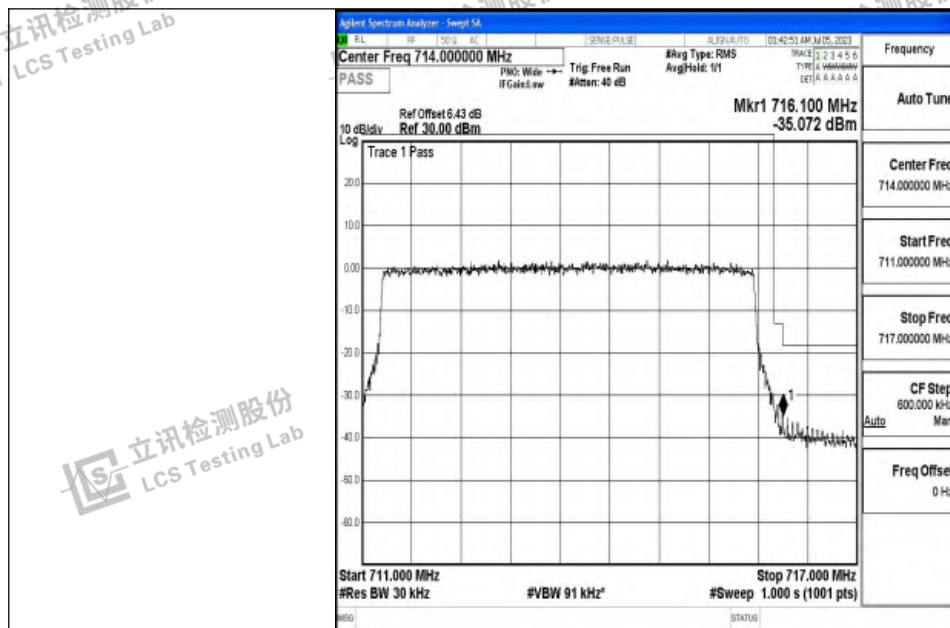
Band12_5MHz_16QAM_23155_25RB#0
