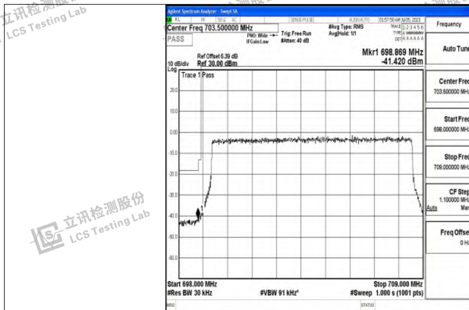
Band12_10MHz_16QAM_23060_50RB#0
