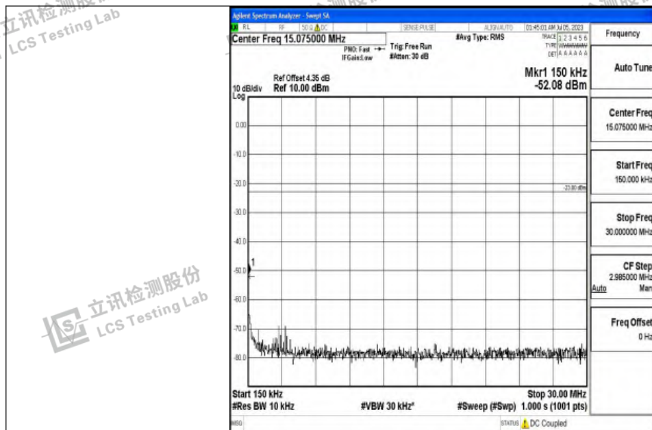
Band12_5MHz_16QAM_23095_1RB#0_0.15~30_0.15~30
