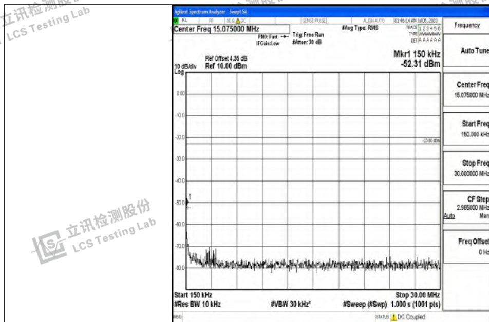
Band12_5MHz_16QAM_23155_1RB#0_0.15~30_0.15~30
