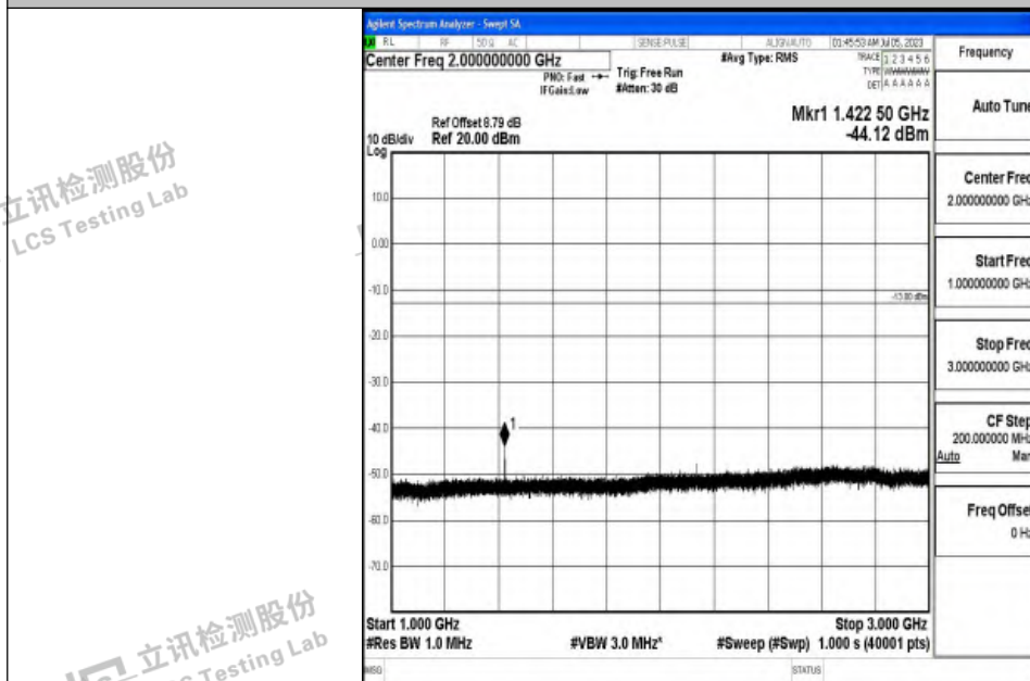
Band12_5MHz_QPSK_23155_1RB#0_1000~3000_1000~3000
