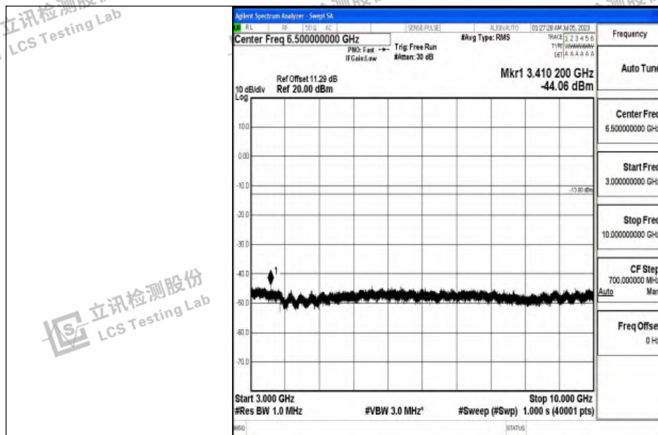
Band12_3MHz_QPSK_23025_1RB#0_3000~10000_3000~10000
