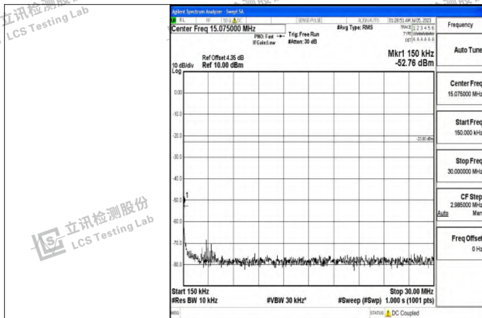
Band12_3MHz_16QAM_23095_1RB#0_0.15~30_0.15~30
