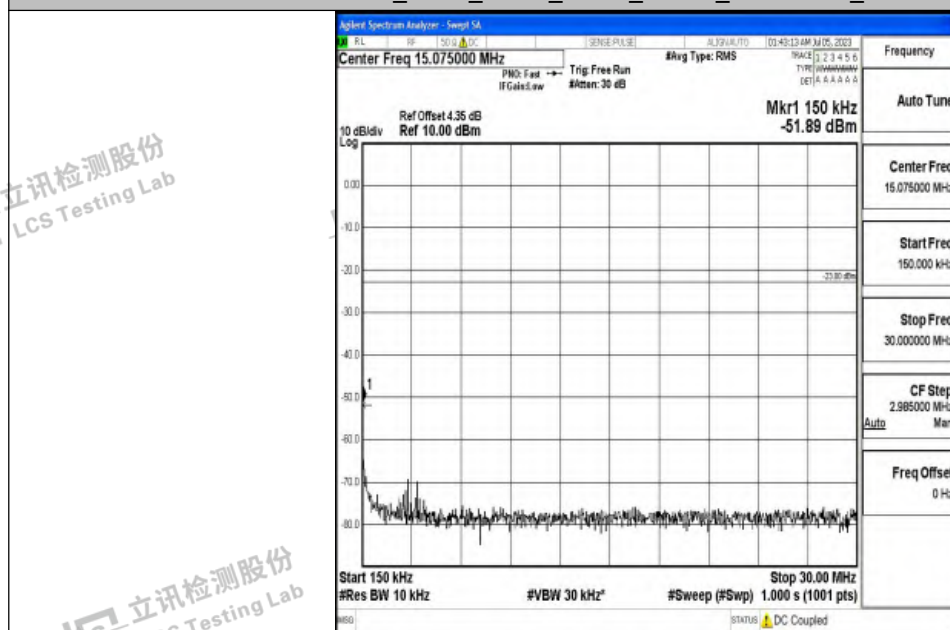
Band12_5MHz_QPSK_23035_1RB#0_0.15~30_0.15~30
