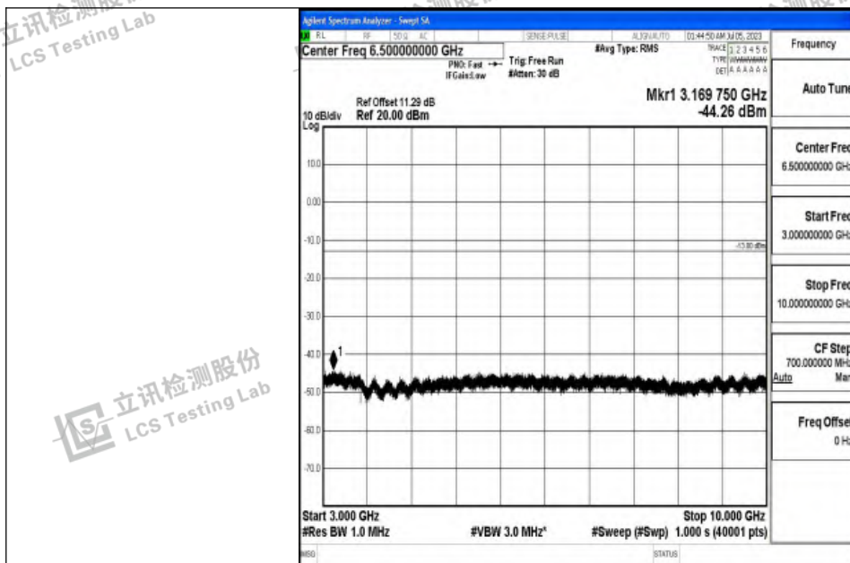
Band12_5MHz_QPSK_23095_1RB#0_3000~10000_3000~10000
