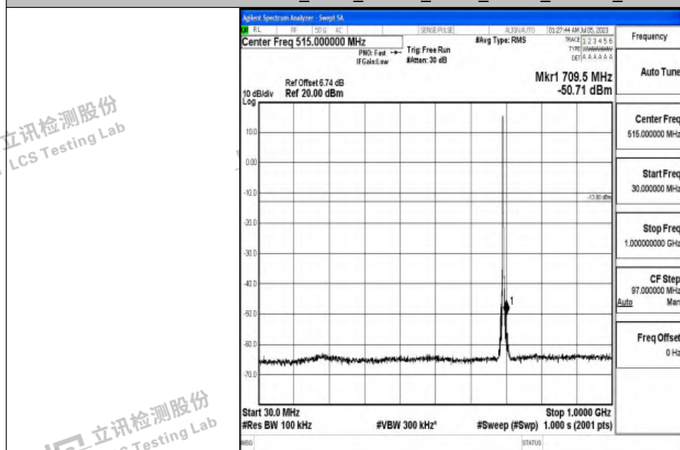
Band12_3MHz_16QAM_23025_1RB#0_30~1000_30~1000
