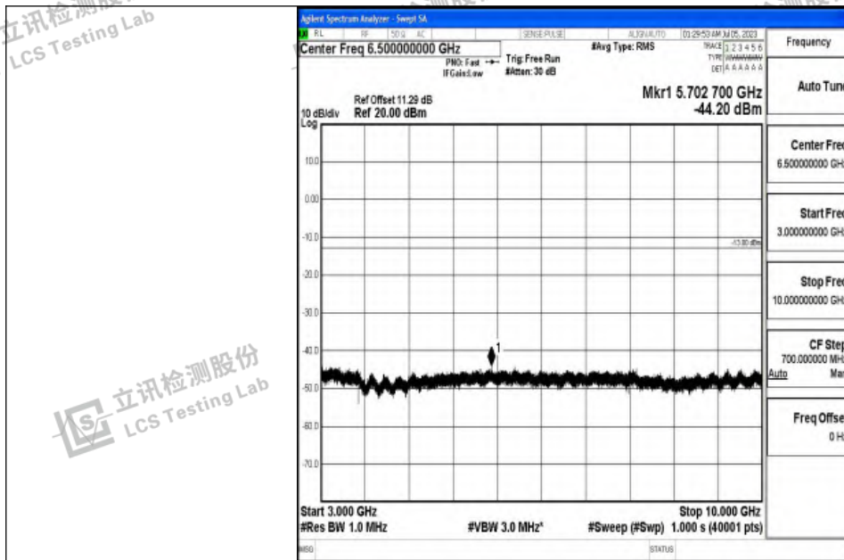
Band12_3MHz_QPSK_23165_1RB#0_3000~10000_3000~10000
