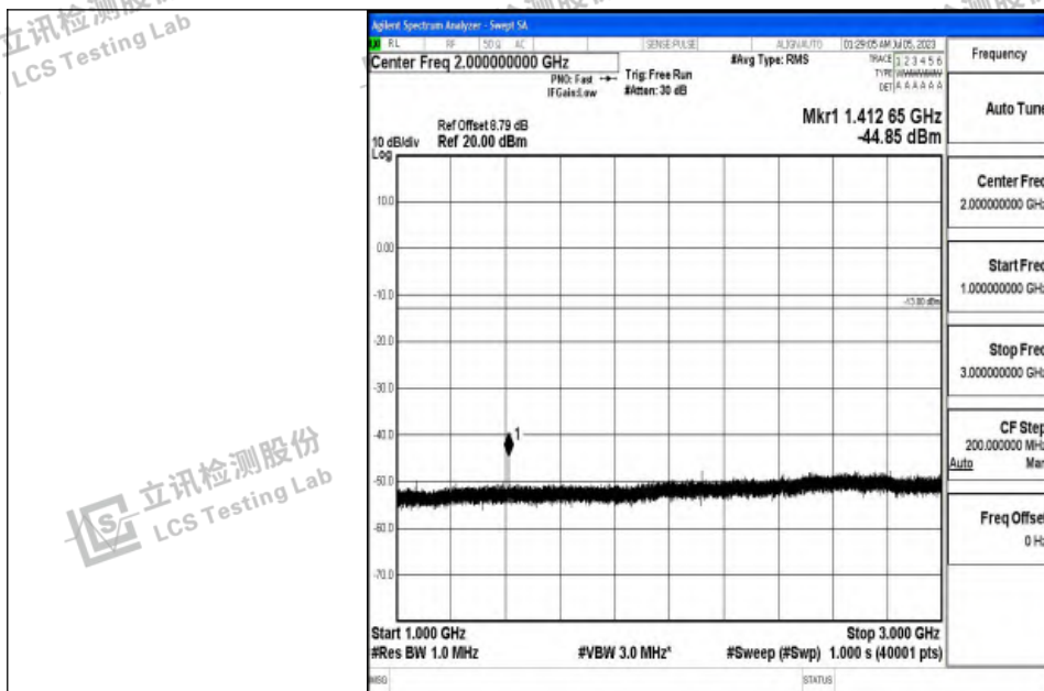
Band12_3MHz_16QAM_23095_1RB#0_1000~3000_1000~3000
