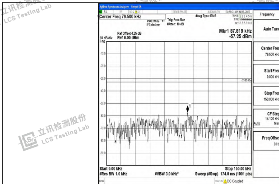
Band12_10MHz_QPSK_23060_1RB#0_0.009~0.15_0.009~0.15
