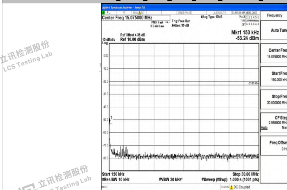
Band12_10MHz_QPSK_23095_1RB#0_0.15~30_0.15~30
