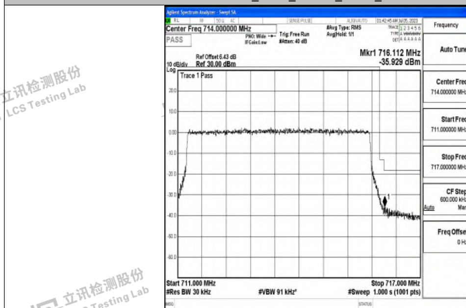
Band12_5MHz_QPSK_23155_25RB#0
