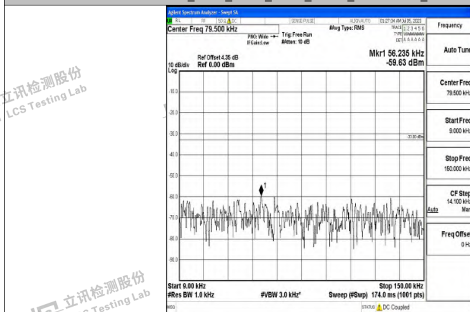
Band12_3MHz_16QAM_23025_1RB#0_0.009~0.15_0.009~0.15
