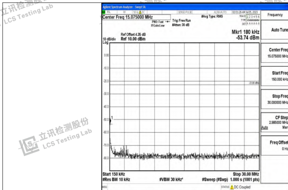
Band12_10MHz_16QAM_23130_1RB#0_0.15~30_0.15~30
