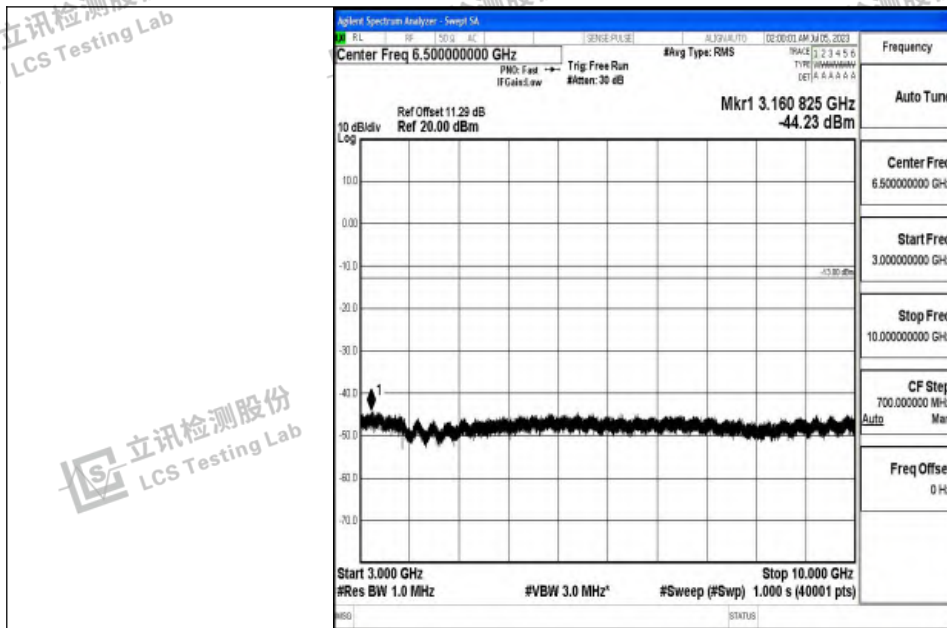
Band12_10MHz_QPSK_23095_1RB#0_3000~10000_3000~10000
