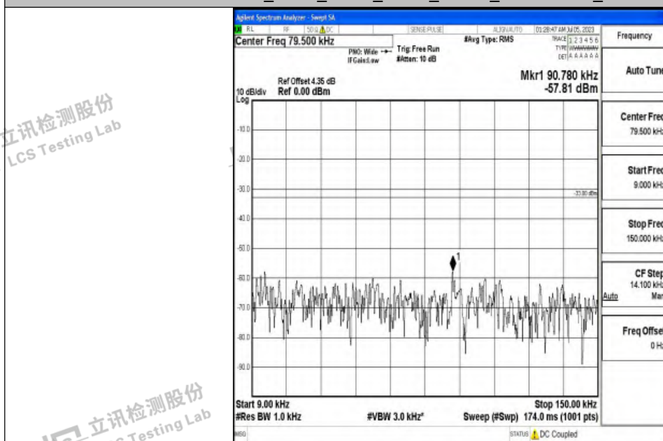
Band12_3MHz_16QAM_23095_1RB#0_0.009~0.15_0.009~0.15
