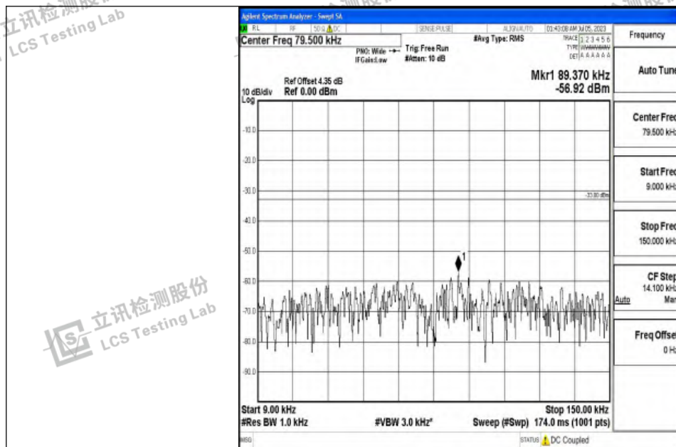
Band12_5MHz_QPSK_23035_1RB#0_0.009~0.15_0.009~0.15
