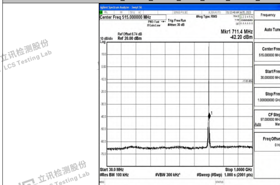
Band12_1.4MHz_16QAM_23095_1RB#0_30~1000_30~1000
