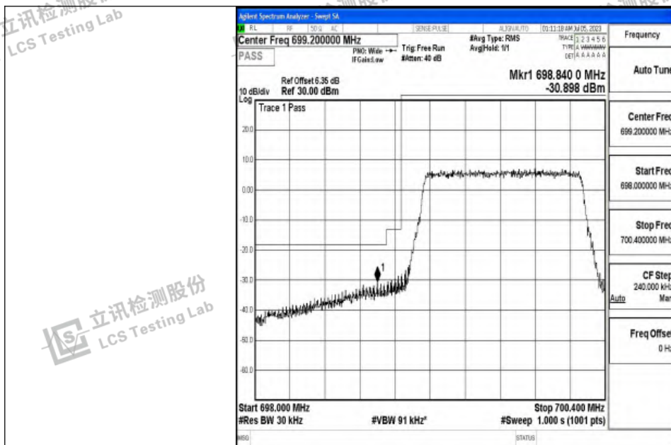
Band12_1.4MHz_16QAM_23017_6RB#0
