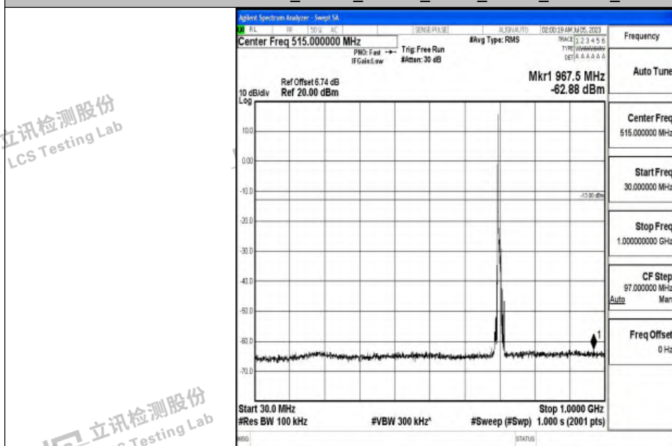
Band12_10MHz_16QAM_23095_1RB#0_30~1000_30~1000
