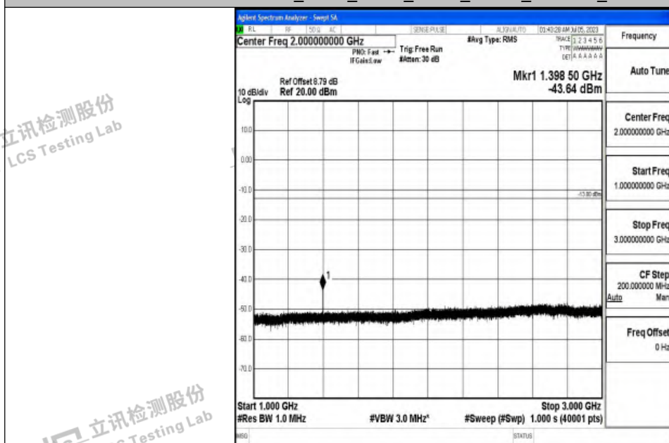
Band12_5MHz_QPSK_23035_1RB#0_1000~3000_1000~3000
