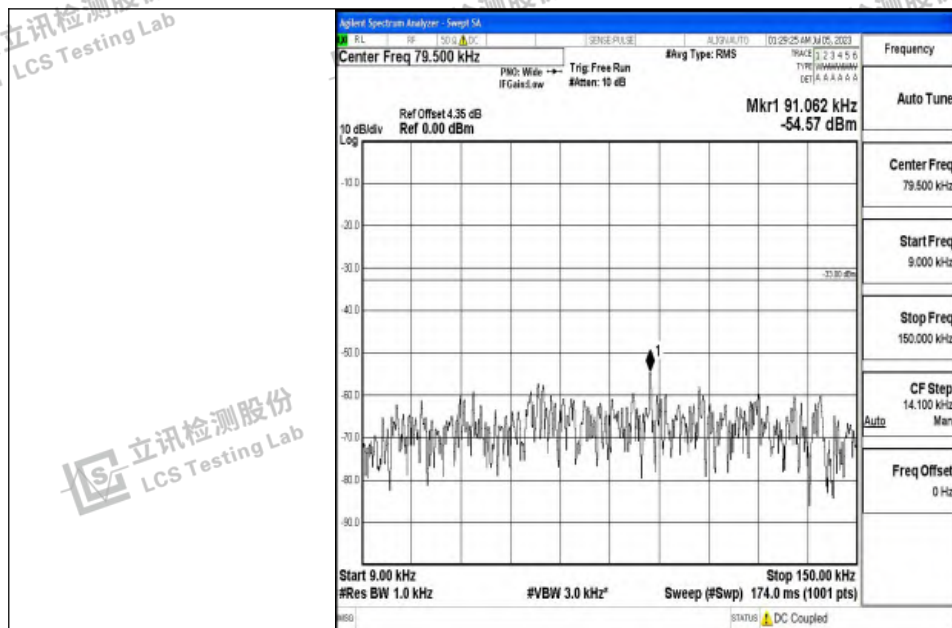
Band12_3MHz_QPSK_23165_1RB#0_0.009~0.15_0.009~0.15
