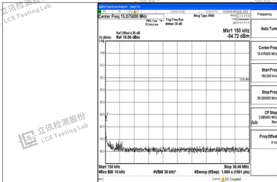
Band12_10MHz_16QAM_23060_1RB#0_0.15~30_0.15~30
