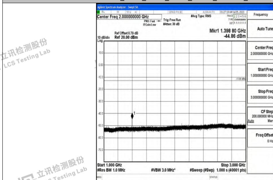
Band12_3MHz_QPSK_23025_1RB#0_1000~3000_1000~3000
