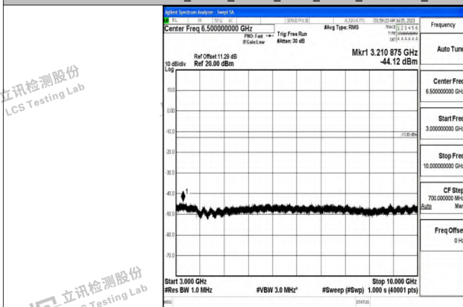
Band12_10MHz_16QAM_23060_1RB#0_3000~10000_3000~10000
