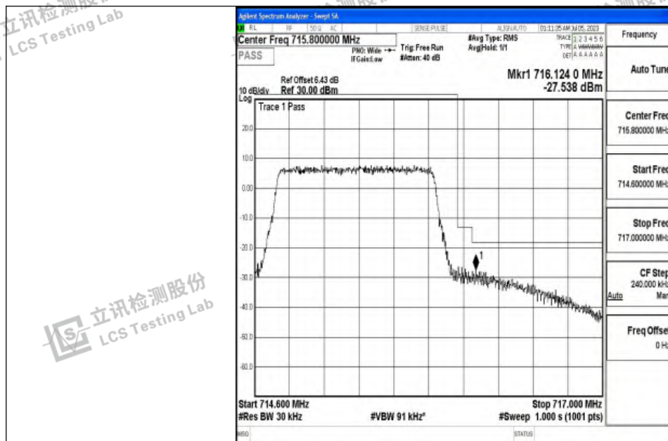
Band12_1.4MHz_16QAM_23173_6RB#0
