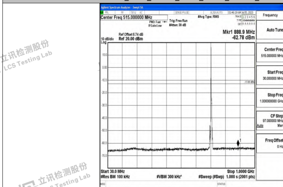
Band12_5MHz_16QAM_23155_1RB#0_30~1000_30~1000
