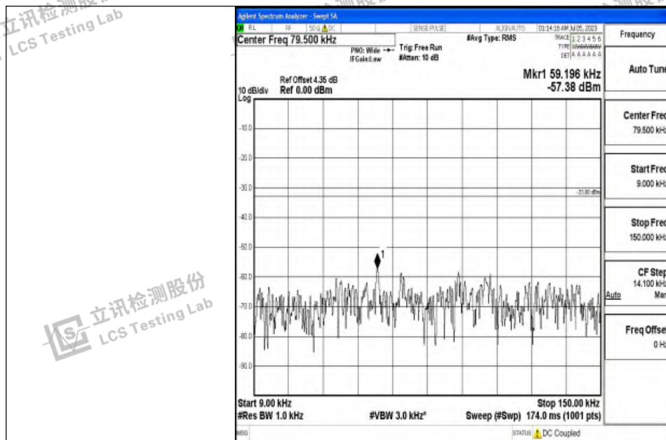
Band12_1.4MHz_QPSK_23173_1RB#0_0.009~0.15_0.009~0.15
