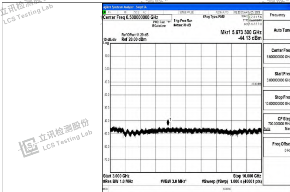
Band12_1.4MHz_QPSK_23095_1RB#0_3000~10000_3000~10000
