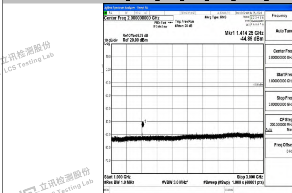
Band12_1.4MHz_QPSK_23095_1RB#0_1000~3000_1000~3000
