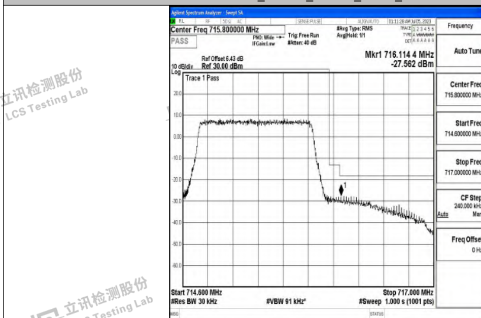
Band12_1.4MHz_QPSK_23173_6RB#0
