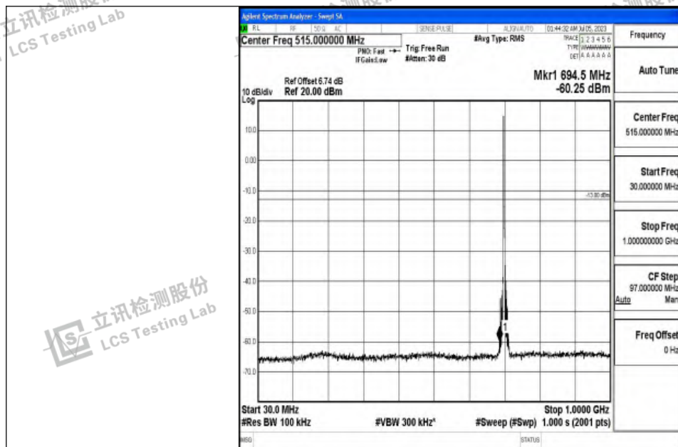
Band12_5MHz_QPSK_23095_1RB#0_30~1000_30~1000
