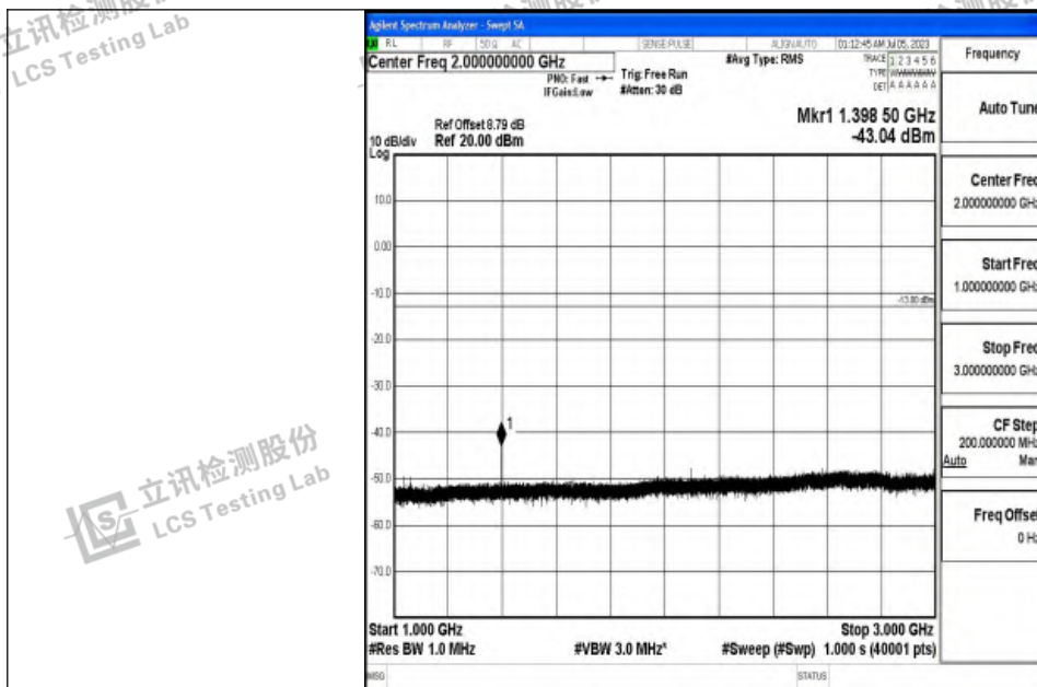
Band12_1.4MHz_16QAM_23017_1RB#0_1000~3000_1000~3000
