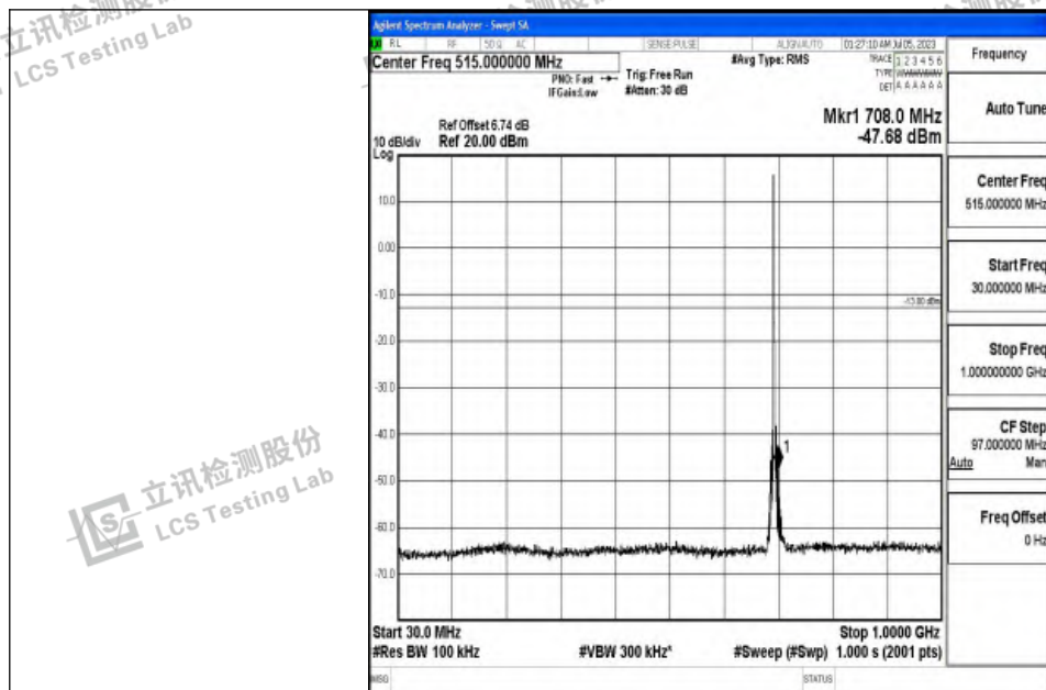
Band12_3MHz_QPSK_23025_1RB#0_30~1000_30~1000
