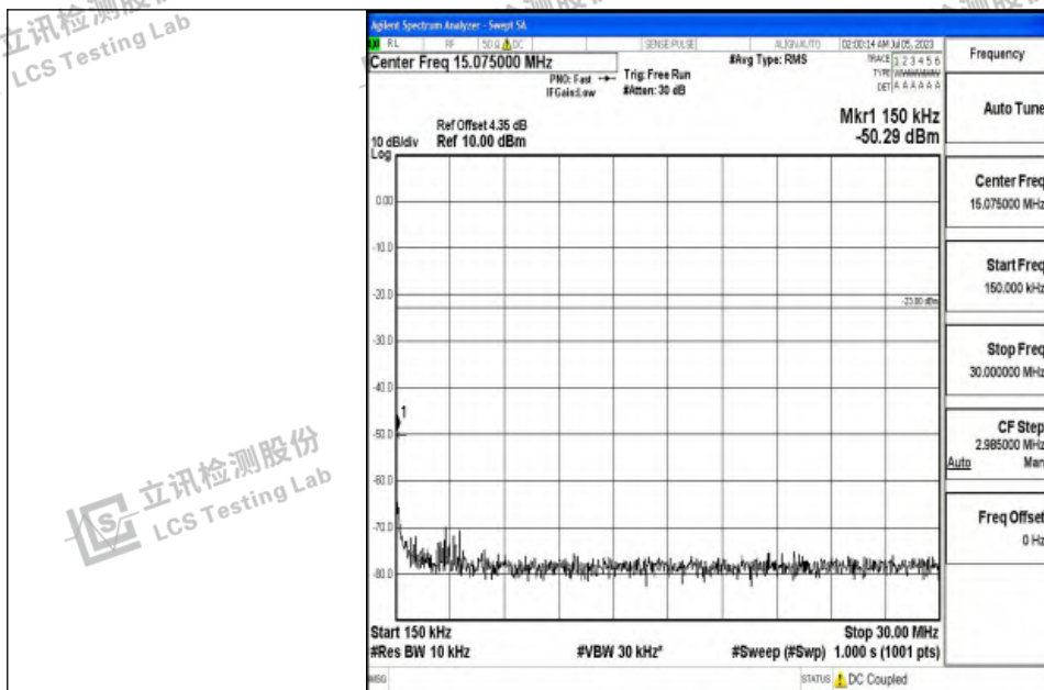
Band12_10MHz_16QAM_23095_1RB#0_0.15~30_0.15~30
