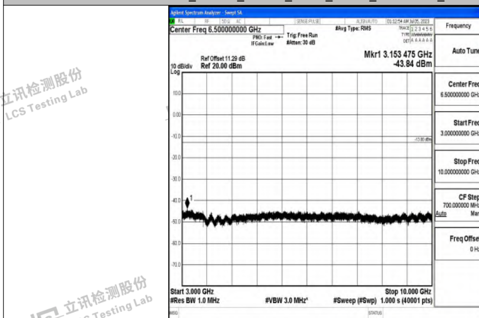
Band12_1.4MHz_16QAM_23017_1RB#0_3000~10000_3000~10000
