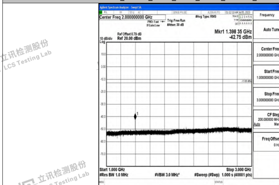
Band12_1.4MHz_QPSK_23017_1RB#0_1000~3000_1000~3000
