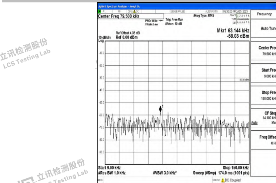
Band12_3MHz_16QAM_23165_1RB#0_0.009~0.15_0.009~0.15
