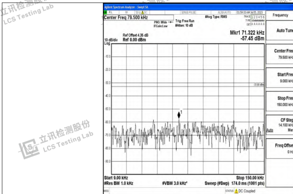
Band12_10MHz_QPSK_23095_1RB#0_0.009~0.15_0.009~0.15
