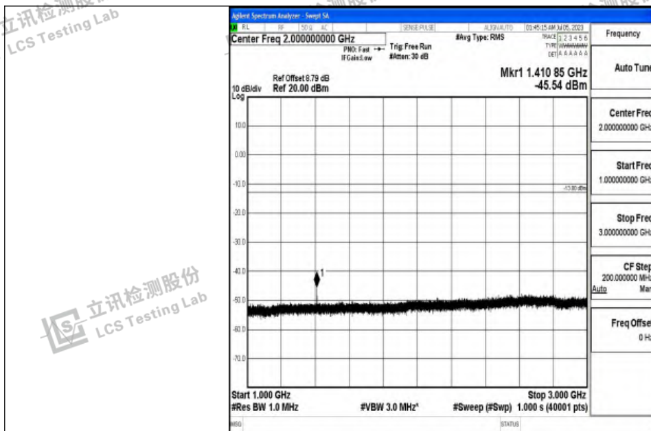
Band12_5MHz_16QAM_23095_1RB#0_1000~3000_1000~3000
