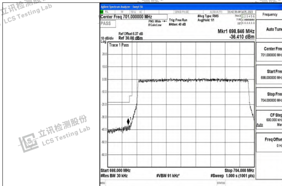
Band12_5MHz_16QAM_23035_25RB#0
