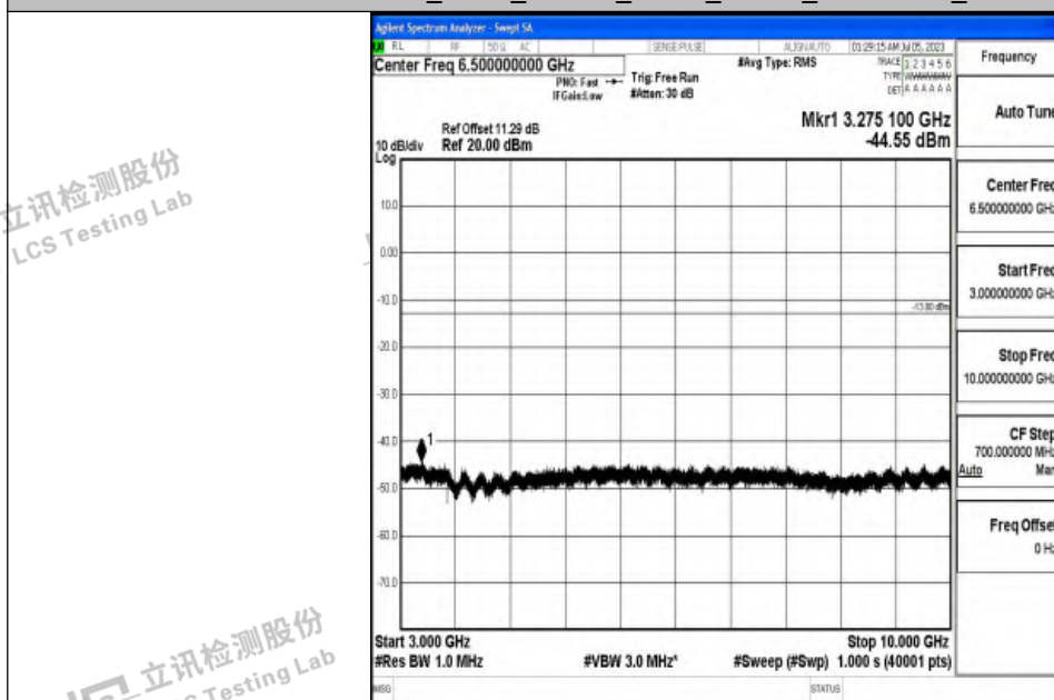
Band12_3MHz_16QAM_23095_1RB#0_3000~10000_3000~10000
