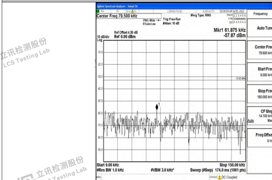
Band12_10MHz_16QAM_23095_1RB#0_0.009~0.15_0.009~0.15
