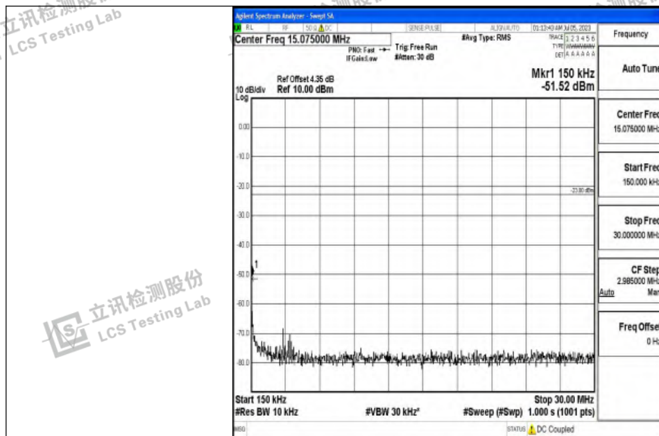
Band12_1.4MHz_16QAM_23095_1RB#0_0.15~30_0.15~30
