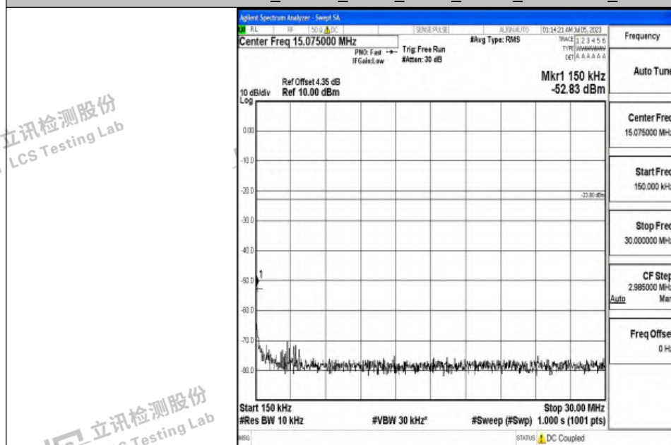
Band12_1.4MHz_QPSK_23173_1RB#0_0.15~30_0.15~30
