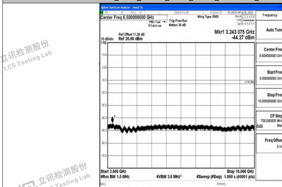
Band12_3MHz_16QAM_23025_1RB#0_3000~10000_3000~10000
