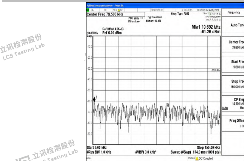
Band12_5MHz_16QAM_23035_1RB#0_0.009~0.15_0.009~0.15
