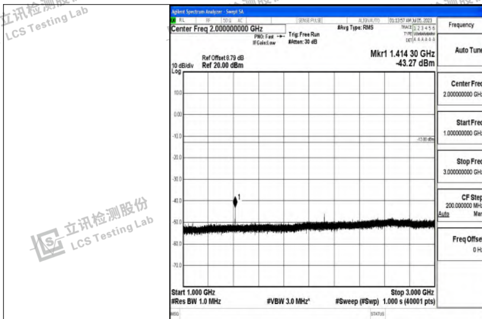
Band12_1.4MHz_16QAM_23095_1RB#0_1000~3000_1000~3000
