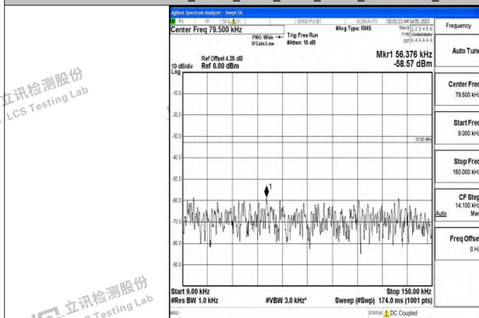
Band12_10MHz_16QAM_23130_1RB#0_0.009~0.15_0.009~0.15
