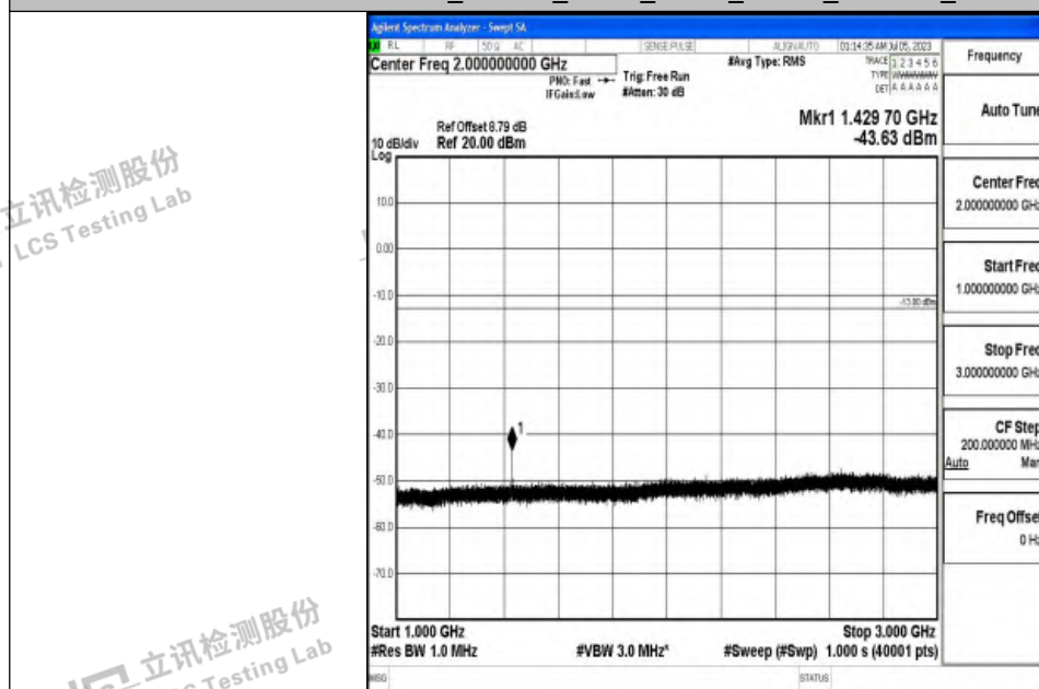
Band12_1.4MHz_QPSK_23173_1RB#0_1000~3000_1000~3000
