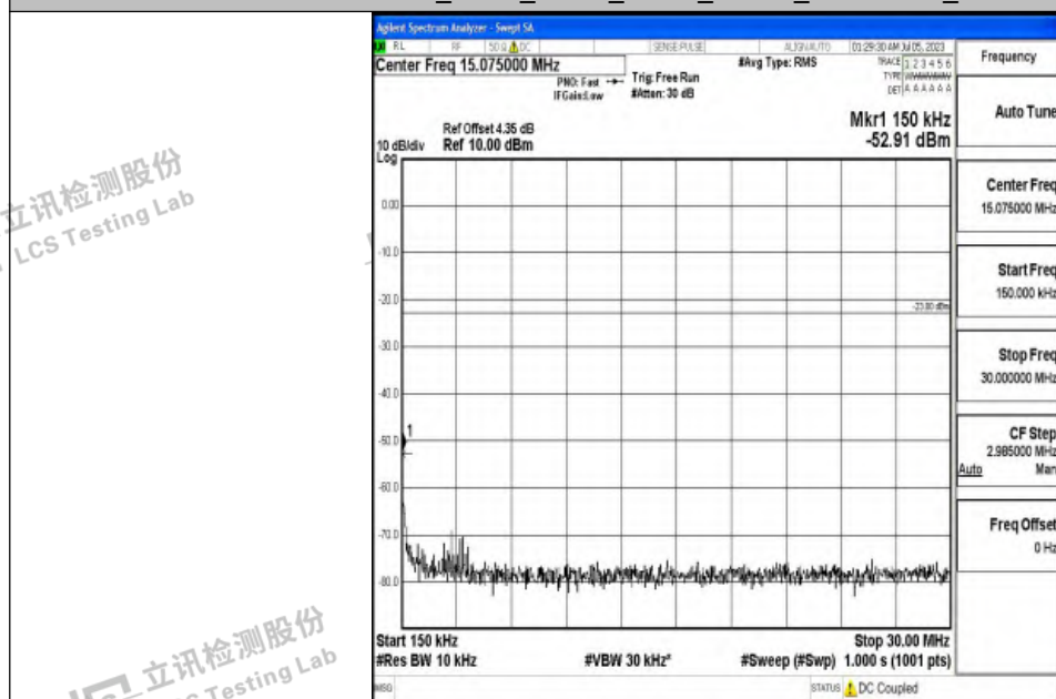
Band12_3MHz_QPSK_23165_1RB#0_0.15~30_0.15~30
