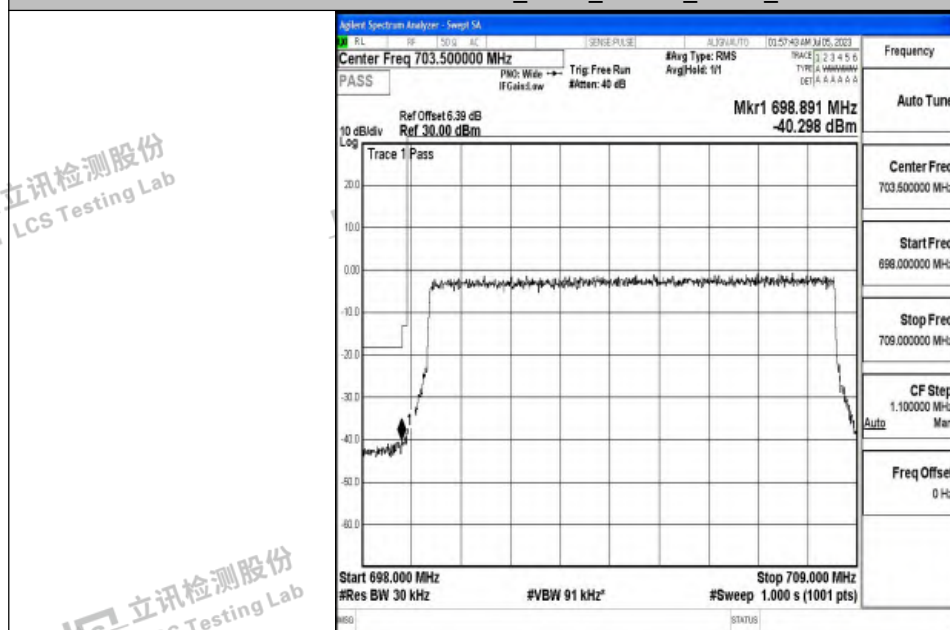
Band12_10MHz_QPSK_23060_50RB#0
