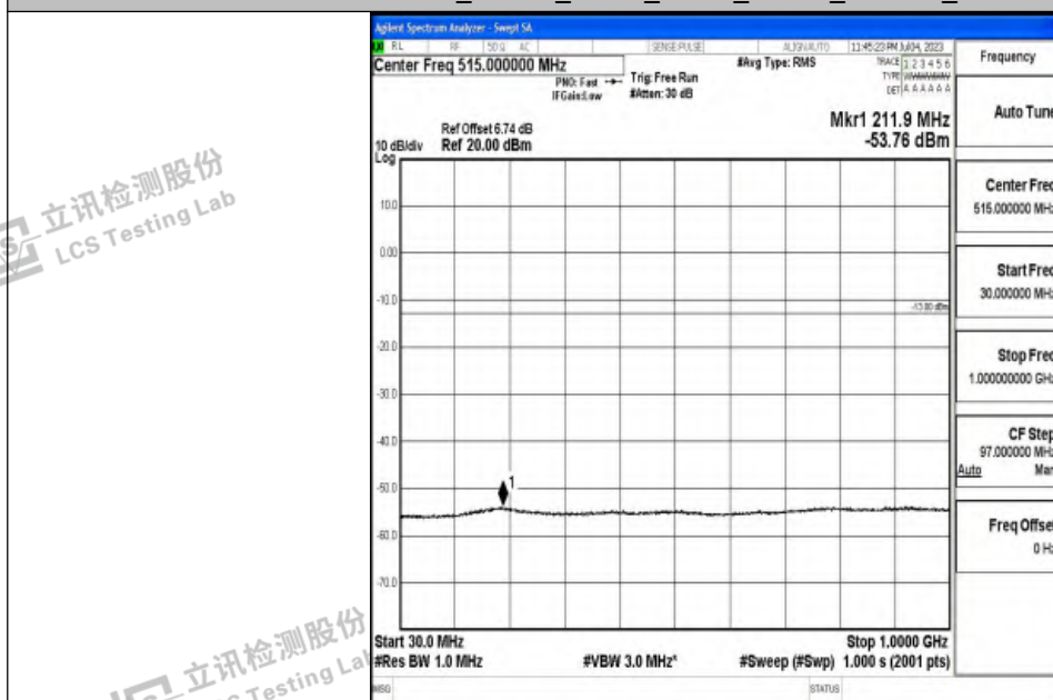
Band4_15MHz_QPSK_20025_1RB#0_30~1000_30~1000
