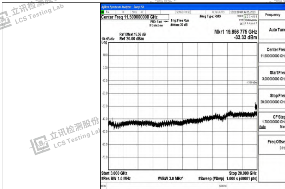
Band4_20MHz_16QAM_20175_1RB#0_3000~20000_3000~20000
