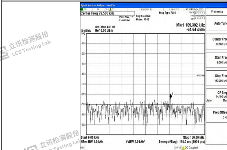
Band4_15MHz_QPSK_20325_1RB#0_0.009~0.15_0.009~0.15
