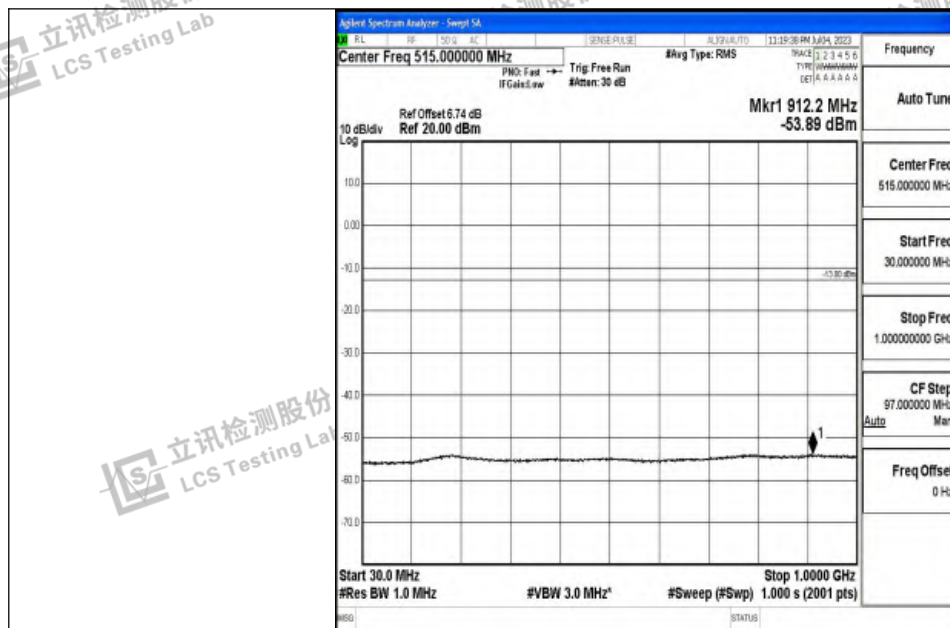
Band4_5MHz_16QAM_20175_1RB#0_30~1000_30~1000
