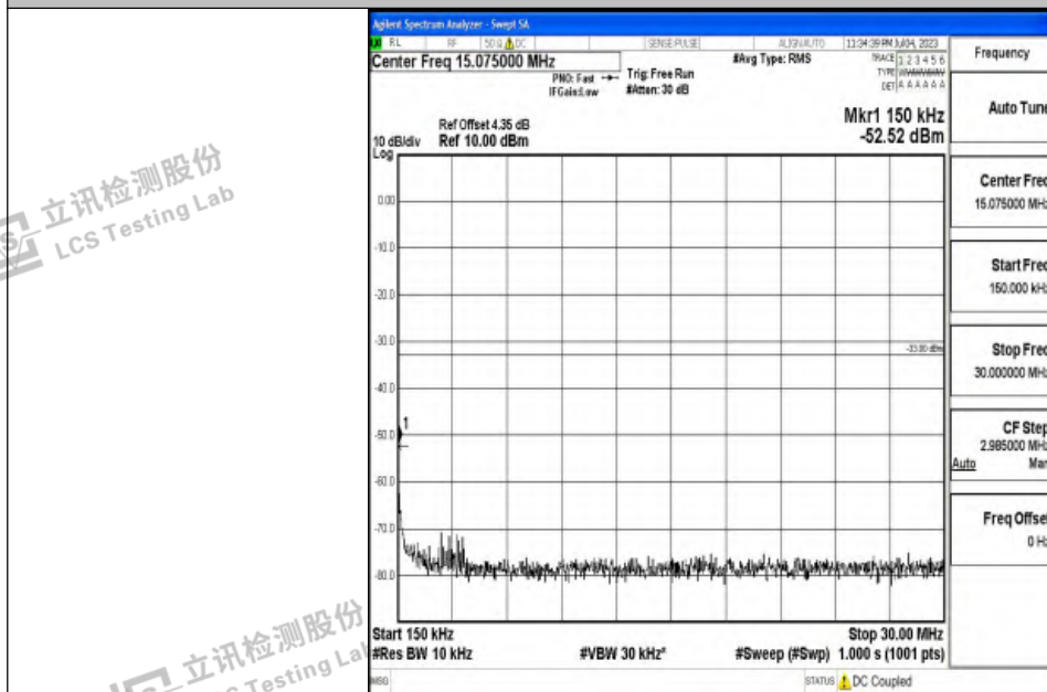
Band4_10MHz_16QAM_20350_1RB#0_0.15~30_0.15~30
