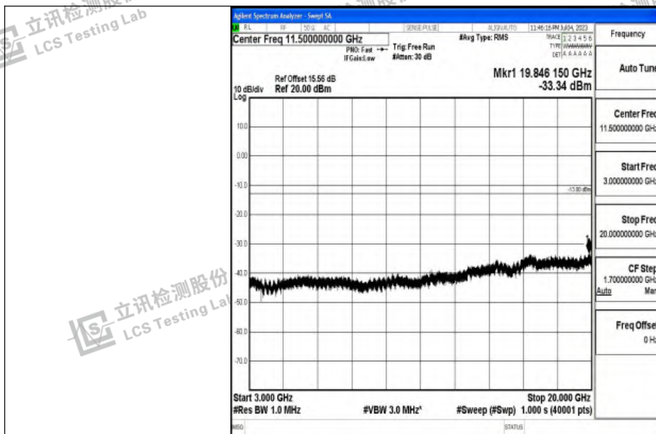
Band4_15MHz_16QAM_20025_1RB#0_3000~20000_3000~20000
