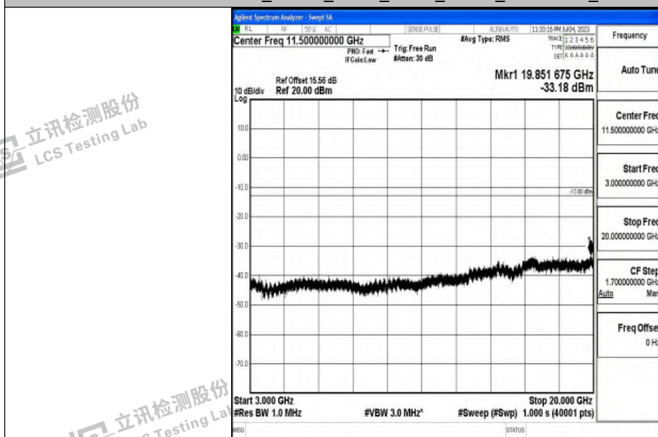
Band4_10MHz_QPSK_20175_1RB#0_3000~20000_3000~20000
