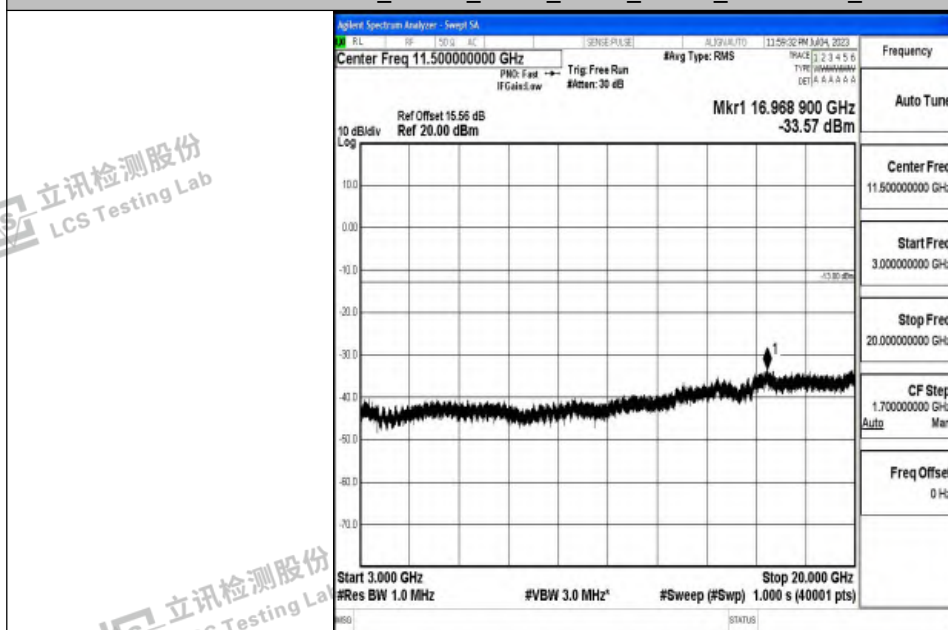
Band4_20MHz_QPSK_20050_1RB#0_3000~20000_3000~20000
