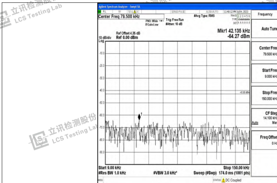
Band4_15MHz_16QAM_20325_1RB#0_0.009~0.15_0.009~0.15
