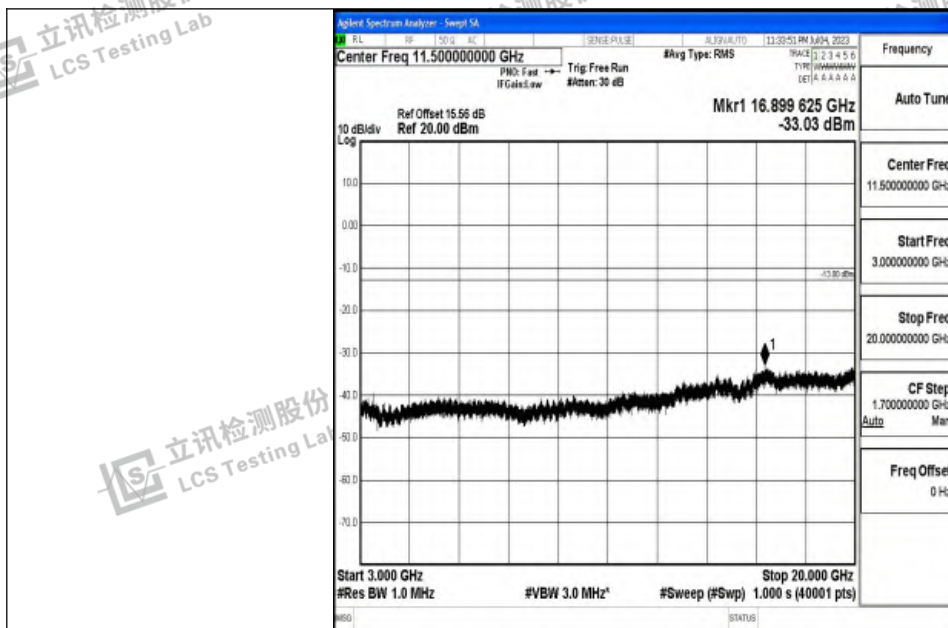
Band4_10MHz_16QAM_20175_1RB#0_3000~20000_3000~20000
