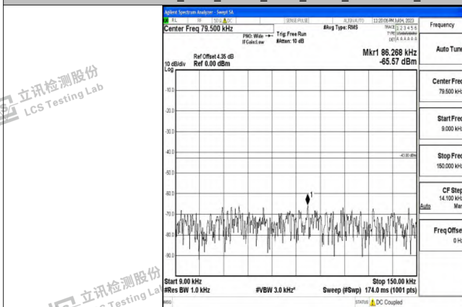
Band4_5MHz_QPSK_20375_1RB#0_0.009~0.15_0.009~0.15
