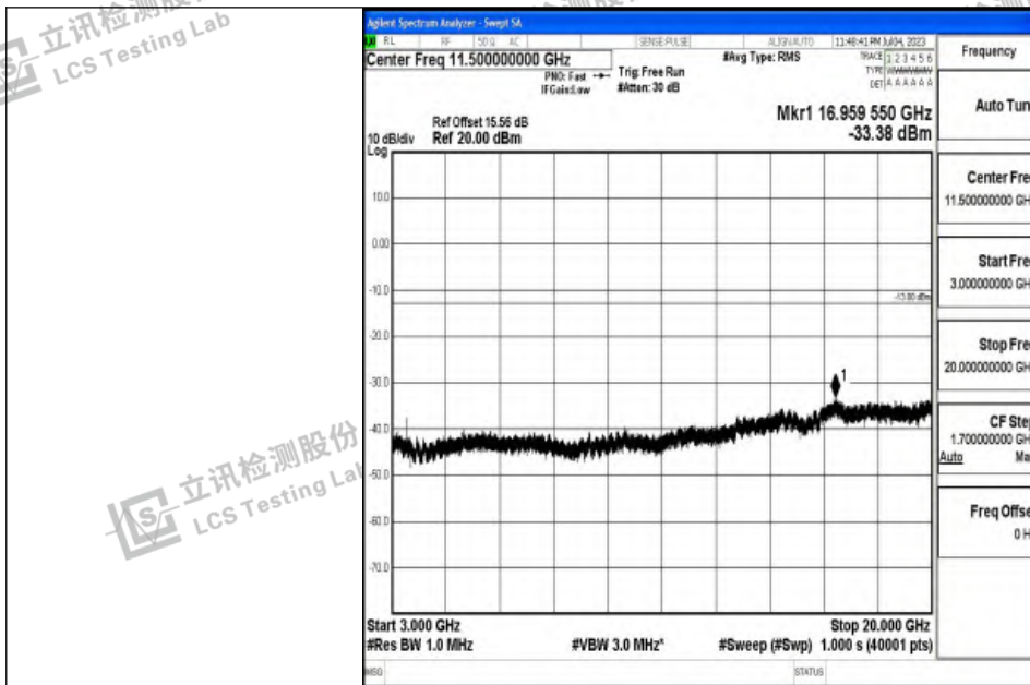
Band4_15MHz_16QAM_20325_1RB#0_3000~20000_3000~20000
