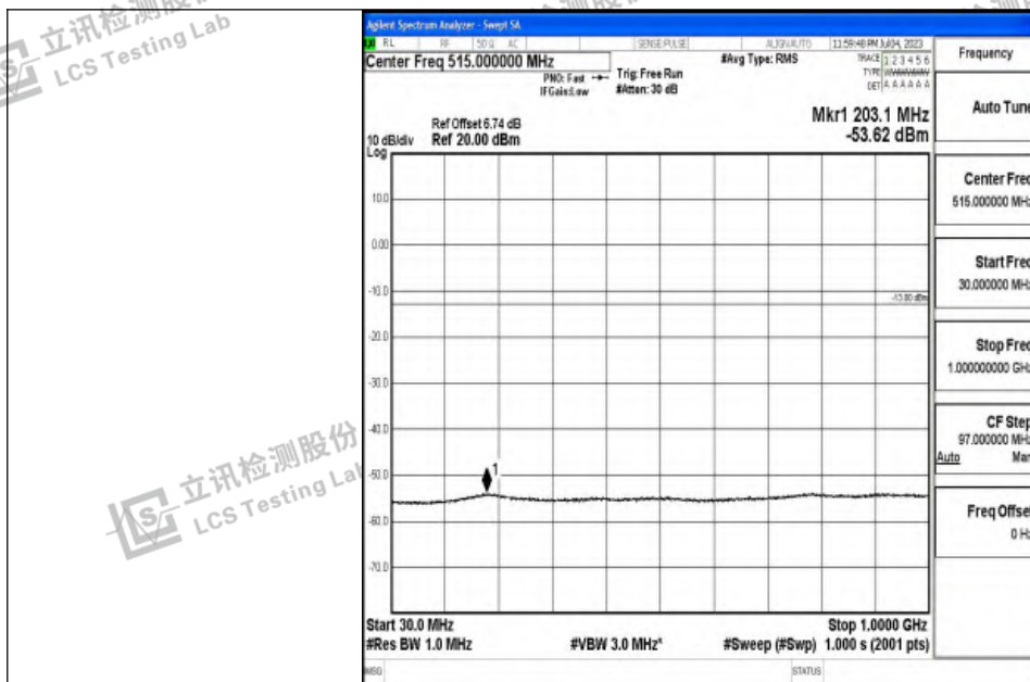
Band4_20MHz_16QAM_20050_1RB#0_30~1000_30~1000
