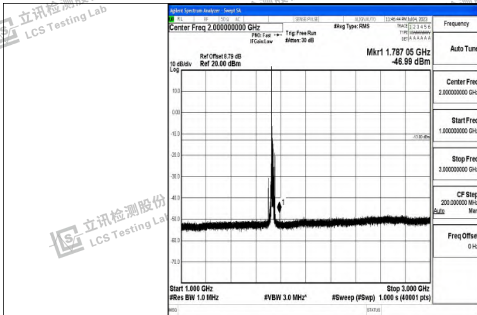
Band4_15MHz_QPSK_20175_1RB#0_1000~3000_1000~3000
