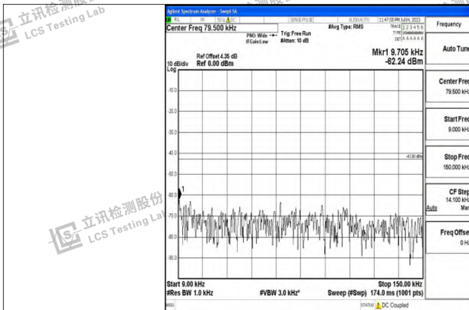
Band4_15MHz_16QAM_20175_1RB#0_0.009~0.15_0.009~0.15
