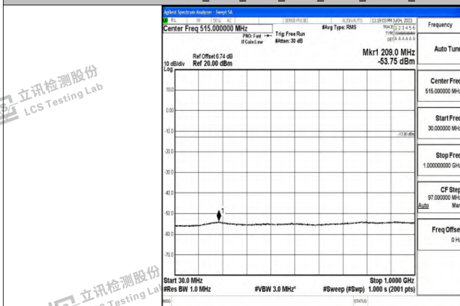
Band4_5MHz_QPSK_20175_1RB#0_30~1000_30~1000
