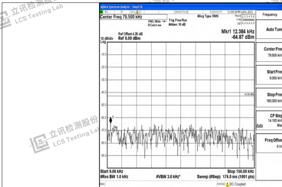
Band4_20MHz_16QAM_20050_1RB#0_0.009~0.15_0.009~0.15
