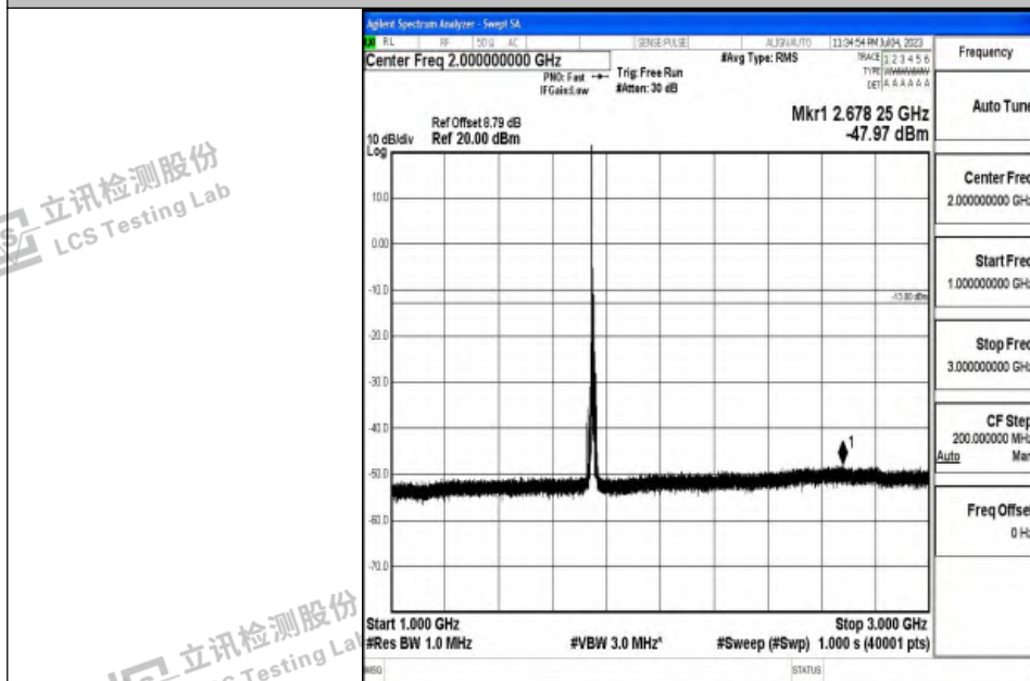
Band4_10MHz_16QAM_20350_1RB#0_1000~3000_1000~3000
