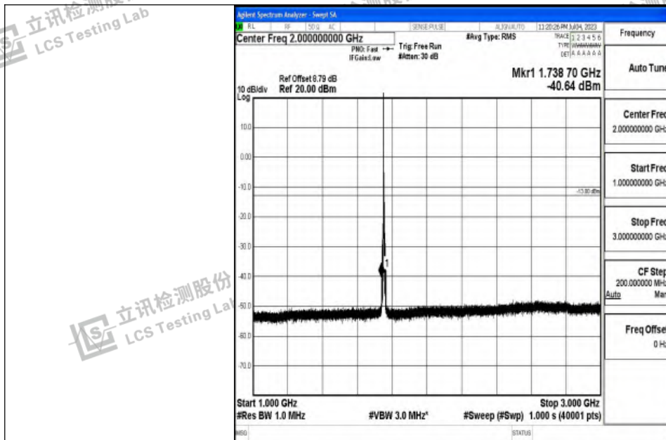
Band4_5MHz_QPSK_20375_1RB#0_1000~3000_1000~3000
