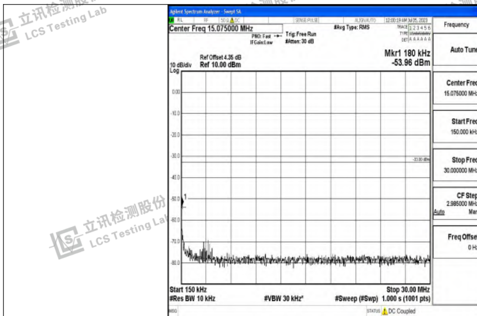
Band4_20MHz_QPSK_20175_1RB#0_0.15~30_0.15~30
