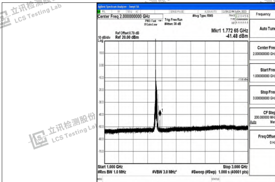
Band4_20MHz_QPSK_20050_1RB#0_1000~3000_1000~3000
