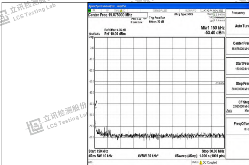
Band4_15MHz_QPSK_20325_1RB#0_0.15~30_0.15~30
