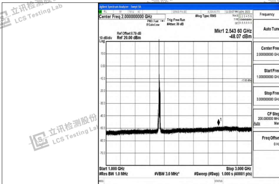
Band4_10MHz_QPSK_20175_1RB#0_1000~3000_1000~3000
