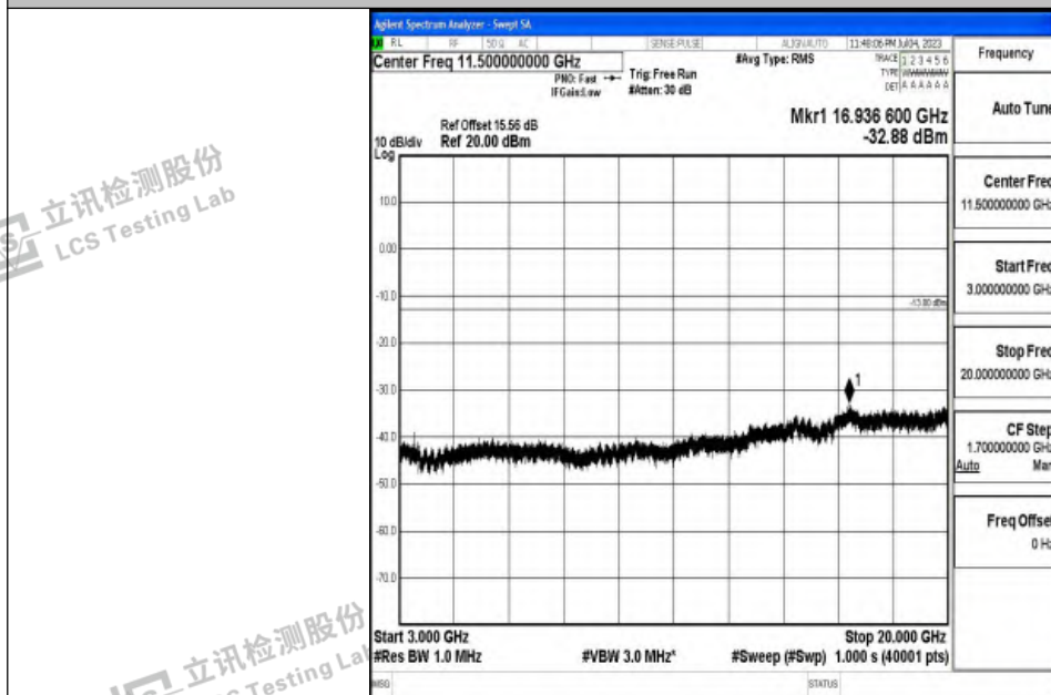
Band4_15MHz_QPSK_20325_1RB#0_3000~20000_3000~20000
