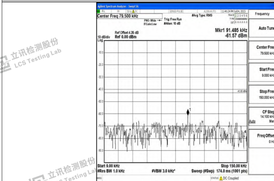
Band4_15MHz_QPSK_20175_1RB#0_0.009~0.15_0.009~0.15
