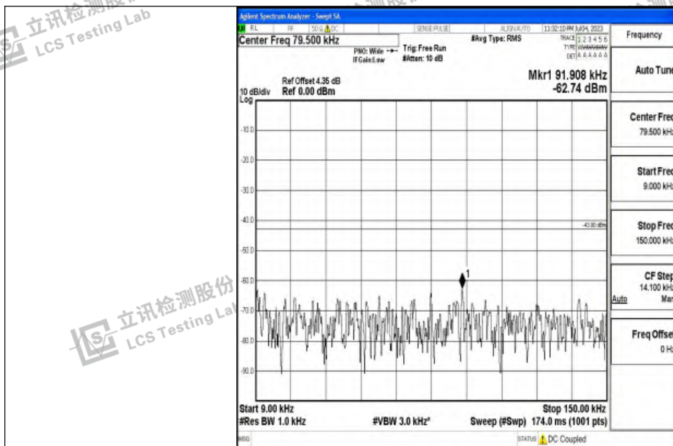
Band4_10MHz_16QAM_20000_1RB#0_0.009~0.15_0.009~0.15
