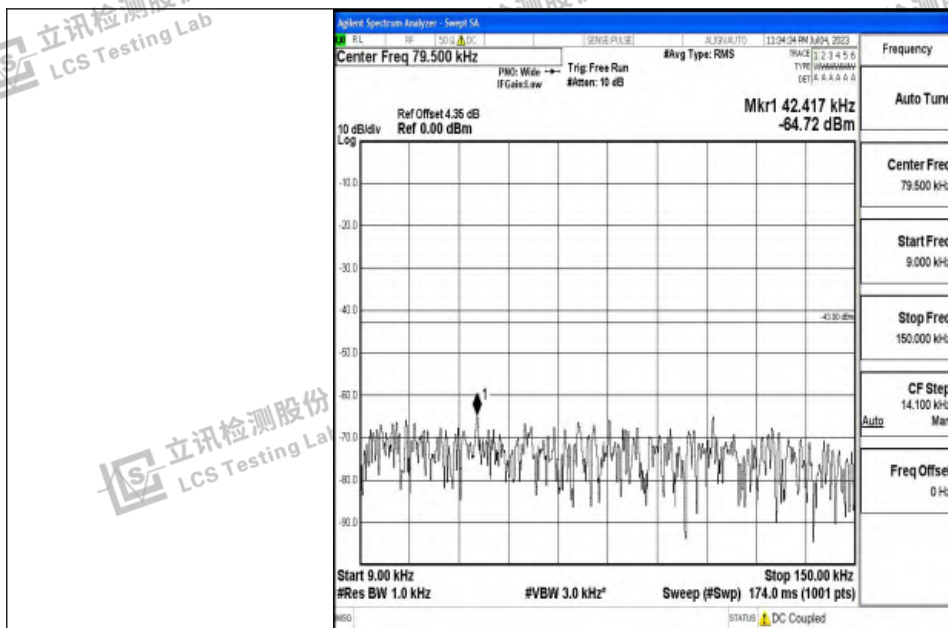
Band4_10MHz_16QAM_20350_1RB#0_0.009~0.15_0.009~0.15
