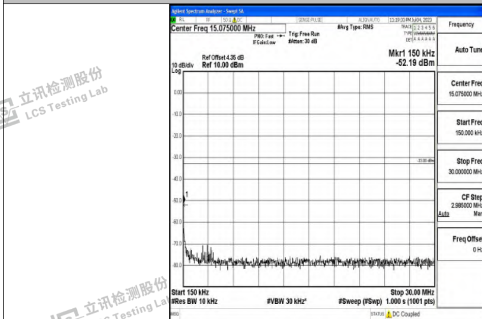
Band4_5MHz_16QAM_20175_1RB#0_0.15~30_0.15~30
