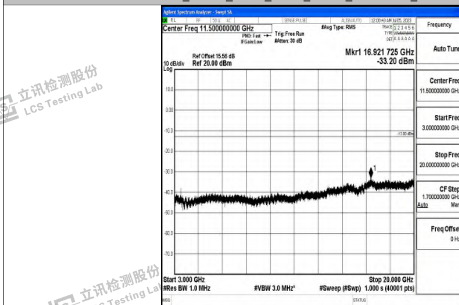
Band4_20MHz_QPSK_20175_1RB#0_3000~20000_3000~20000
