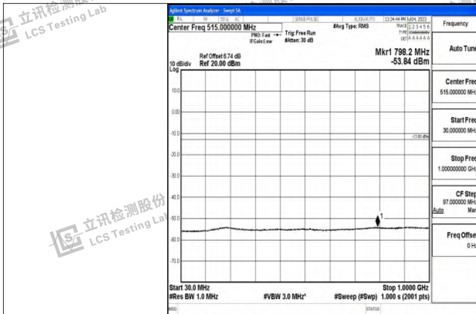
Band4_10MHz_16QAM_20350_1RB#0_30~1000_30~1000
