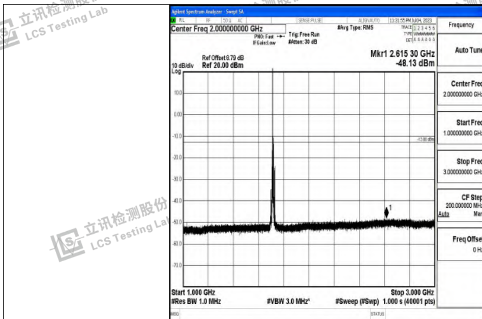
Band4_10MHz_QPSK_20000_1RB#0_1000~3000_1000~3000
