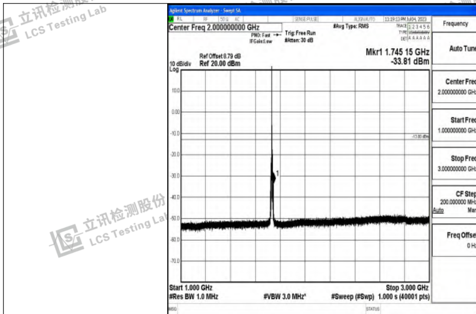
Band4_5MHz_QPSK_20175_1RB#0_1000~3000_1000~3000
