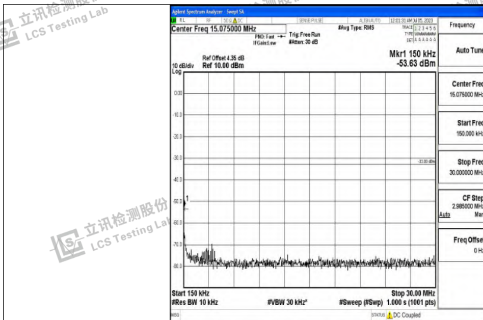
Band4_20MHz_QPSK_20300_1RB#0_0.15~30_0.15~30
