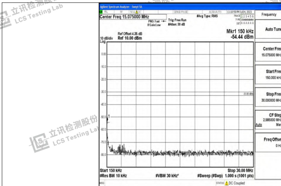
Band4_5MHz_QPSK_20175_1RB#0_0.15~30_0.15~30
