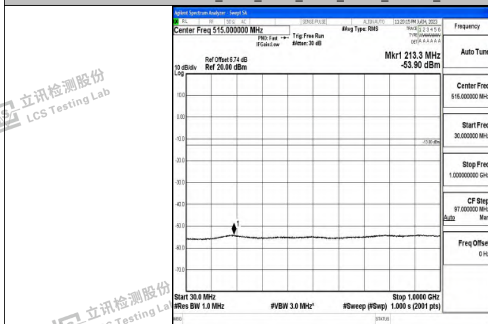
Band4_5MHz_QPSK_20375_1RB#0_30~1000_30~1000
