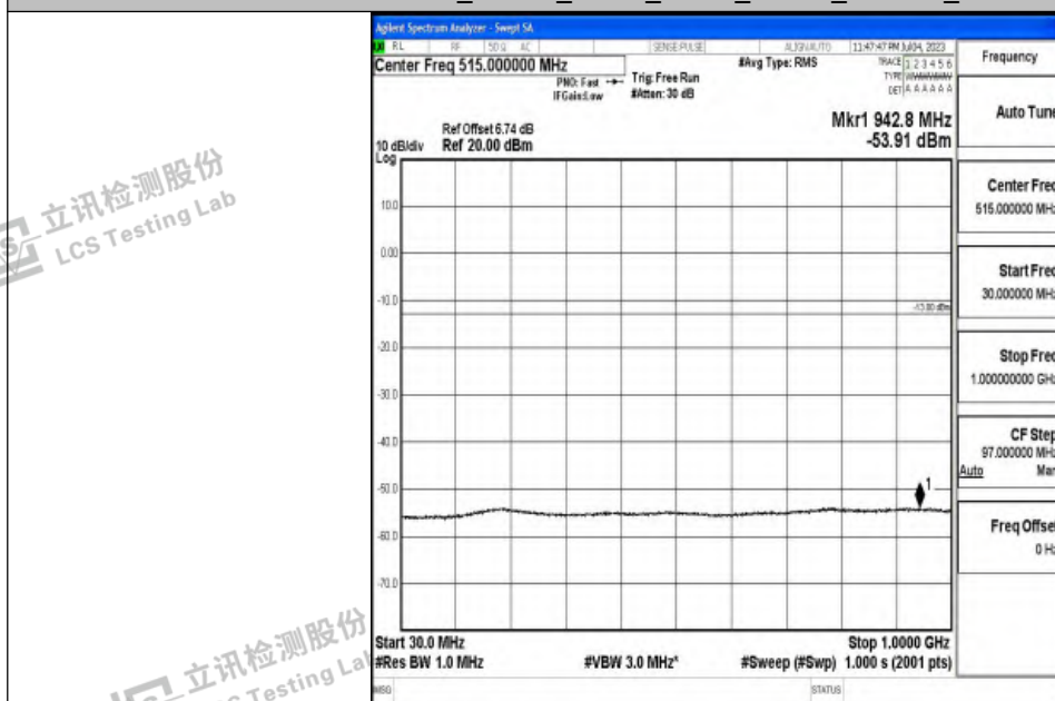
Band4_15MHz_QPSK_20325_1RB#0_30~1000_30~1000
