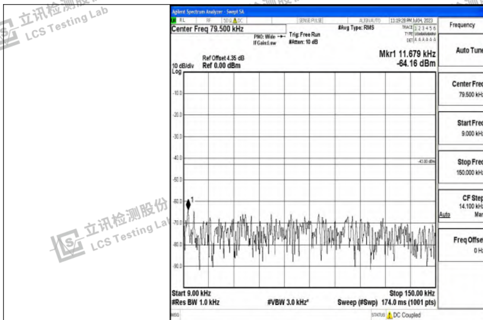
Band4_5MHz_16QAM_20175_1RB#0_0.009~0.15_0.009~0.15
