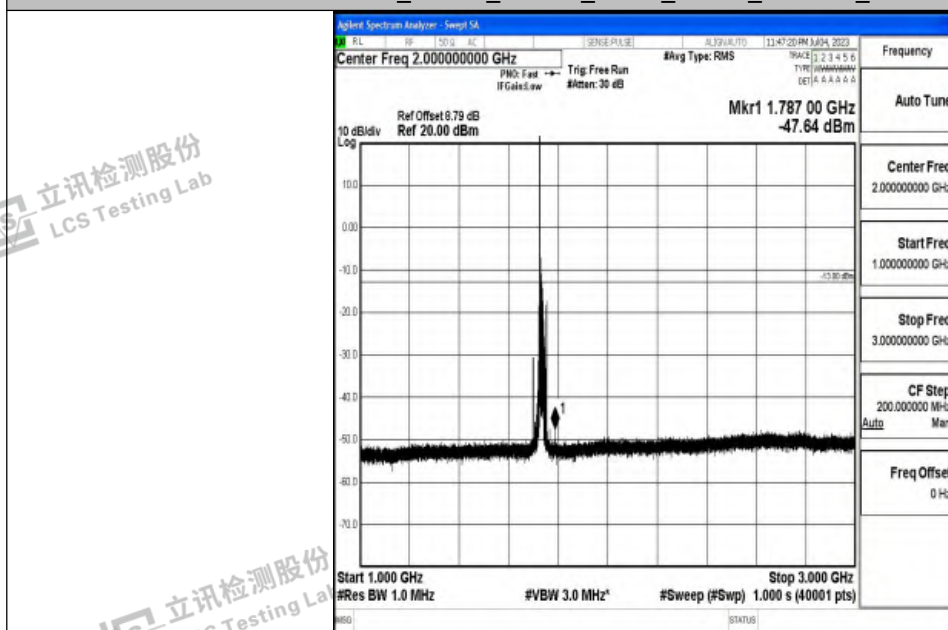
Band4_15MHz_16QAM_20175_1RB#0_1000~3000_1000~3000
