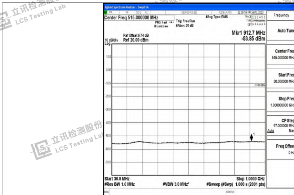
Band4_20MHz_16QAM_20175_1RB#0_30~1000_30~1000
