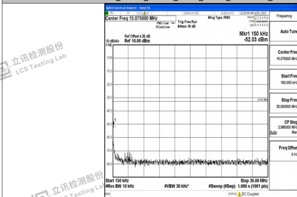
Band4_20MHz_16QAM_20175_1RB#0_0.15~30_0.15~30
