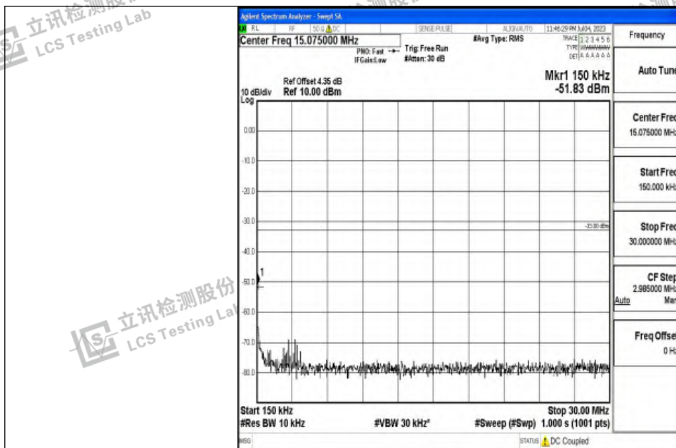
Band4_15MHz_QPSK_20175_1RB#0_0.15~30_0.15~30
