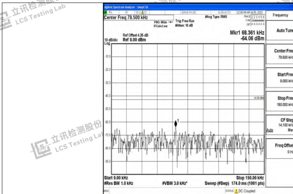
Band4_20MHz_16QAM_20175_1RB#0_0.009~0.15_0.009~0.15
