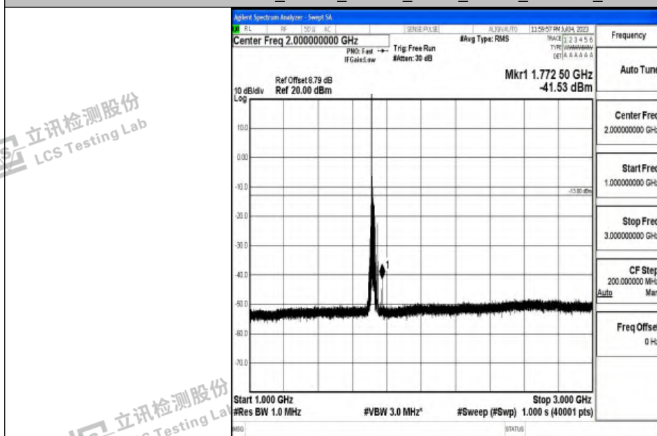
Band4_20MHz_16QAM_20050_1RB#0_1000~3000_1000~3000
