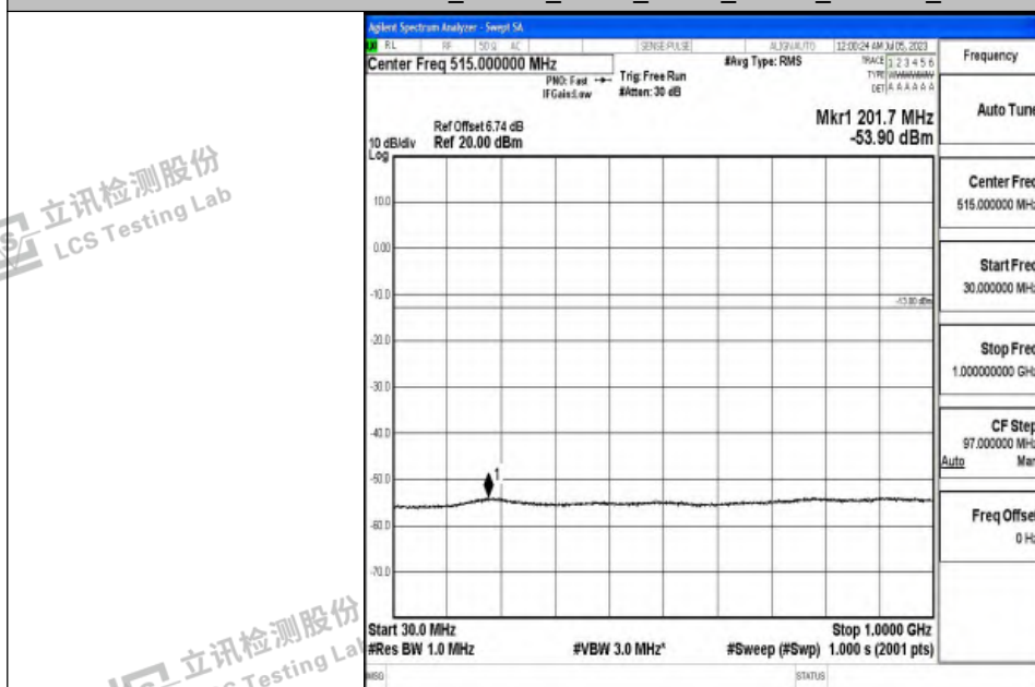
Band4_20MHz_QPSK_20175_1RB#0_30~1000_30~1000
