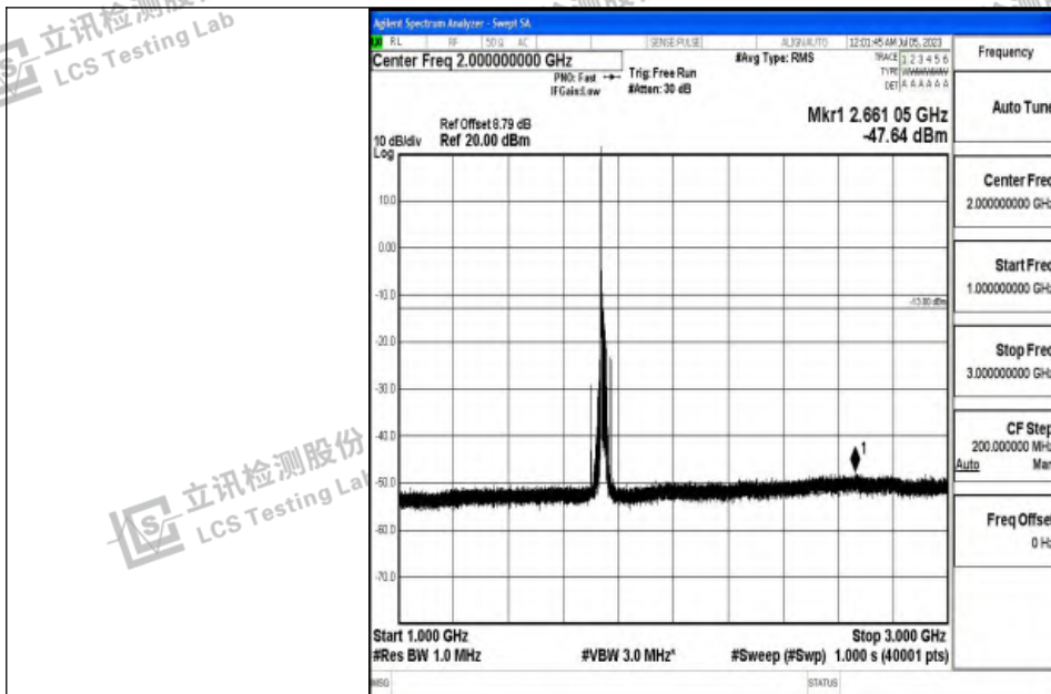
Band4_20MHz_QPSK_20300_1RB#0_1000~3000_1000~3000
