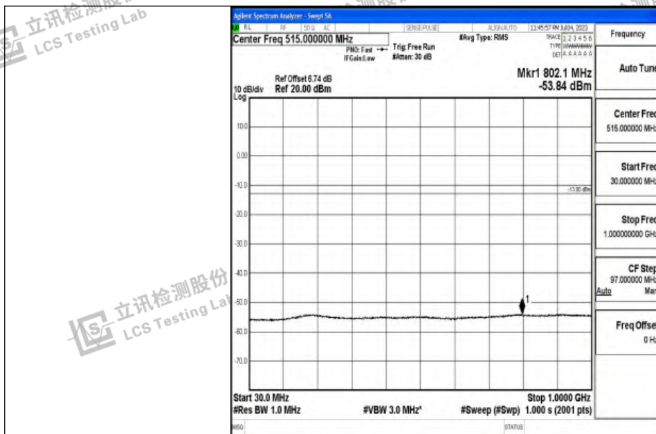
Band4_15MHz_16QAM_20025_1RB#0_30~1000_30~1000
