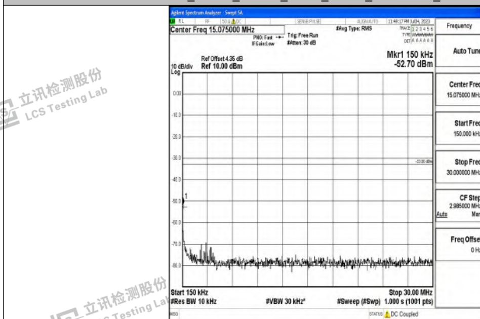
Band4_15MHz_16QAM_20325_1RB#0_0.15~30_0.15~30
