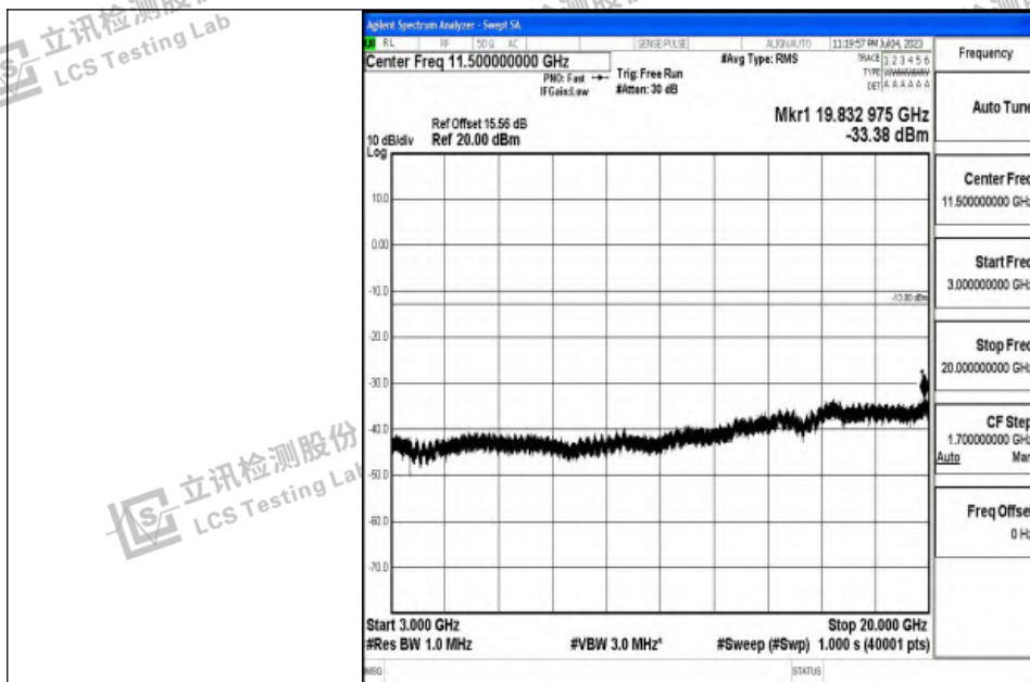
Band4_5MHz_16QAM_20175_1RB#0_3000~20000_3000~20000
