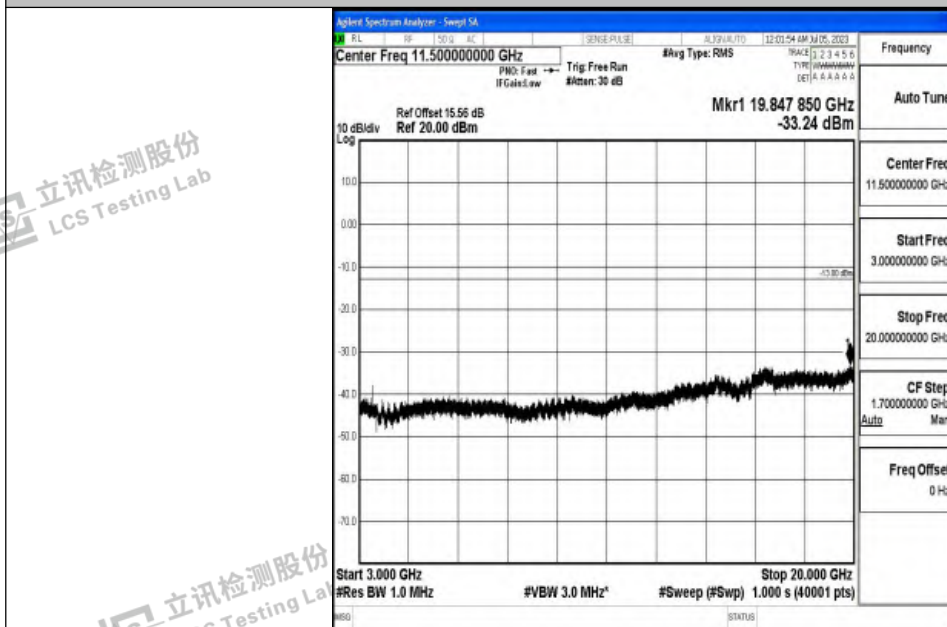
Band4_20MHz_QPSK_20300_1RB#0_3000~20000_3000~20000
