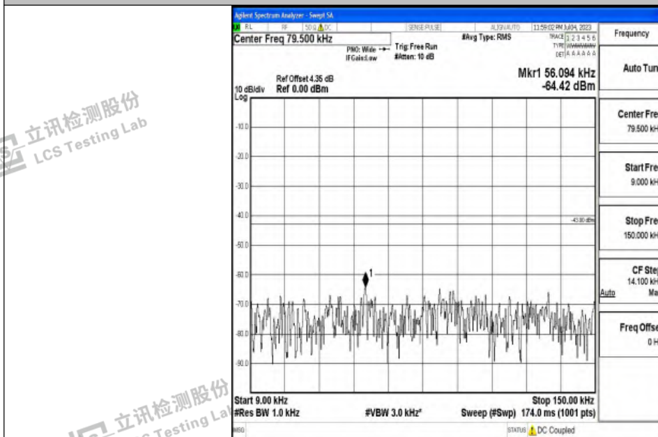
Band4_20MHz_QPSK_20050_1RB#0_0.009~0.15_0.009~0.15
