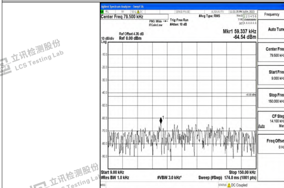
Band4_10MHz_QPSK_20000_1RB#0_0.009~0.15_0.009~0.15
