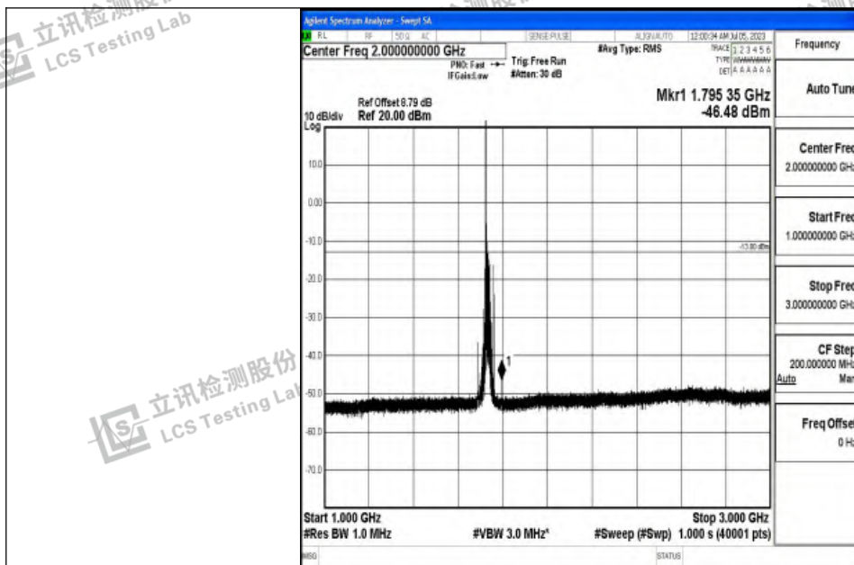
Band4_20MHz_QPSK_20175_1RB#0_1000~3000_1000~3000
