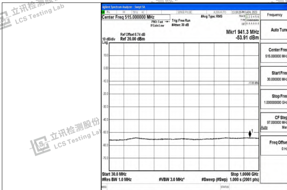
Band4_5MHz_16QAM_19975_1RB#0_30~1000_30~1000
