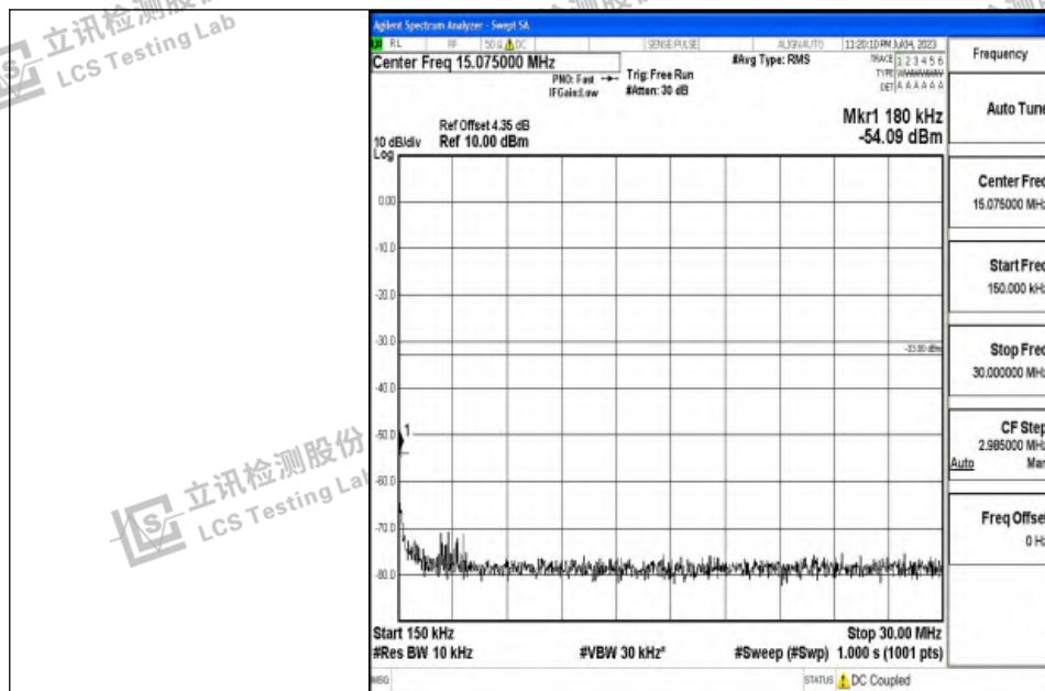
Band4_5MHz_QPSK_20375_1RB#0_0.15~30_0.15~30
