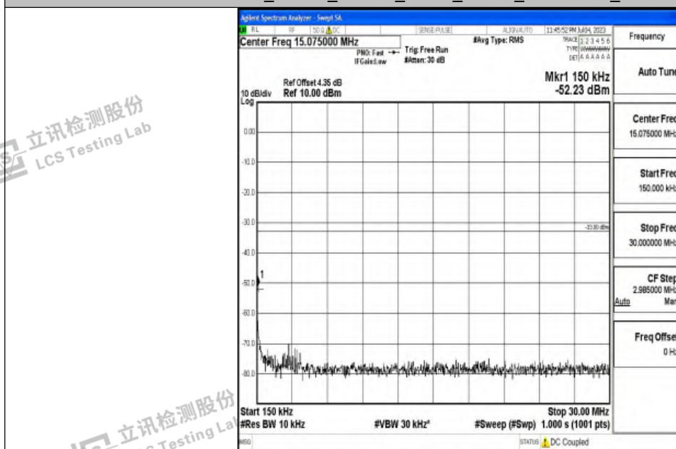
Band4_15MHz_16QAM_20025_1RB#0_0.15~30_0.15~30
