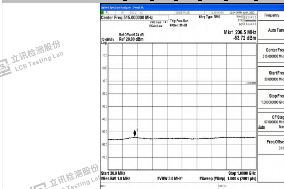
Band4_10MHz_QPSK_20350_1RB#0_30~1000_30~1000
