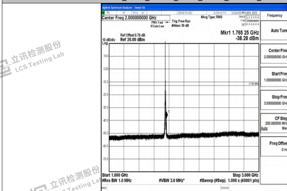
Band4_5MHz_16QAM_20375_1RB#0_1000~3000_1000~3000
