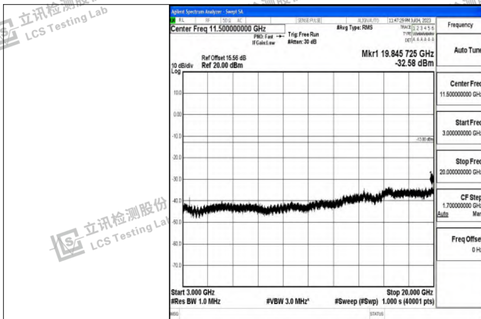
Band4_15MHz_16QAM_20175_1RB#0_3000~20000_3000~20000
