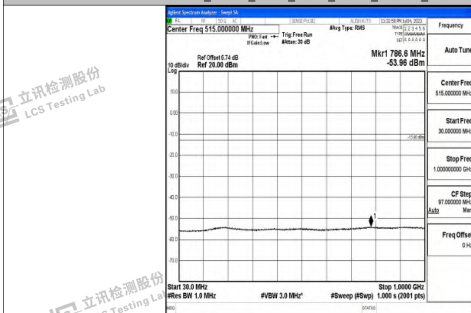
Band4_10MHz_QPSK_20175_1RB#0_30~1000_30~1000
