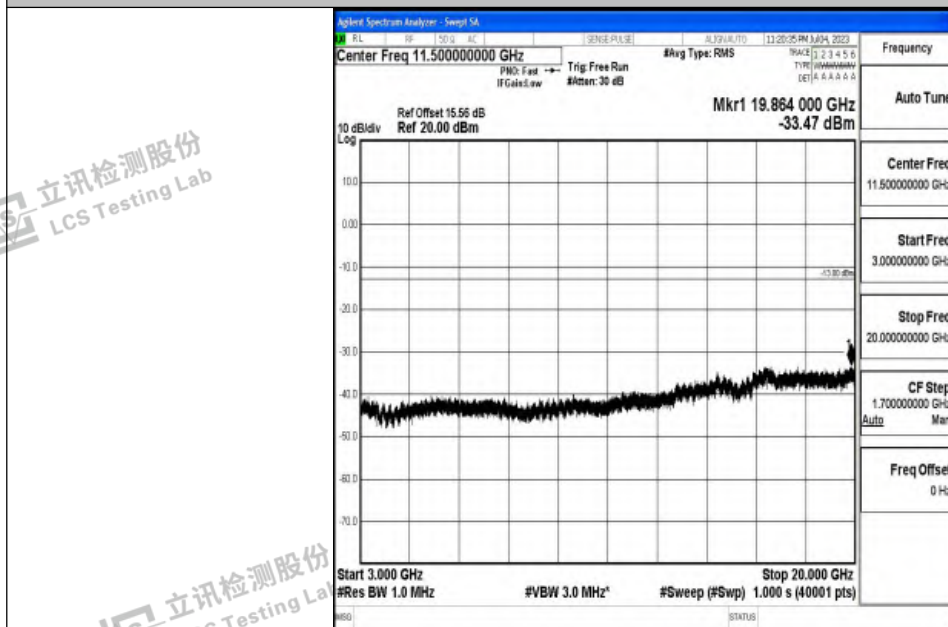
Band4_5MHz_QPSK_20375_1RB#0_3000~20000_3000~20000
