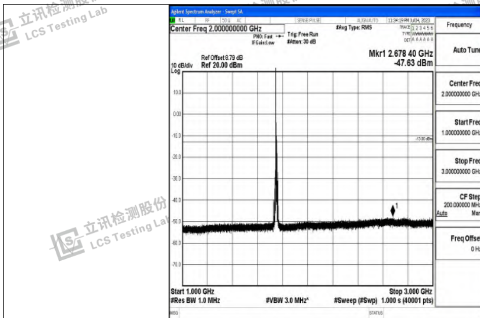
Band4_10MHz_QPSK_20350_1RB#0_1000~3000_1000~3000
