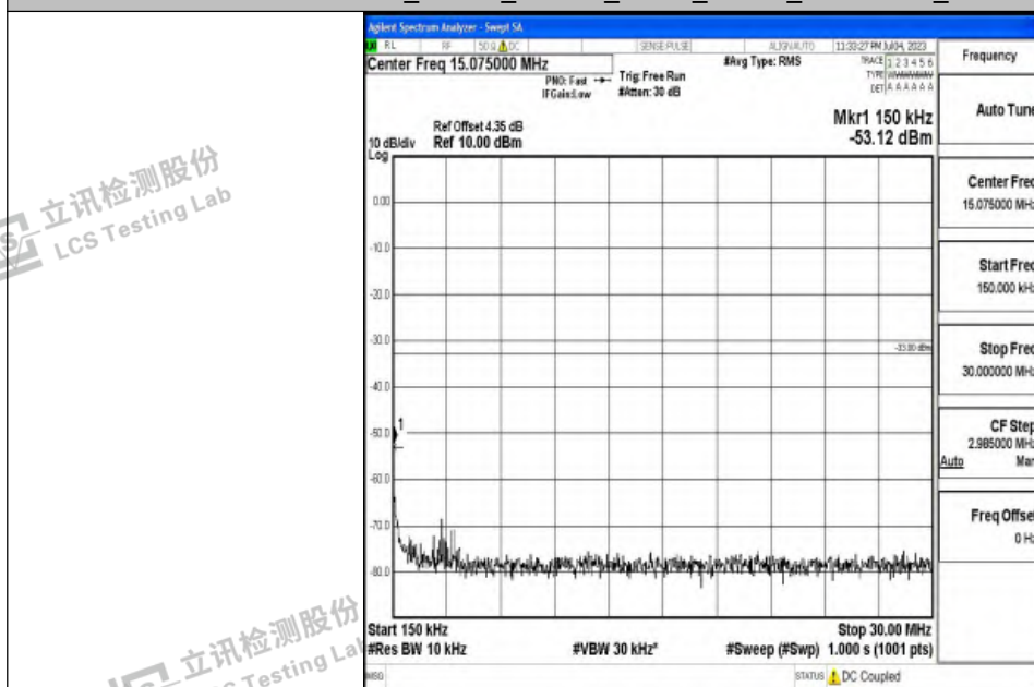
Band4_10MHz_16QAM_20175_1RB#0_0.15~30_0.15~30
