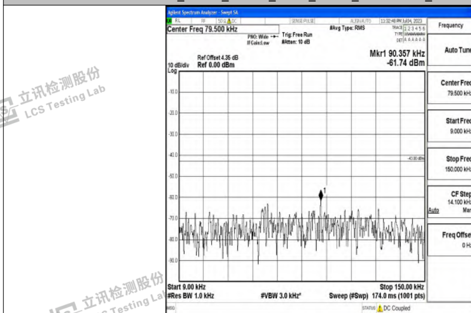
Band4_10MHz_QPSK_20175_1RB#0_0.009~0.15_0.009~0.15
