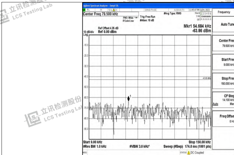
Band4_15MHz_16QAM_20025_1RB#0_0.009~0.15_0.009~0.15
