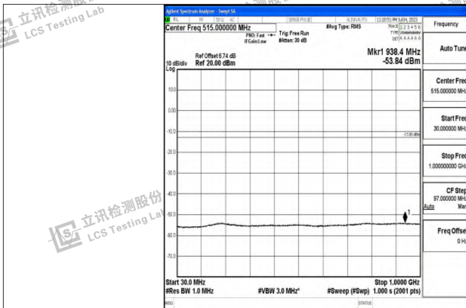
Band4_5MHz_16QAM_20375_1RB#0_30~1000_30~1000
