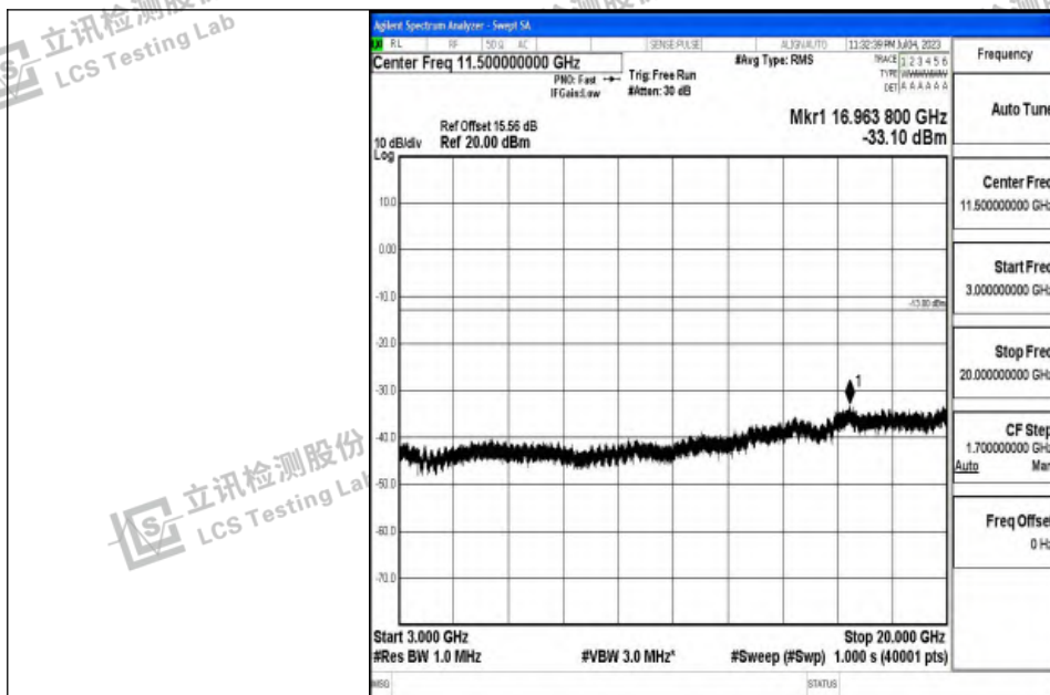
Band4_10MHz_16QAM_20000_1RB#0_3000~20000_3000~20000
