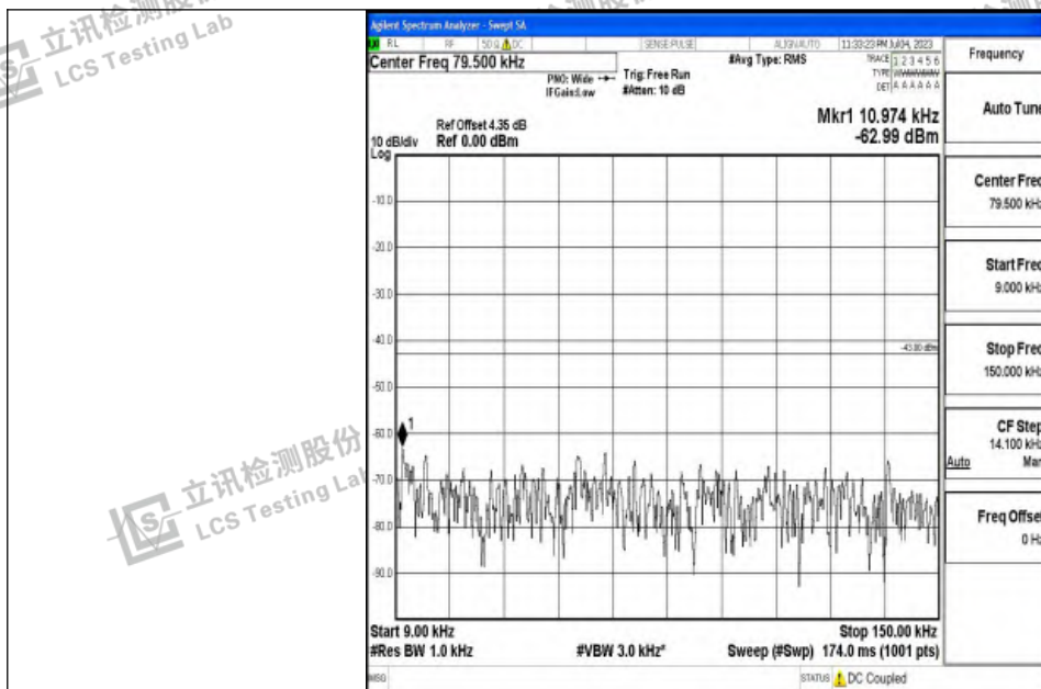
Band4_10MHz_16QAM_20175_1RB#0_0.009~0.15_0.009~0.15
