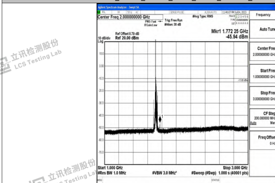
Band4_15MHz_16QAM_20025_1RB#0_1000~3000_1000~3000
