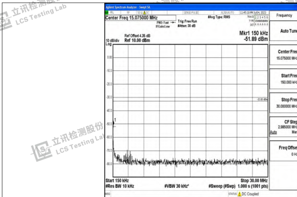
Band4_15MHz_QPSK_20025_1RB#0_0.15~30_0.15~30
