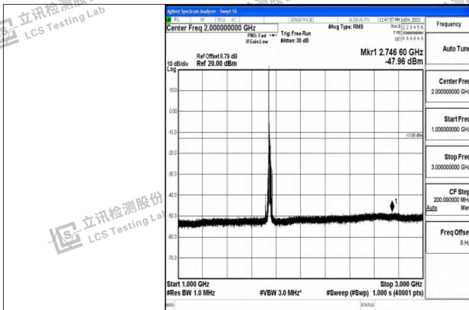
Band4_15MHz_QPSK_20325_1RB#0_1000~3000_1000~3000
