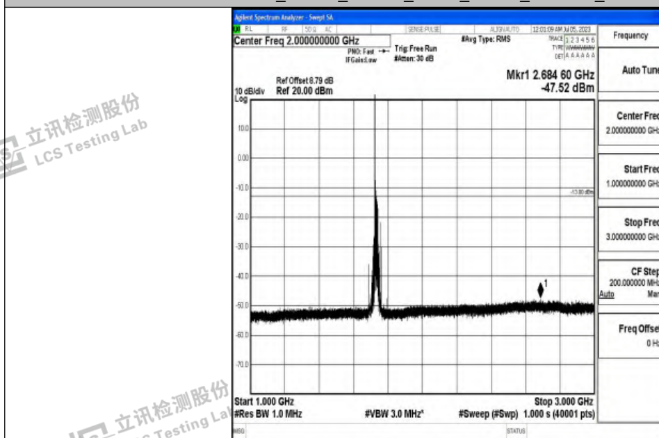
Band4_20MHz_16QAM_20175_1RB#0_1000~3000_1000~3000
