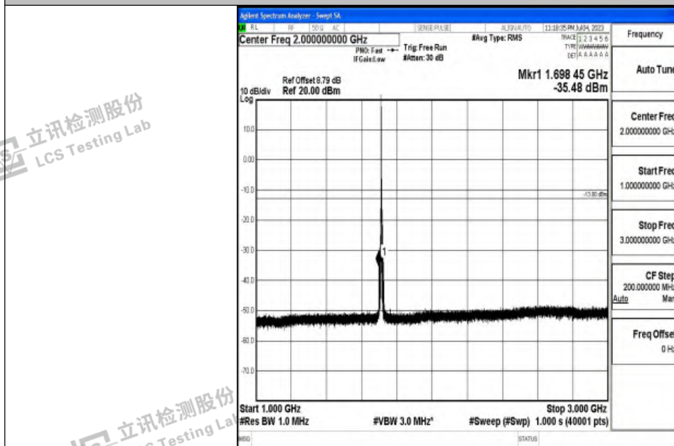
Band4_5MHz_16QAM_19975_1RB#0_1000~3000_1000~3000
