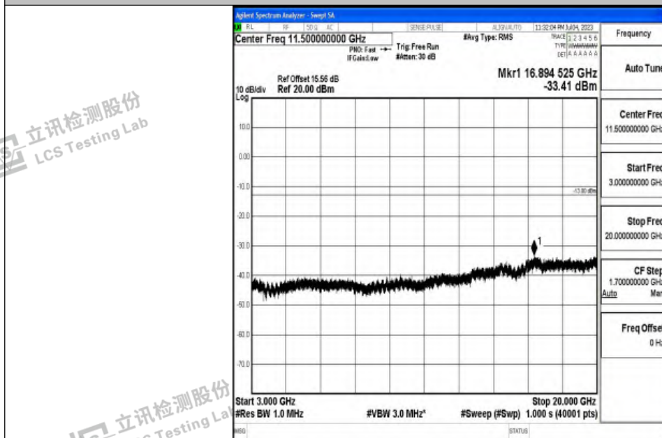
Band4_10MHz_QPSK_20000_1RB#0_3000~20000_3000~20000
