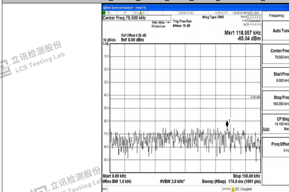
Band4_20MHz_QPSK_20175_1RB#0_0.009~0.15_0.009~0.15
