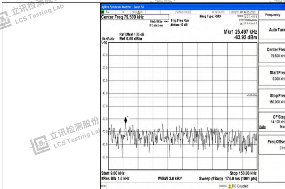
Band4_20MHz_16QAM_20300_1RB#0_0.009~0.15_0.009~0.15
