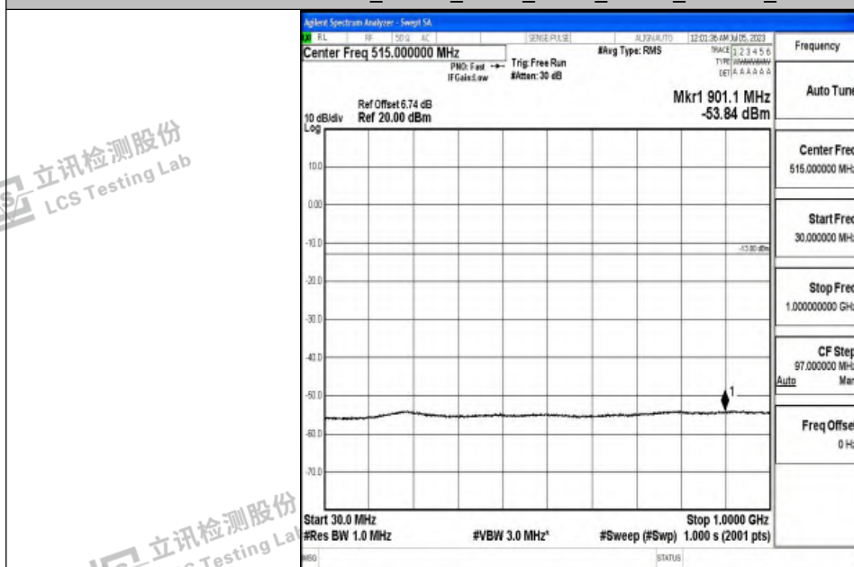
Band4_20MHz_QPSK_20300_1RB#0_30~1000_30~1000
