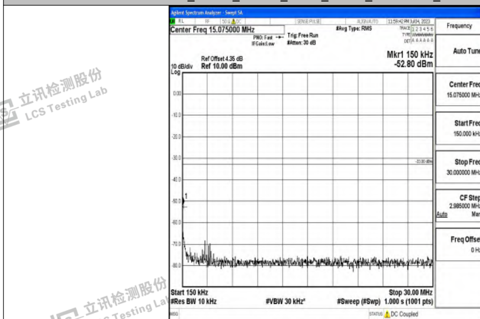
Band4_20MHz_16QAM_20050_1RB#0_0.15~30_0.15~30
