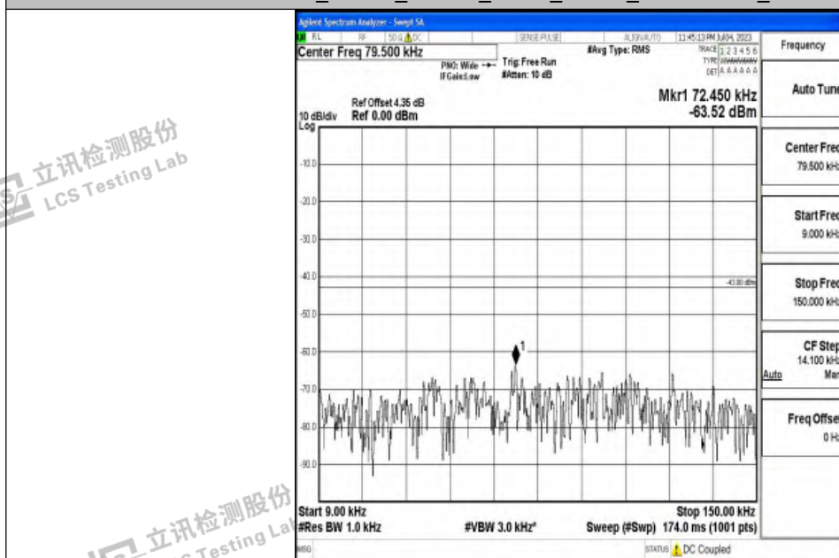
Band4_15MHz_QPSK_20025_1RB#0_0.009~0.15_0.009~0.15
