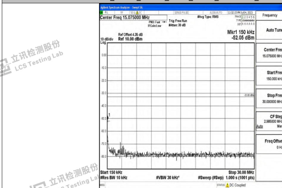
Band4_10MHz_16QAM_20000_1RB#0_0.15~30_0.15~30
