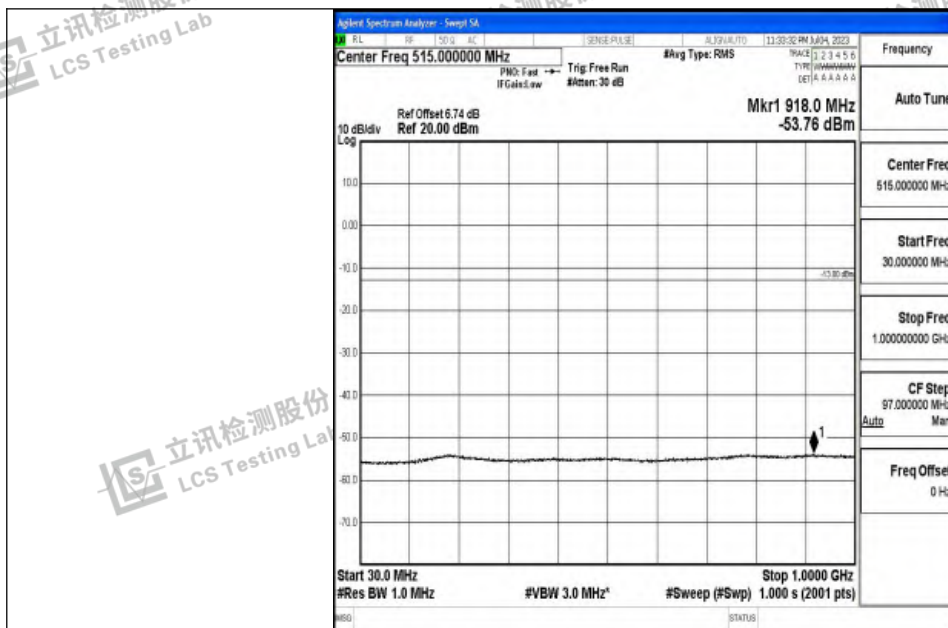
Band4_10MHz_16QAM_20175_1RB#0_30~1000_30~1000
