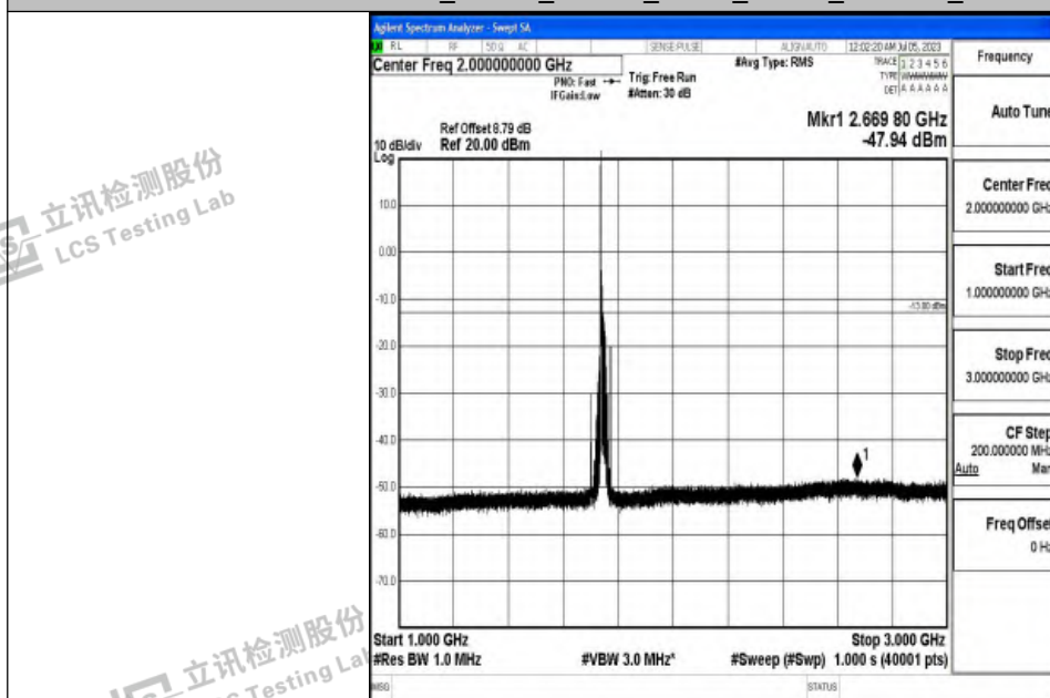
Band4_20MHz_16QAM_20300_1RB#0_1000~3000_1000~3000
