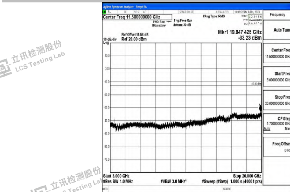
Band4_5MHz_QPSK_20175_1RB#0_3000~20000_3000~20000
