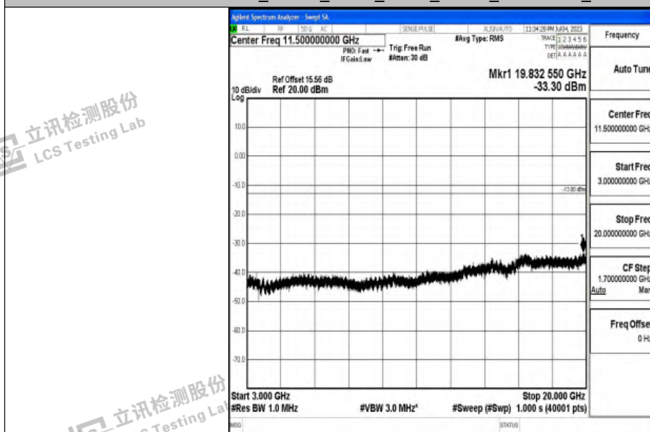
Band4_10MHz_QPSK_20350_1RB#0_3000~20000_3000~20000
