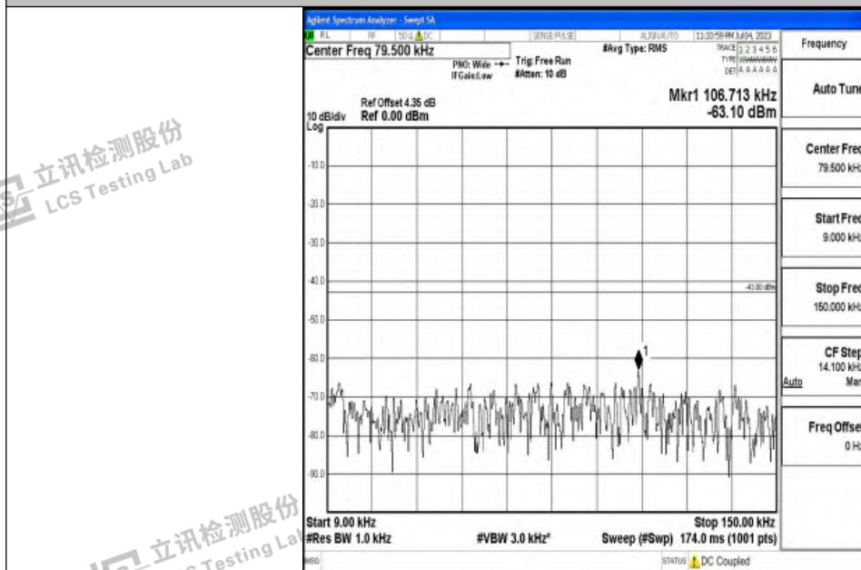
Band4_10MHz_QPSK_20350_1RB#0_0.009~0.15_0.009~0.15
