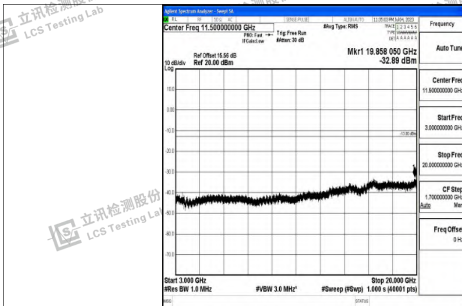
Band4_10MHz_16QAM_20350_1RB#0_3000~20000_3000~20000
