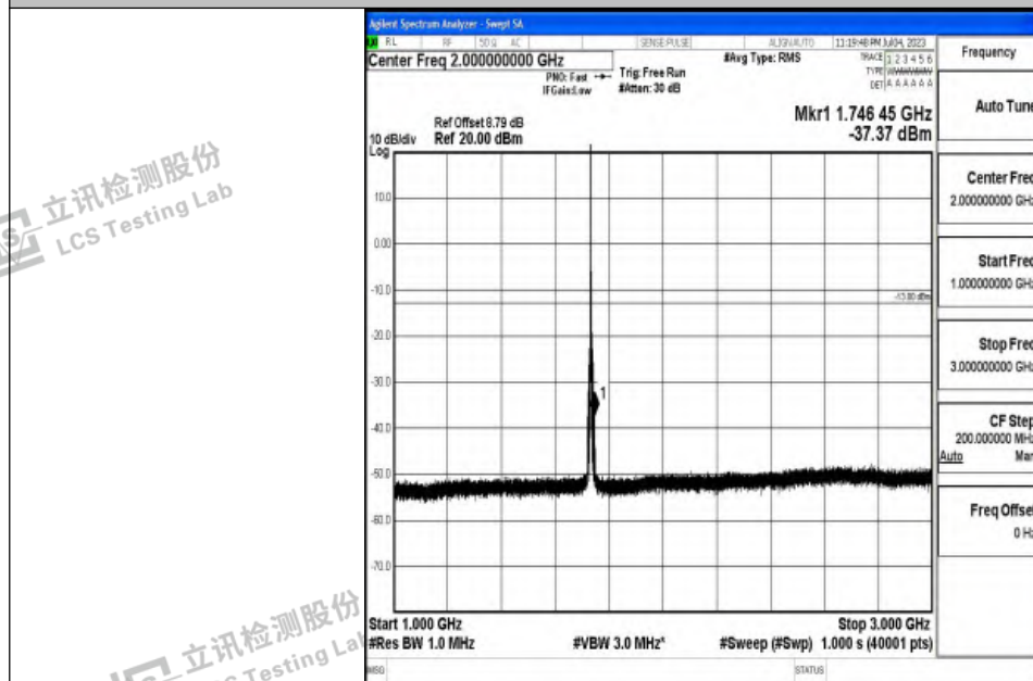
Band4_5MHz_16QAM_20175_1RB#0_1000~3000_1000~3000
