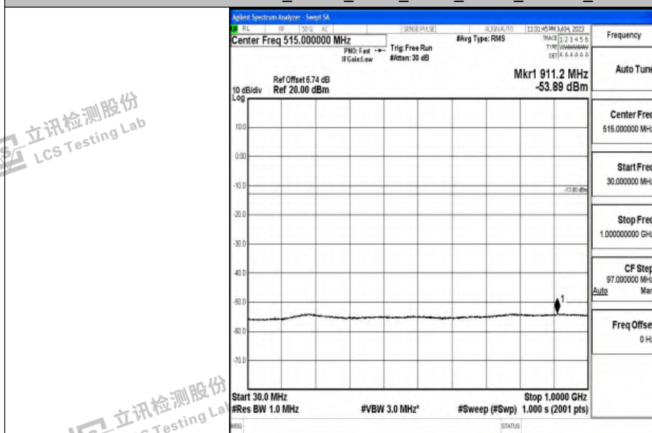
Band4_10MHz_QPSK_20000_1RB#0_30~1000_30~1000
