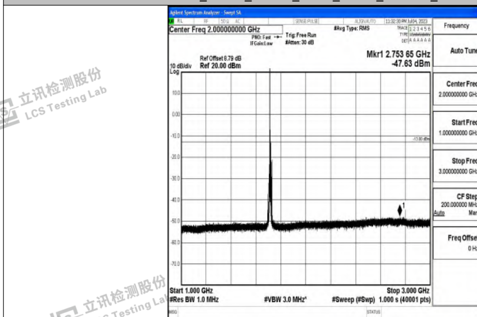
Band4_10MHz_16QAM_20000_1RB#0_1000~3000_1000~3000
