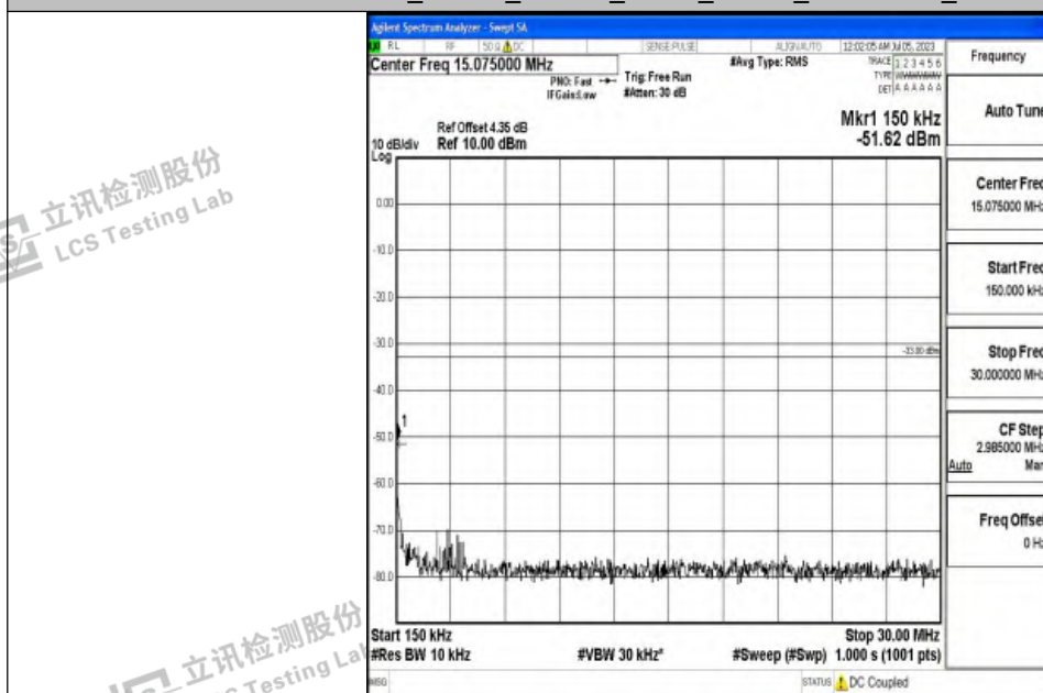
Band4_20MHz_16QAM_20300_1RB#0_0.15~30_0.15~30
