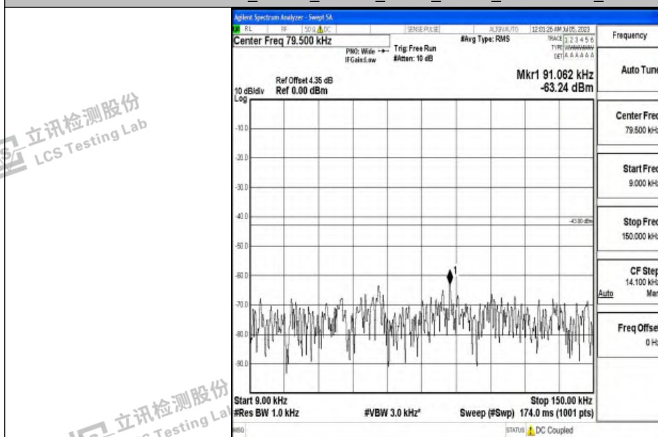
Band4_20MHz_QPSK_20300_1RB#0_0.009~0.15_0.009~0.15
