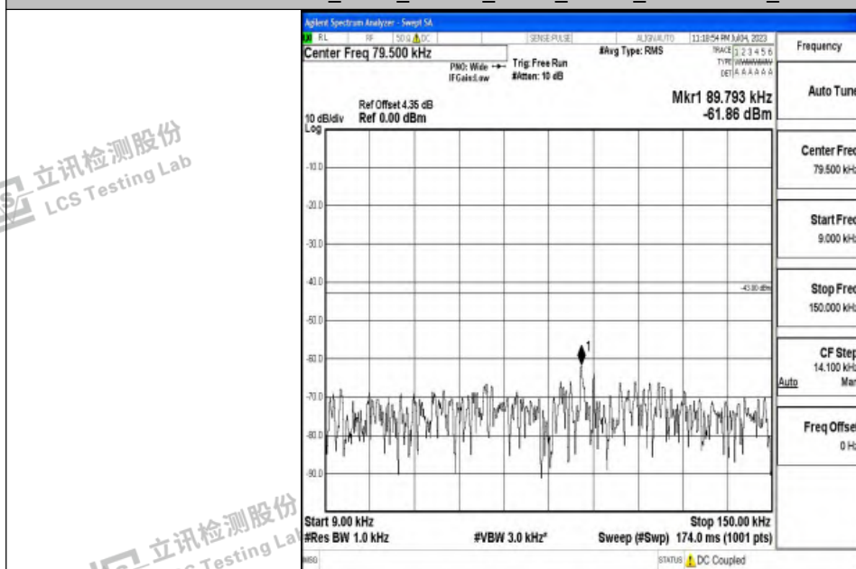
Band4_5MHz_QPSK_20175_1RB#0_0.009~0.15_0.009~0.15
