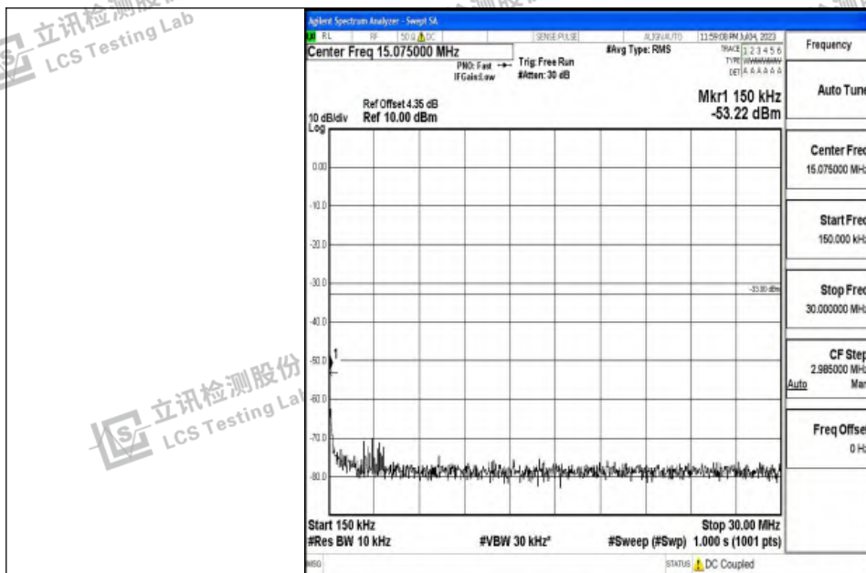
Band4_20MHz_QPSK_20050_1RB#0_0.15~30_0.15~30
