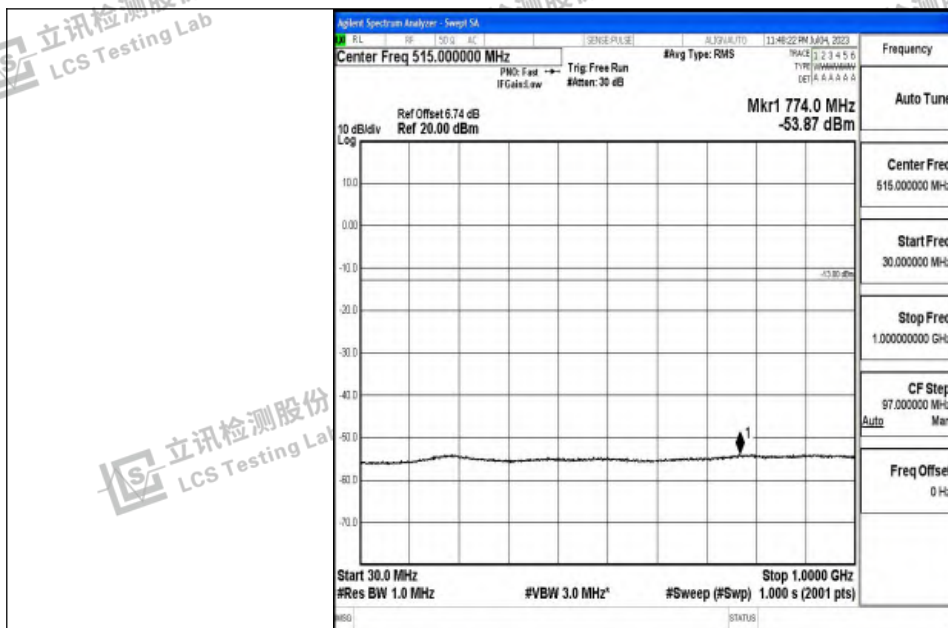
Band4_15MHz_16QAM_20325_1RB#0_30~1000_30~1000
