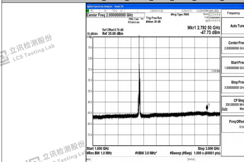
Band4_10MHz_16QAM_20175_1RB#0_1000~3000_1000~3000
