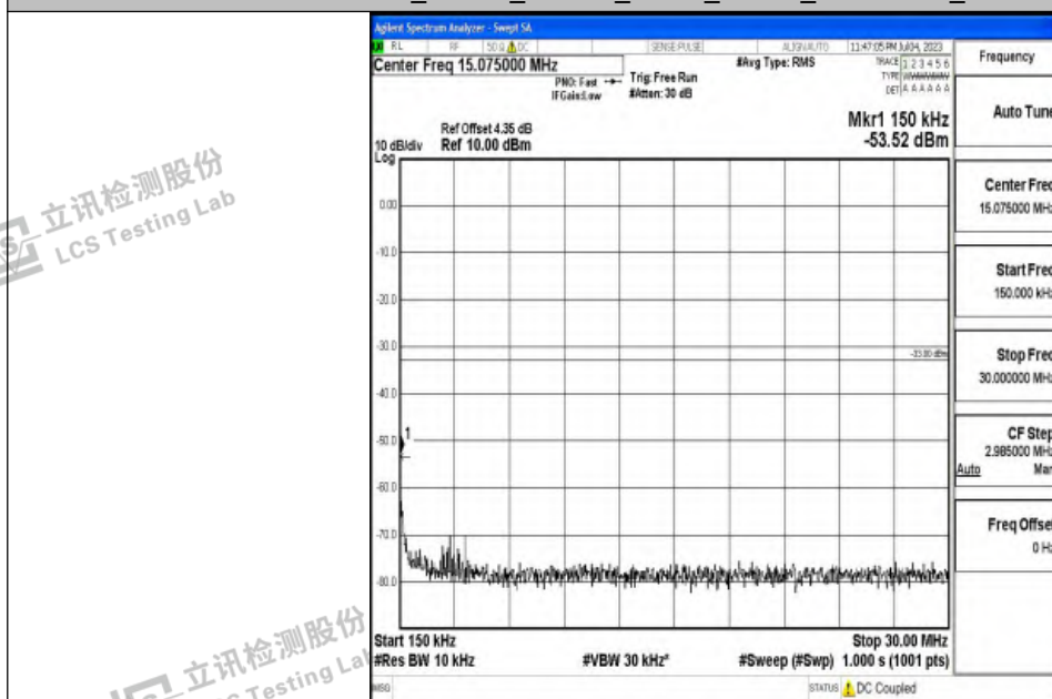
Band4_15MHz_16QAM_20175_1RB#0_0.15~30_0.15~30
