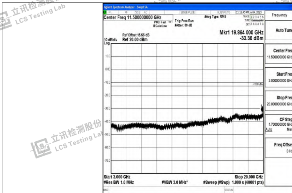
Band4_5MHz_16QAM_19975_1RB#0_3000~20000_3000~20000
