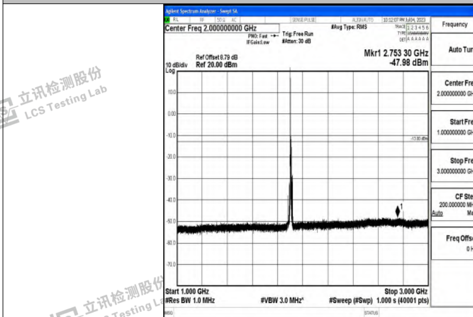
Band2_10MHz_16QAM_19150_1RB#0_1000~3000_1000~3000
