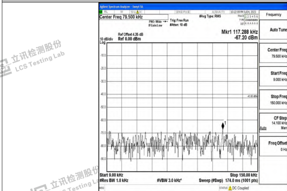
Band2_15MHz_QPSK_18675_1RB#0_0.009~0.15_0.009~0.15
