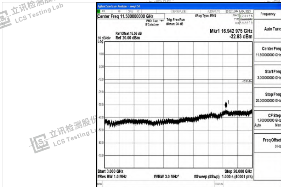
Band2_10MHz_16QAM_19150_1RB#0_3000~20000_3000~20000
