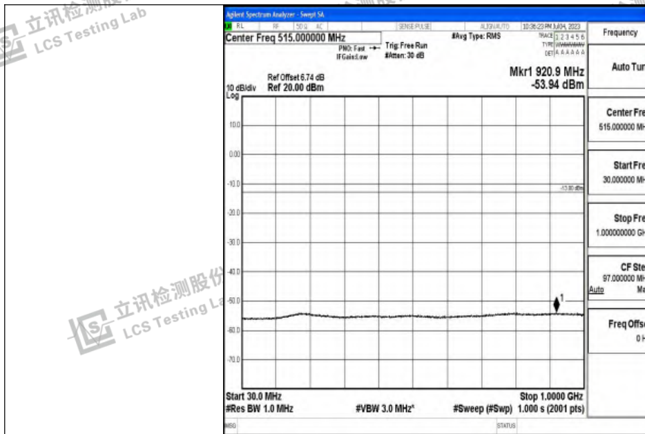
Band2_20MHz_16QAM_18700_1RB#0_30~1000_30~1000
