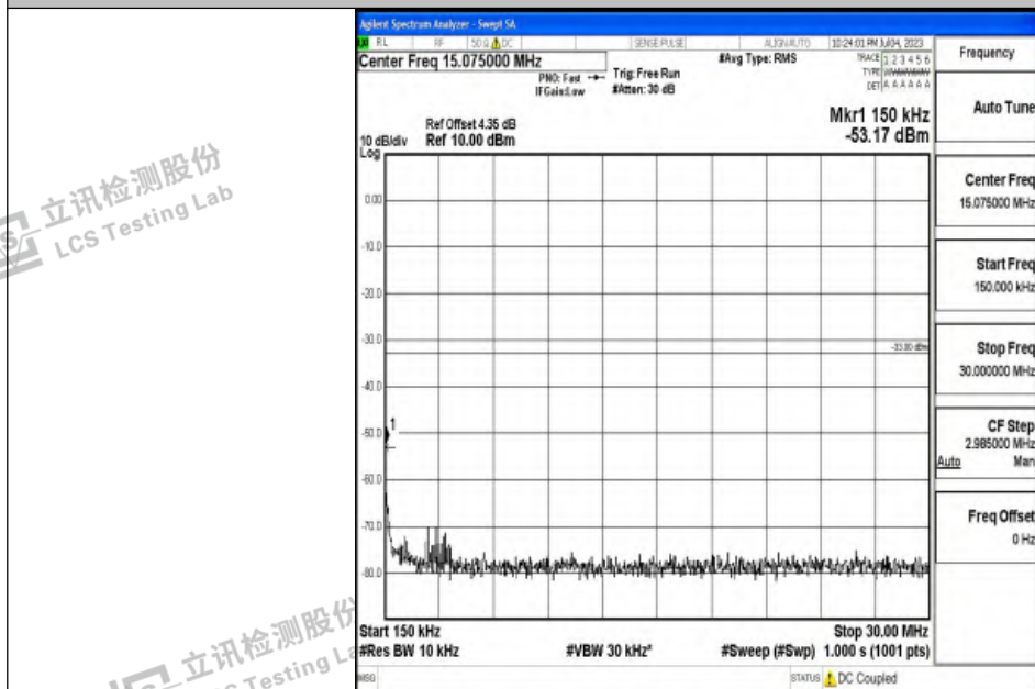
Band2_15MHz_16QAM_18900_1RB#0_0.15~30_0.15~30
