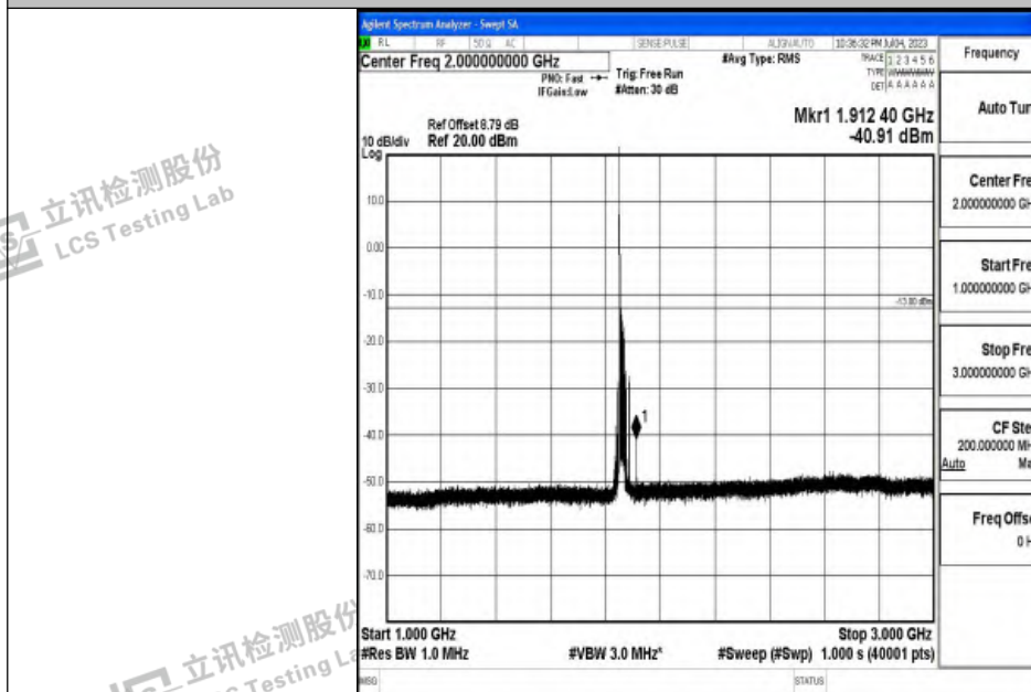
Band2_20MHz_16QAM_18700_1RB#0_1000~3000_1000~3000
