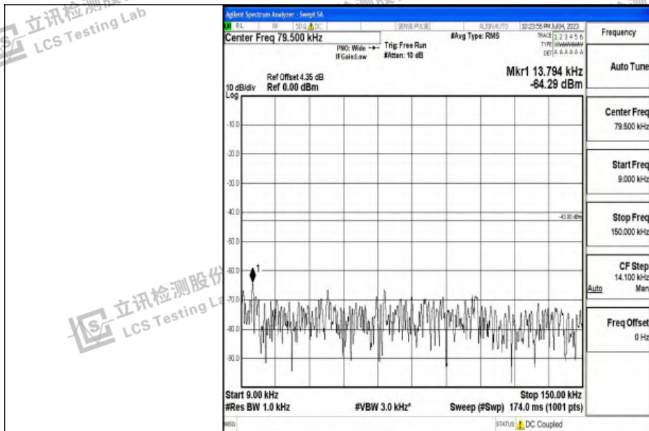
Band2_15MHz_16QAM_18900_1RB#0_0.009~0.15_0.009~0.15
