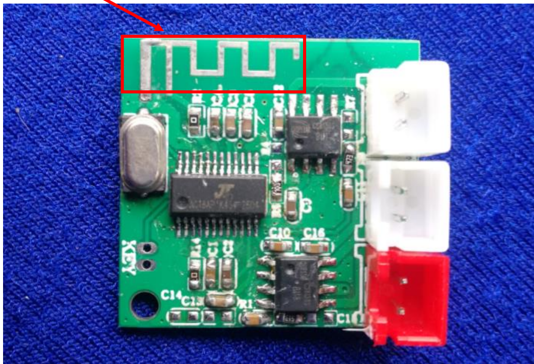
Bluetooth antenna
