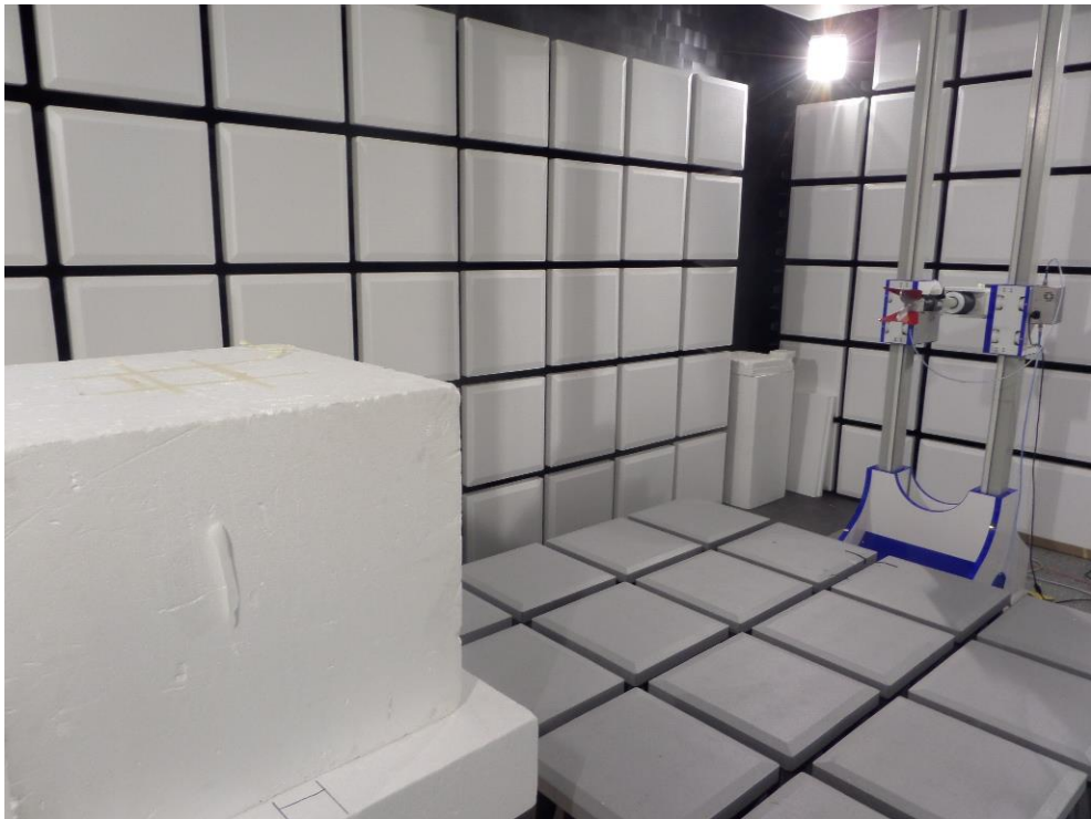
Anechoic chamber test site
