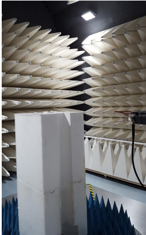
FigureC3. Radiated Setup – High Range
