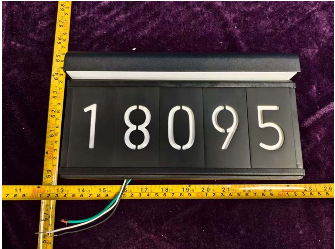
FIGURE 15 LED wall light (M/N: OUT-BOW5C-C1BL-DISPLAY) OUT-1
