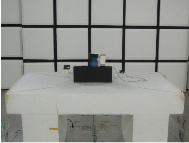
Radiated_Setup
