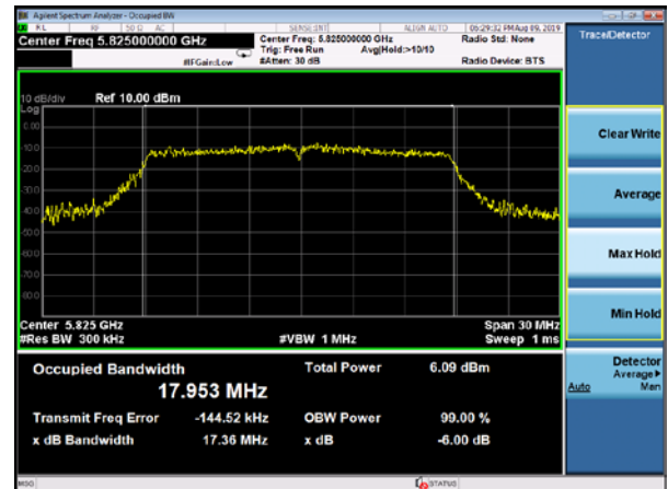
(802.11 AC20) 99%Bandwidth plot on channel 165
