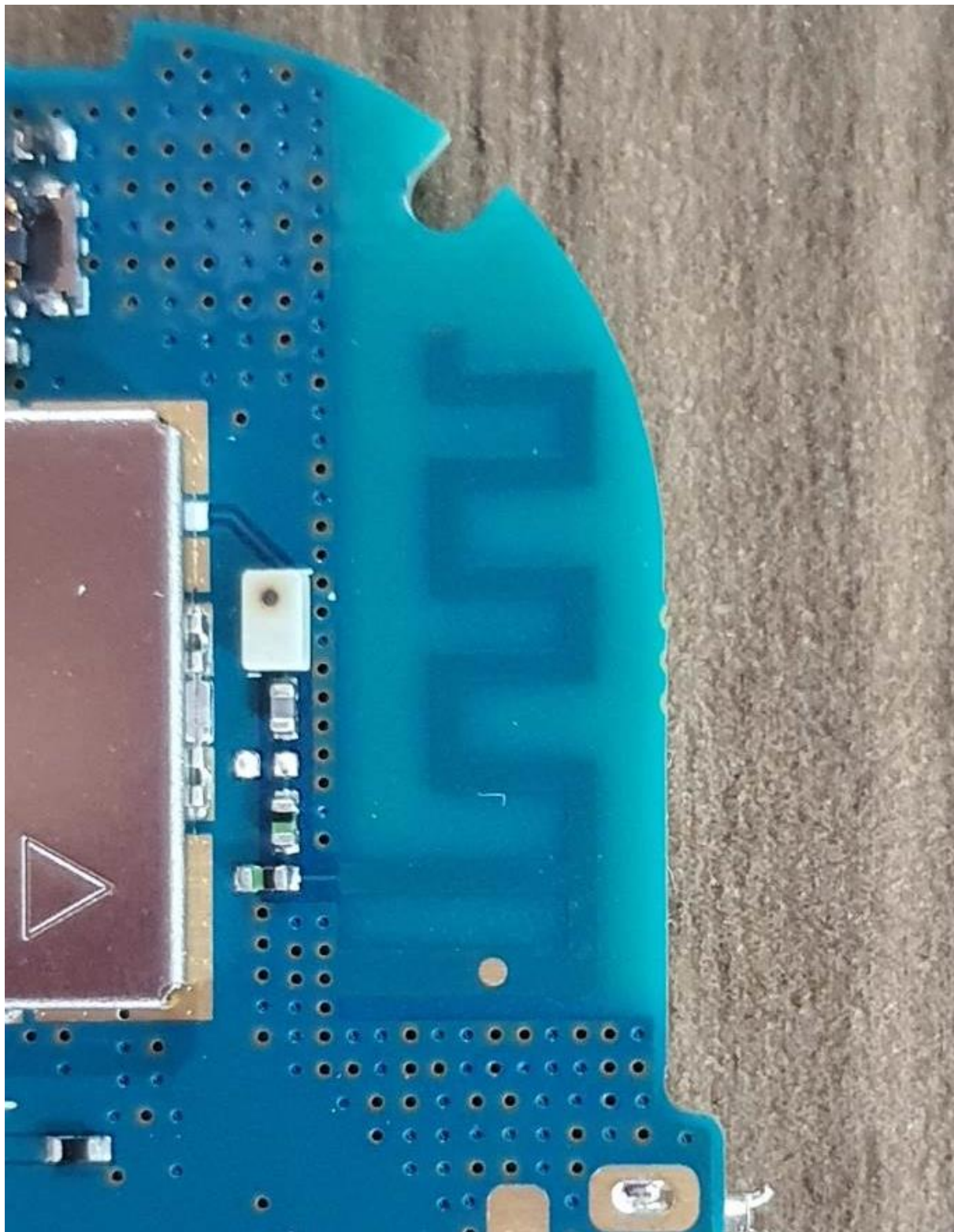
PCB Antenna
