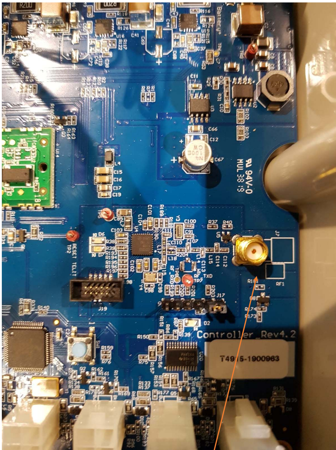
Transceiver module on card view. Antenna connector.
