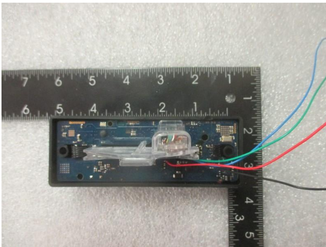
Figure 8.2 EUT Back Side, Size View (02)
