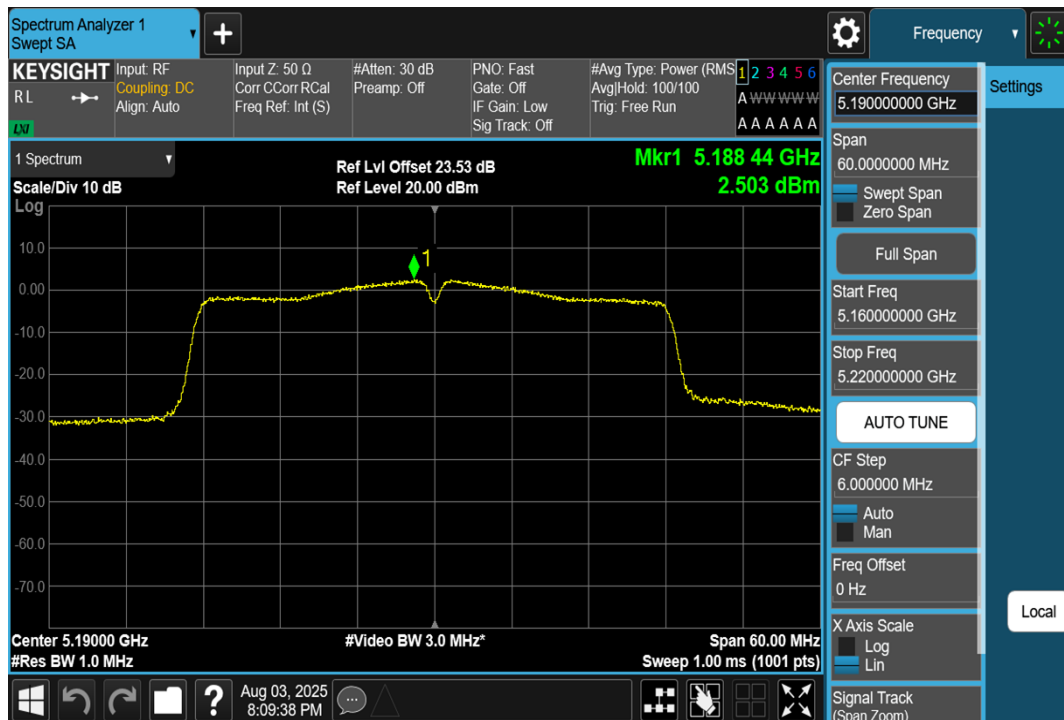
11N40SISO-Ant1-5190-PASS
