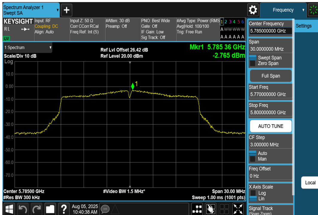
11N20SISO-Ant1-5785-PASS
