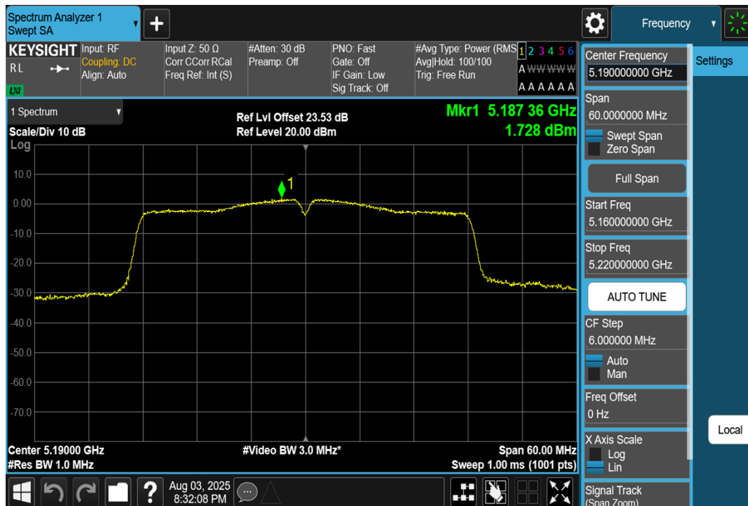
11AC40SISO-Ant1-5190-PASS
