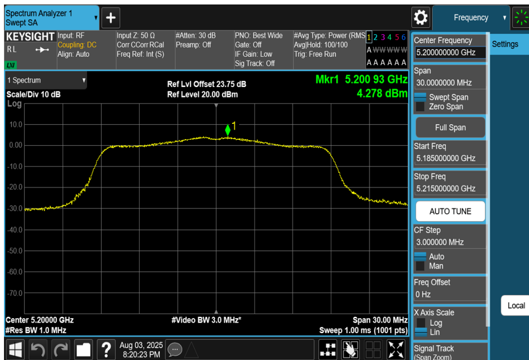
11AC20SISO-Ant1-5200-PASS
