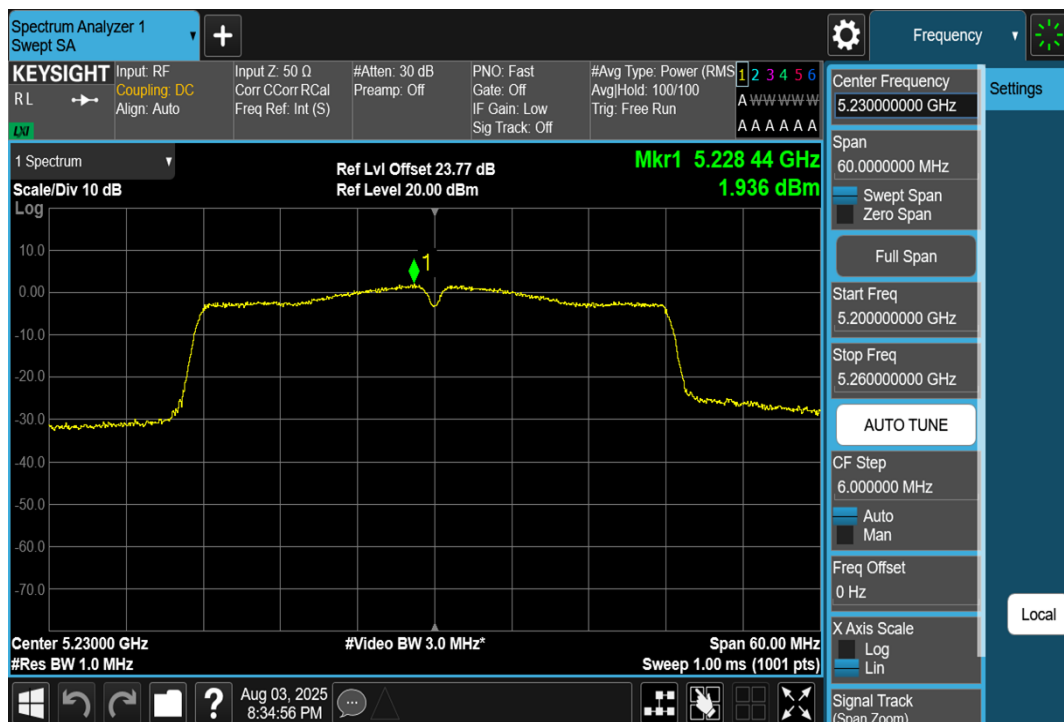
11AC40SISO-Ant1-5230-PASS
