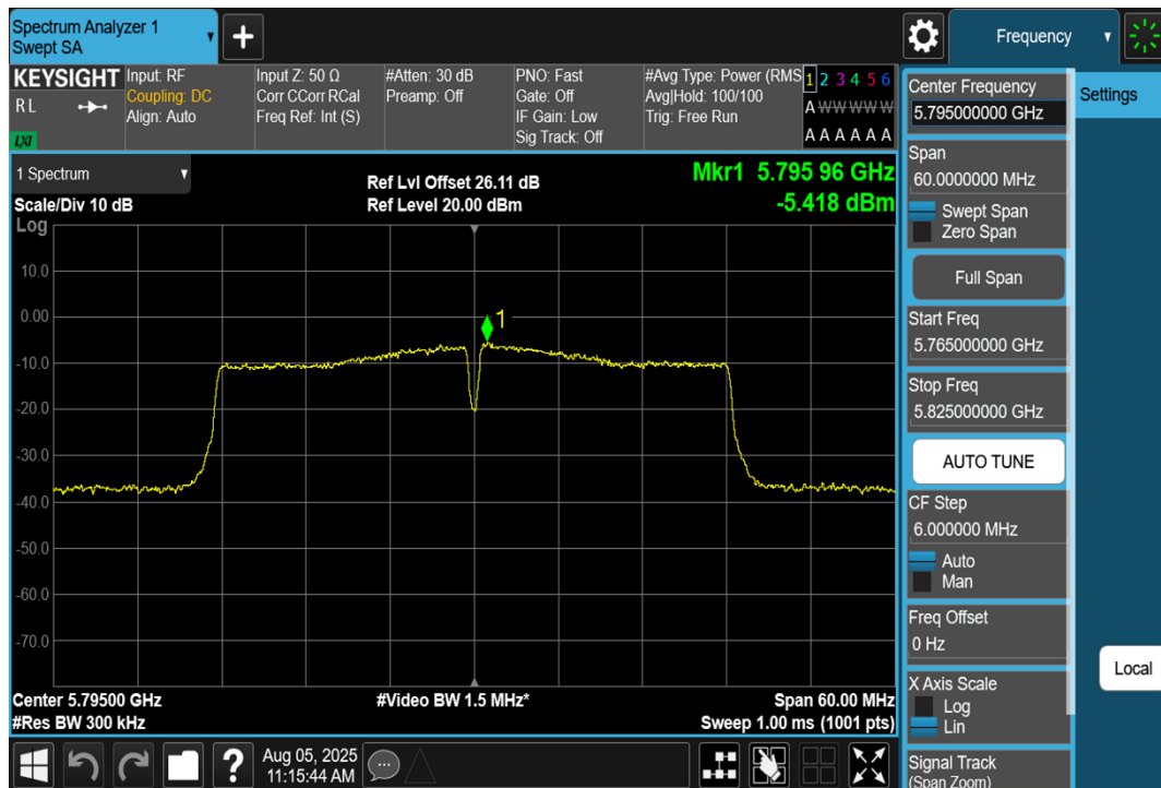
11AC40SISO-Ant1-5795-PASS
