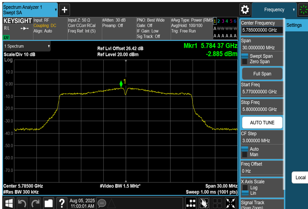
11AC20SISO-Ant1-5785-PASS
