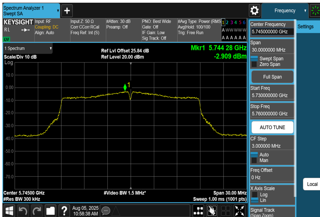
11AC20SISO-Ant1-5745-PASS
