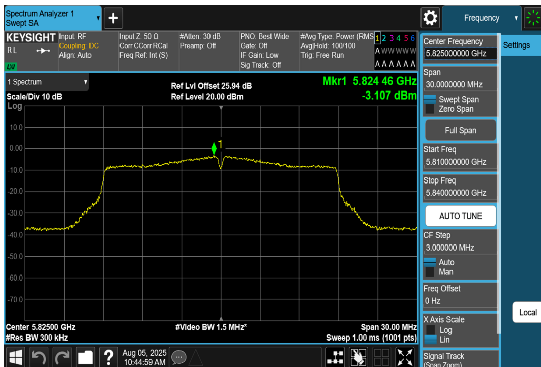
11N20SISO-Ant1-5825-PASS
