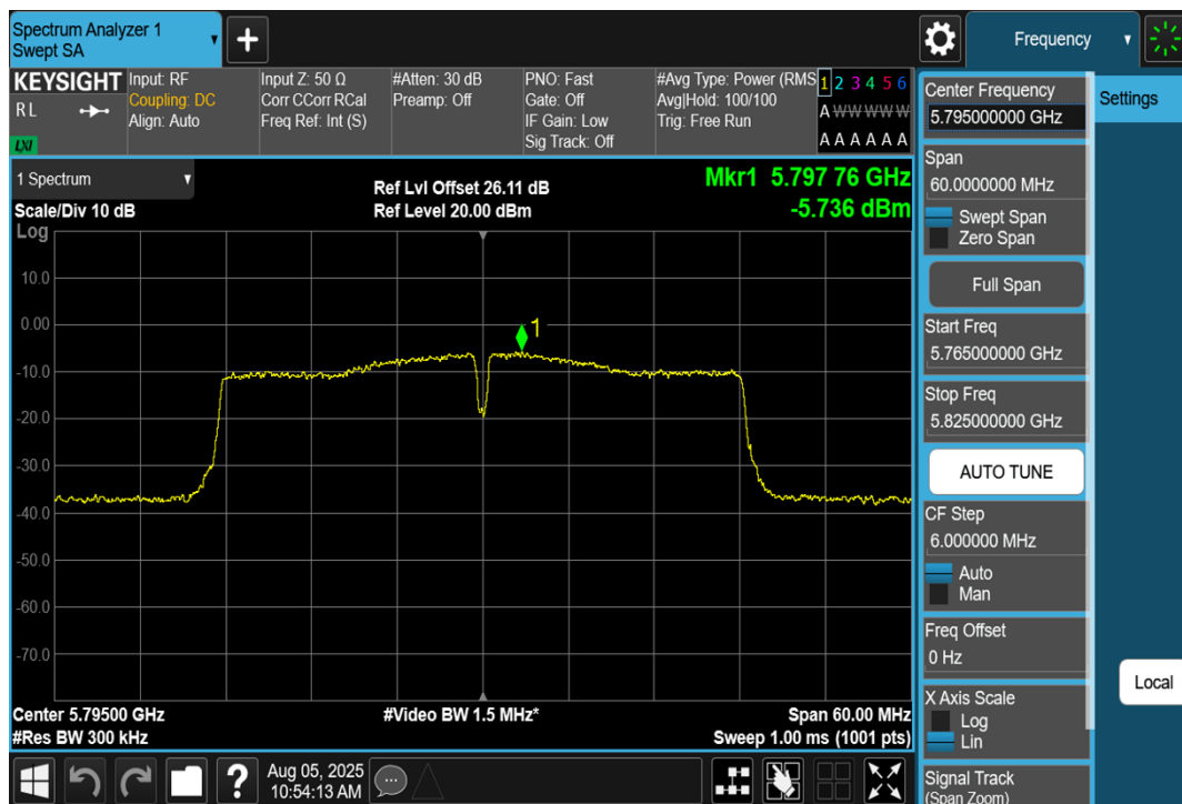
11N40SISO-Ant1-5795-PASS
