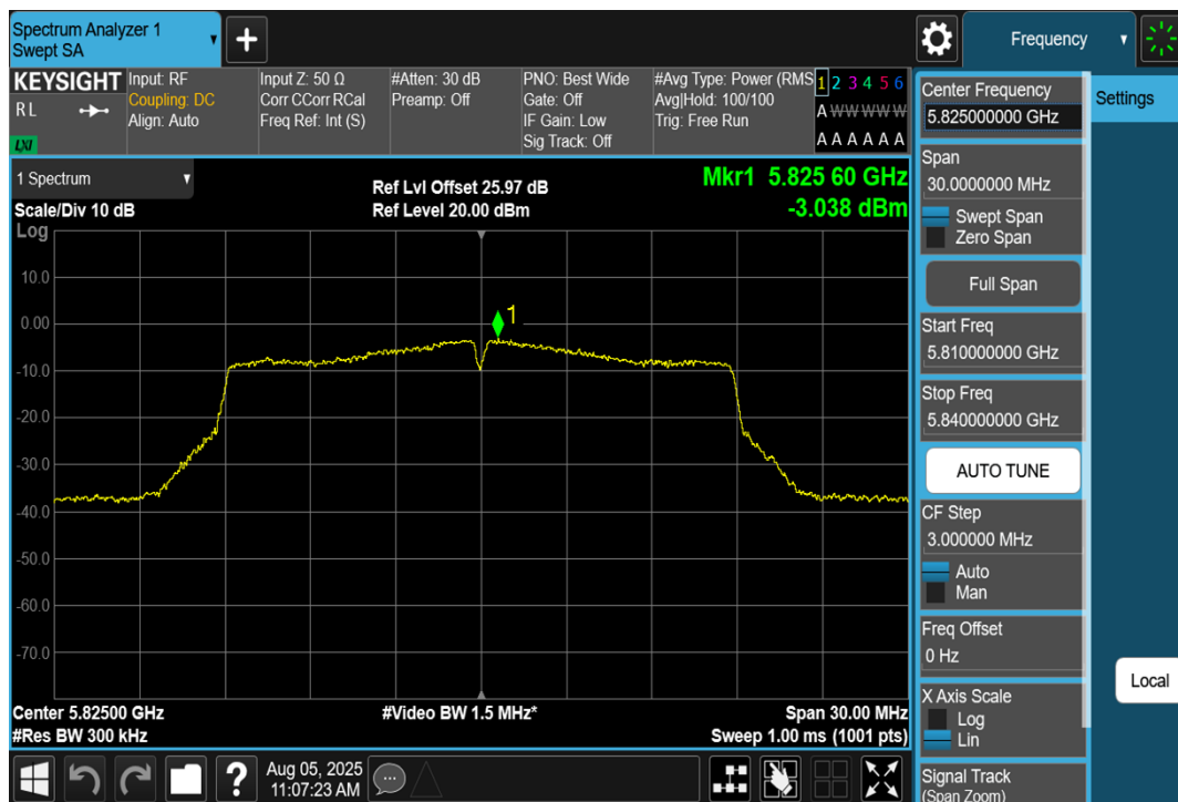
11AC20SISO-Ant1-5825-PASS
