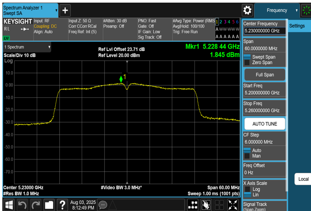
11N40SISO-Ant1-5230-PASS
