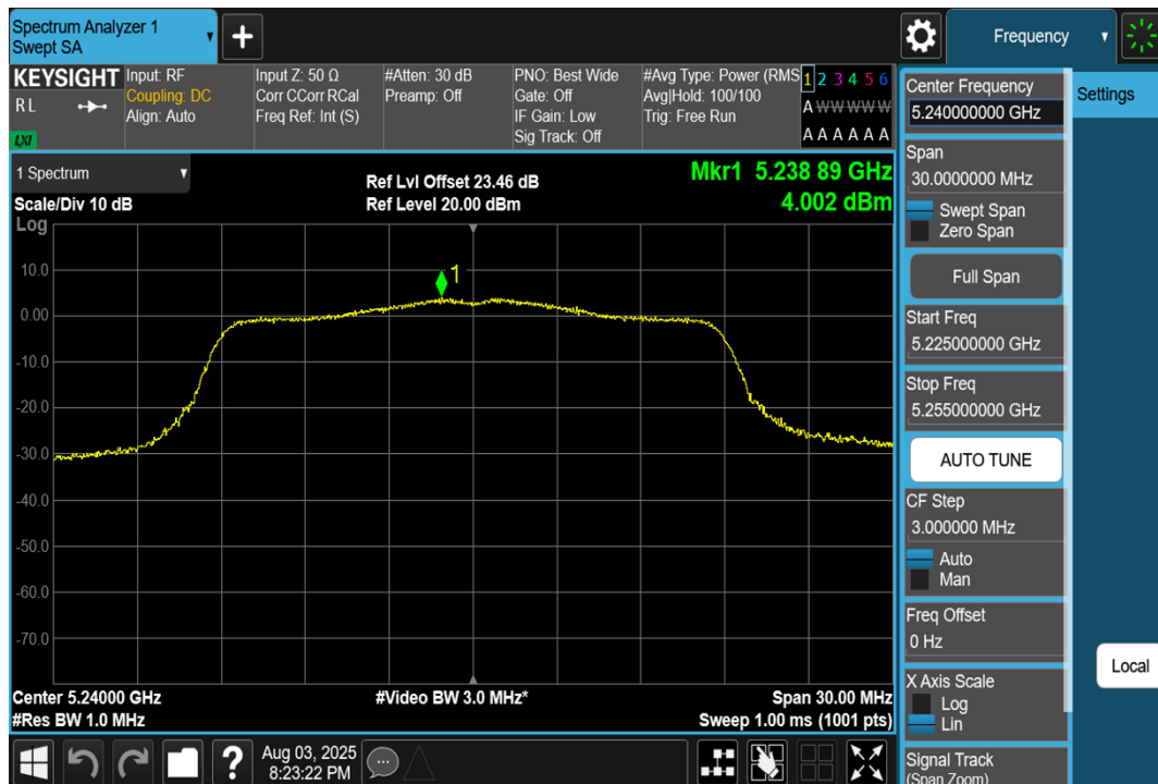
11AC20SISO-Ant1-5240-PASS
