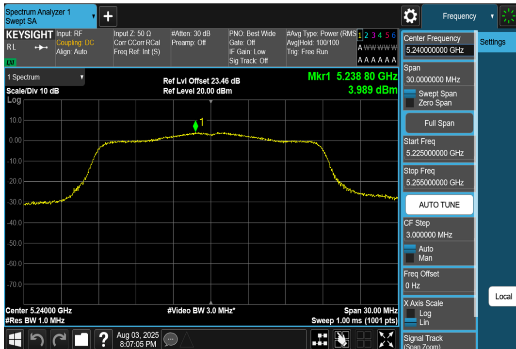
11N20SISO-Ant1-5240-PASS
