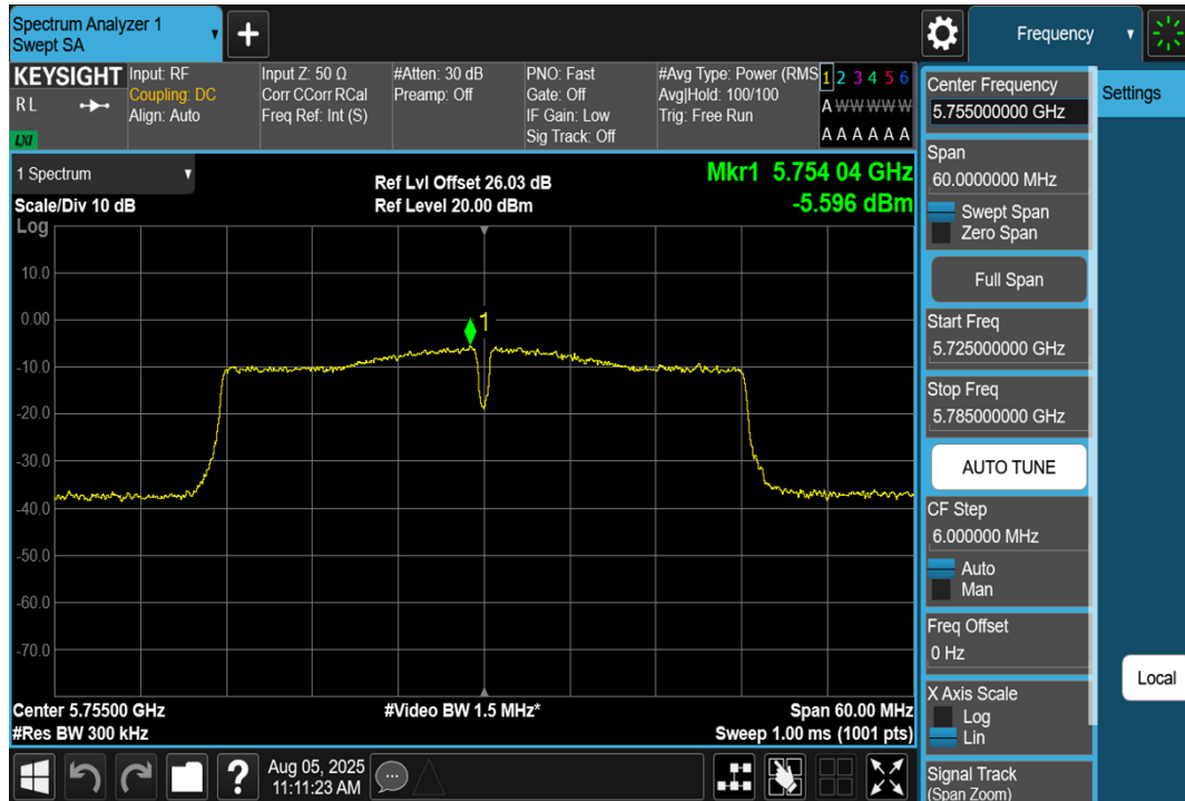
11AC40SISO-Ant1-5755-PASS
