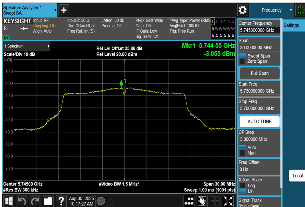
11A-Ant1-5745-PASS
