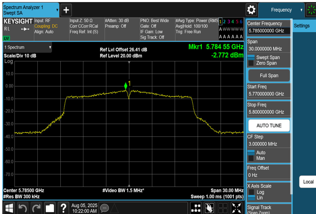
11A-Ant1-5785-PASS
