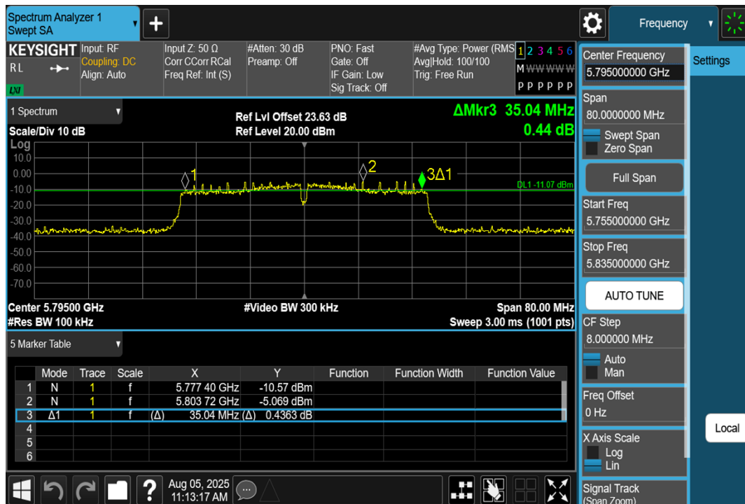
11AC40SISO-Ant1-5795-PASS
