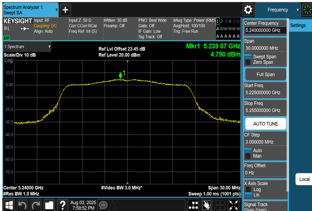
11A-Ant1-5240-PASS
