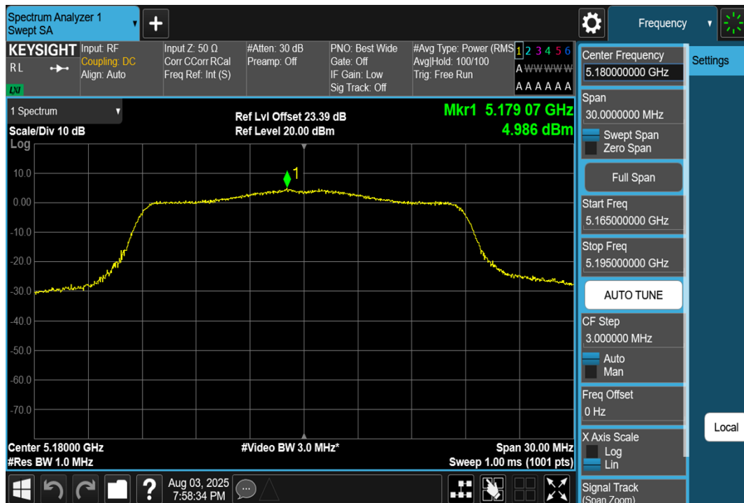
11N20SISO-Ant1-5180-PASS
