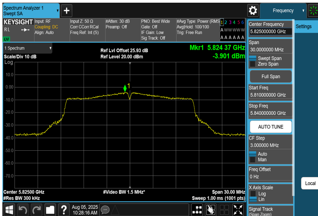
11A-Ant1-5825-PASS
