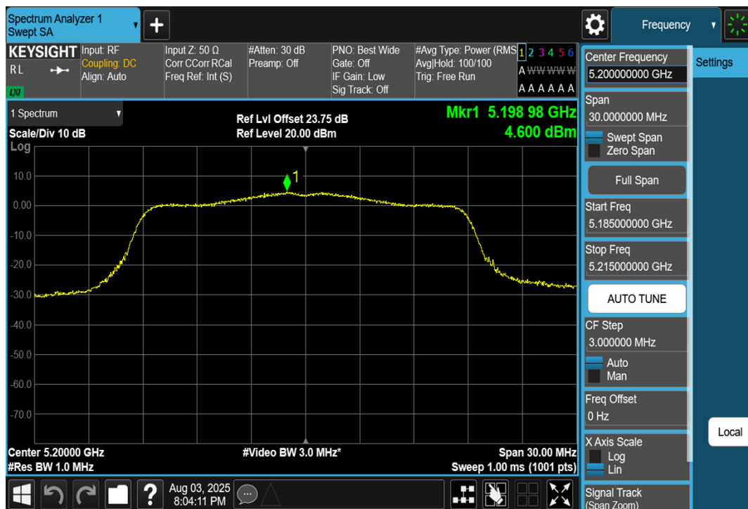
11N20SISO-Ant1-5200-PASS
