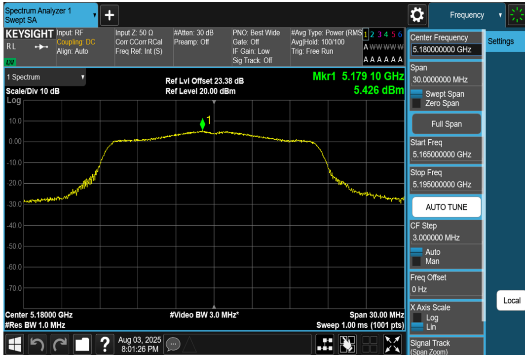
11A-Ant1-5180-PASS
