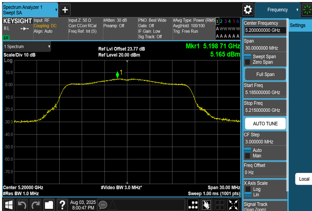
11A-Ant1-5200-PASS
