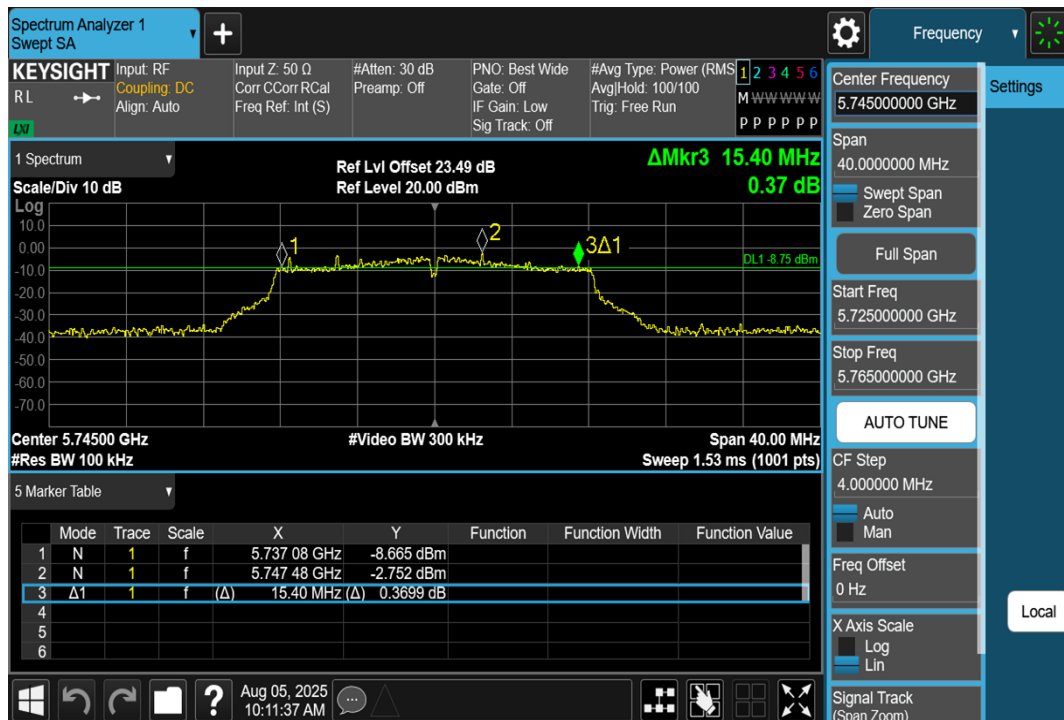
11A-Ant1-5745-PASS
