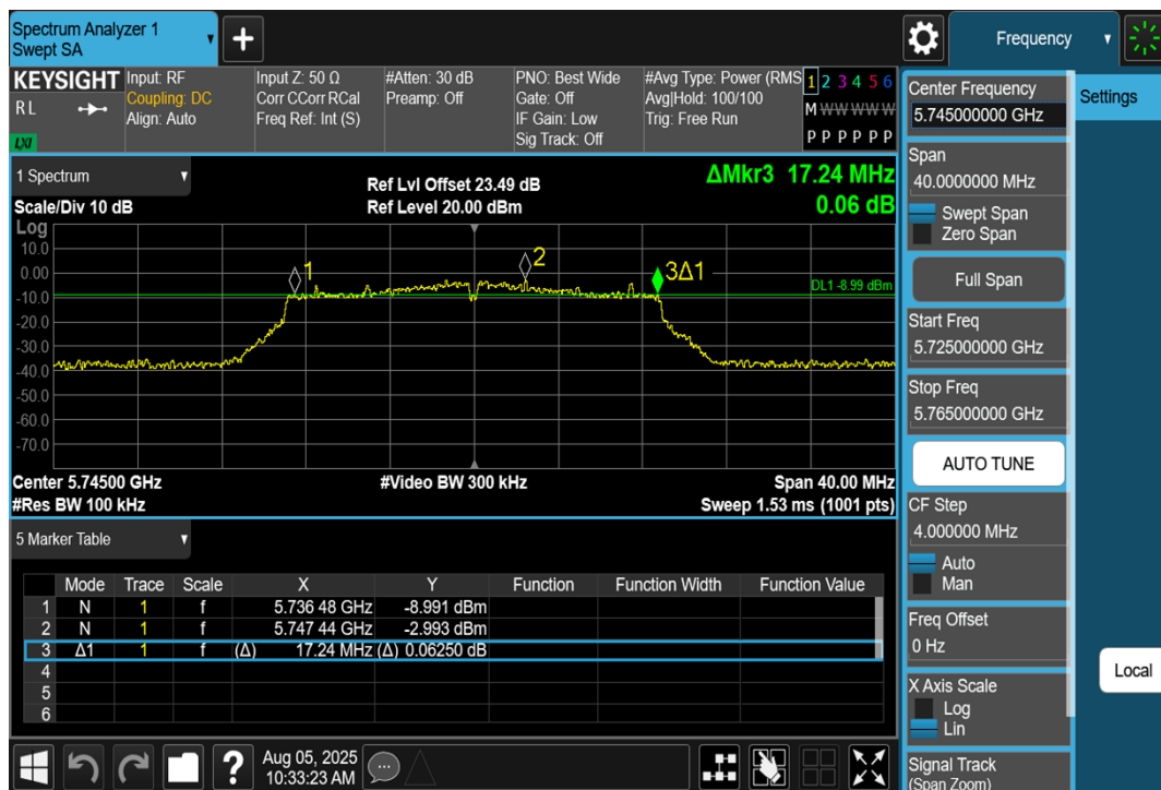
11N20SISO-Ant1-5745-PASS
