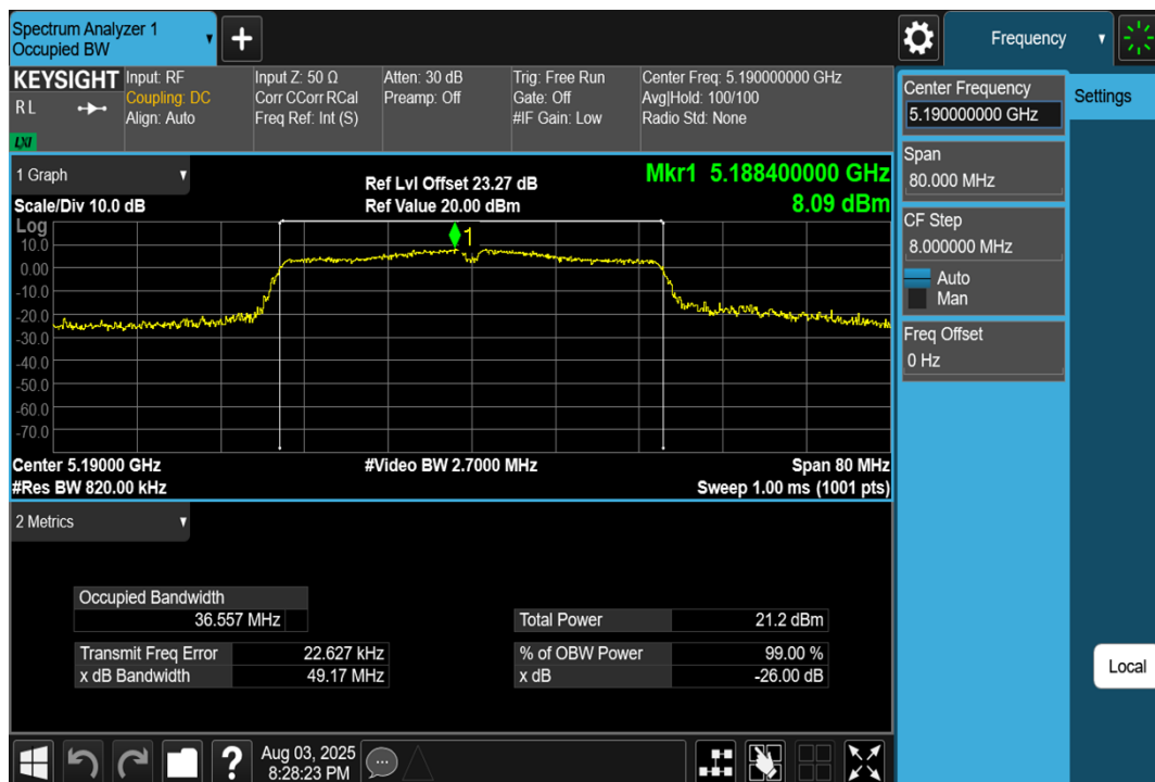
11AC40SISO-Ant1-5190
