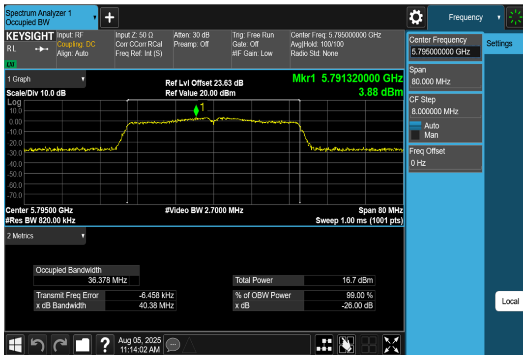
11AC40SISO-Ant1-5795
