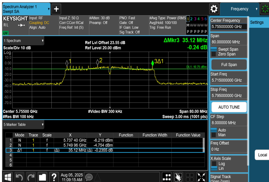
11AC40SISO-Ant1-5755-PASS
