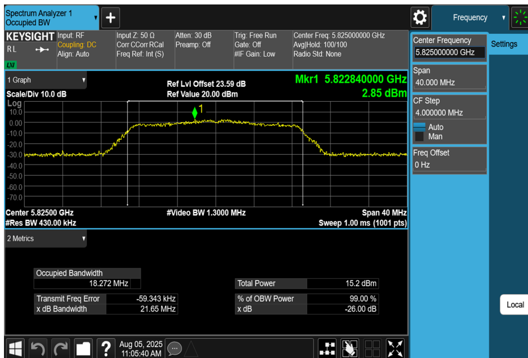
11AC20SISO-Ant1-5825
