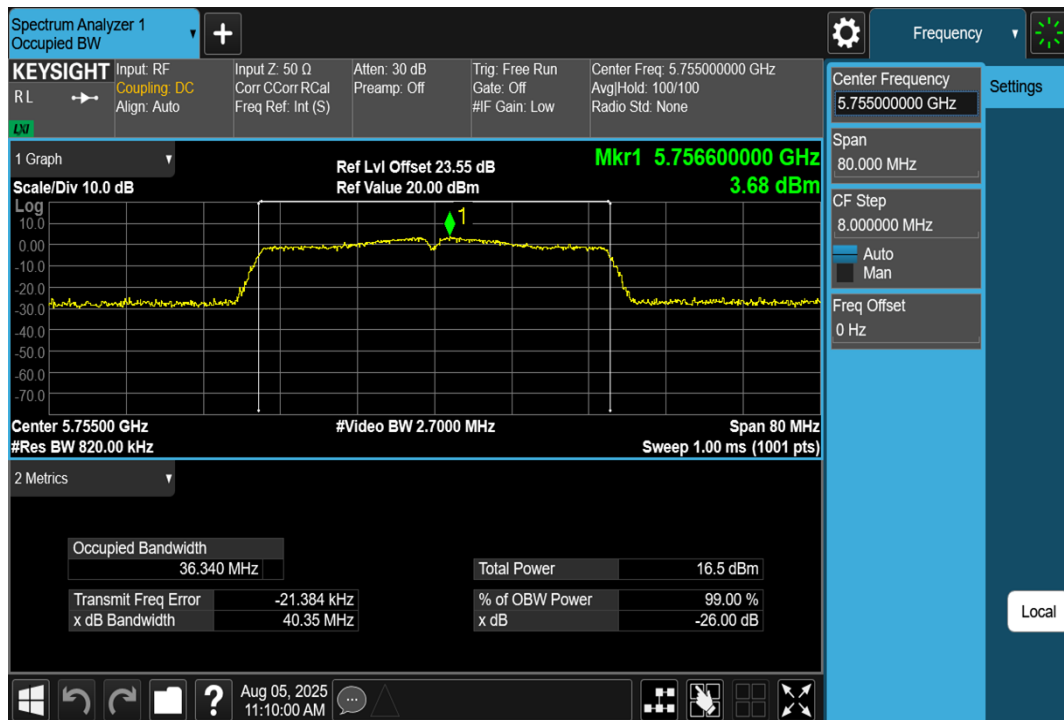
11AC40SISO-Ant1-5755
