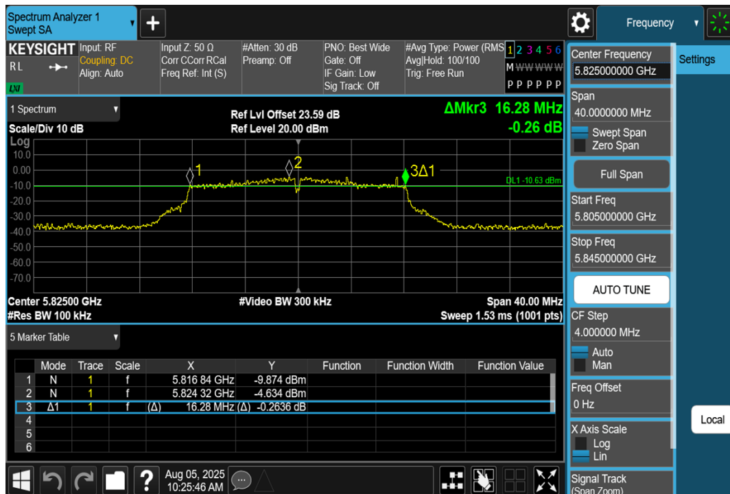
11A-Ant1-5825-PASS
