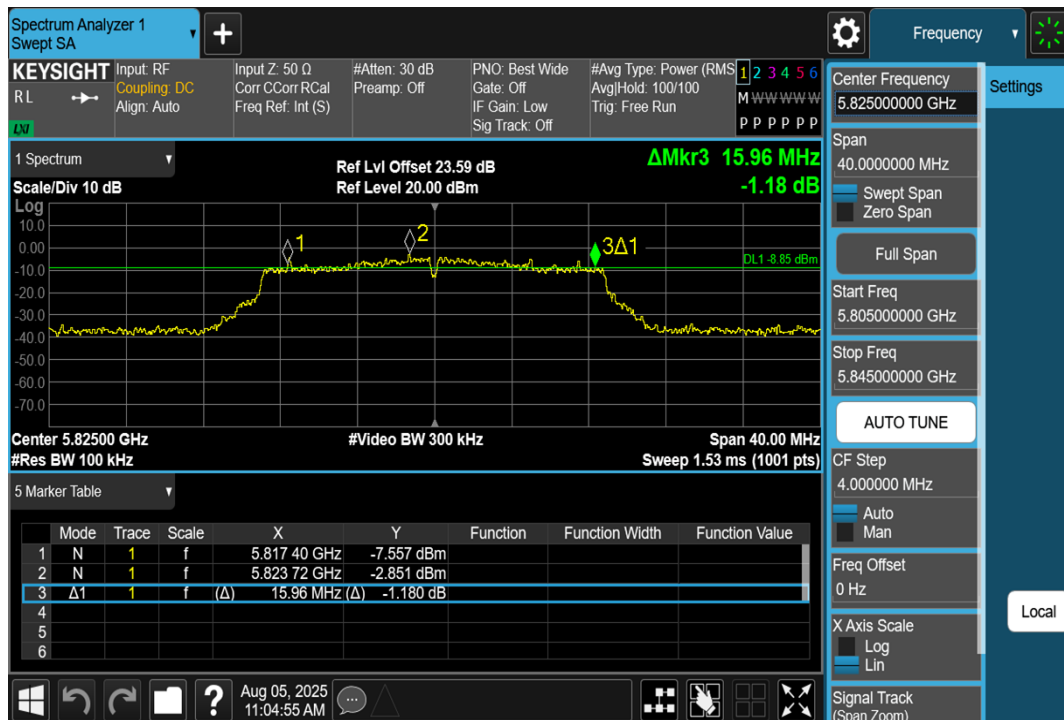
11AC20SISO-Ant1-5825-PASS
