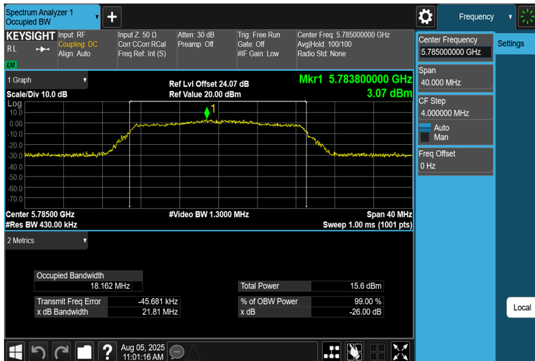
11AC20SISO-Ant1-5785
