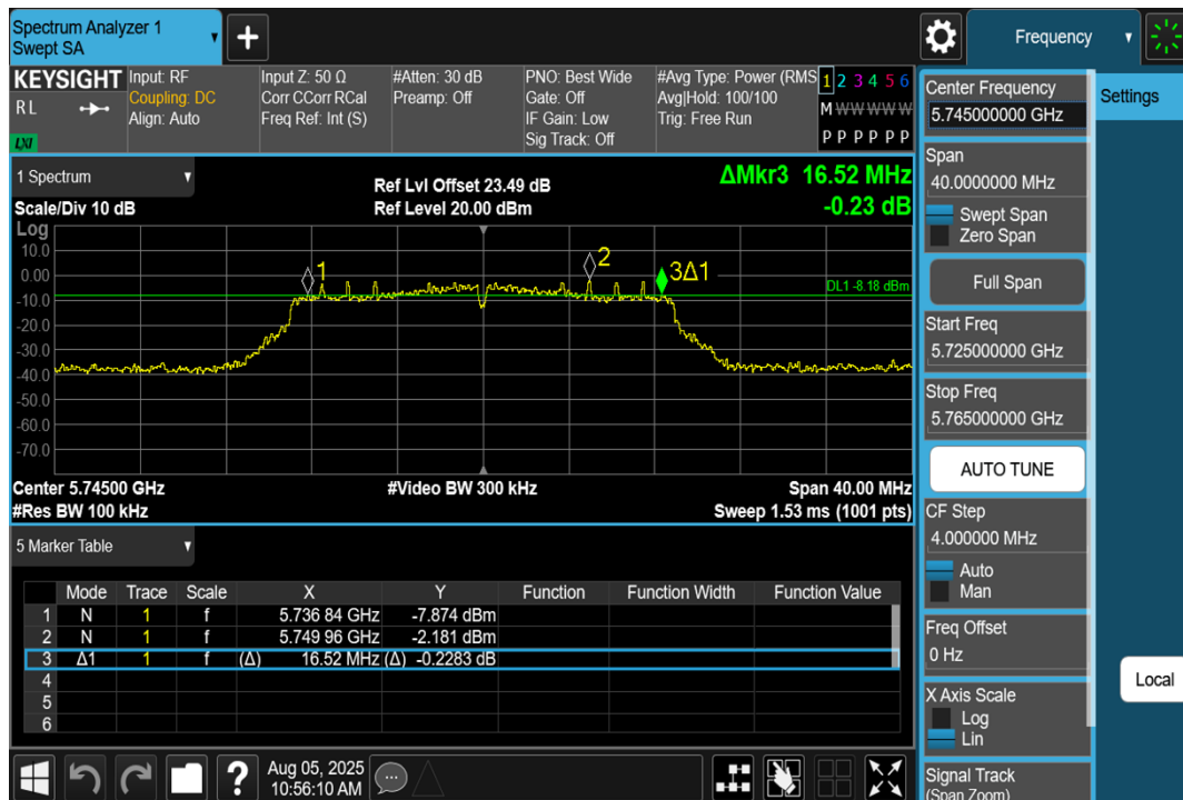
11AC20SISO-Ant1-5745-PASS
