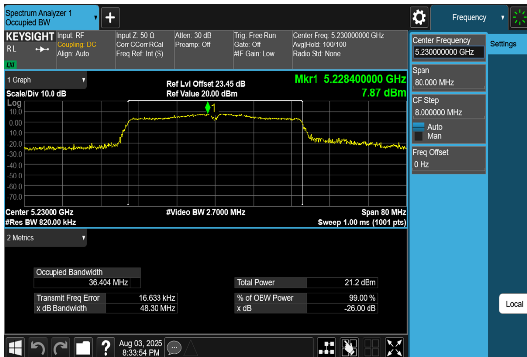
11AC40SISO-Ant1-5230
