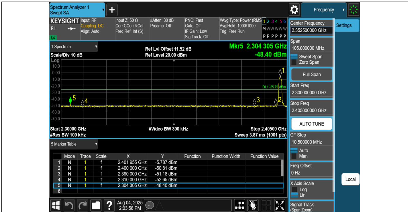
2DH5-Ant1-2402-PASS
