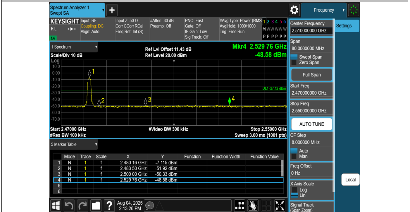
3DH5-Ant1-2480-PASS
