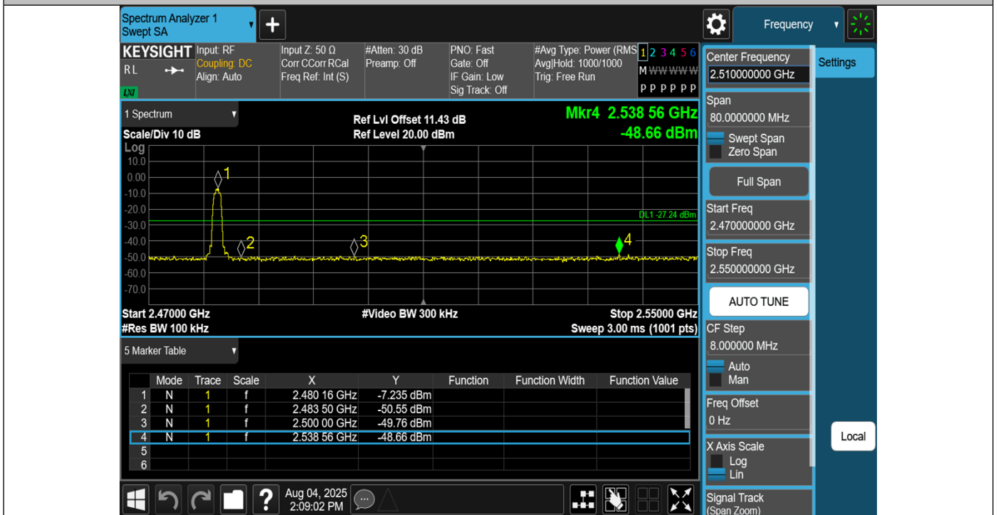
2DH5-Ant1-2480-PASS
