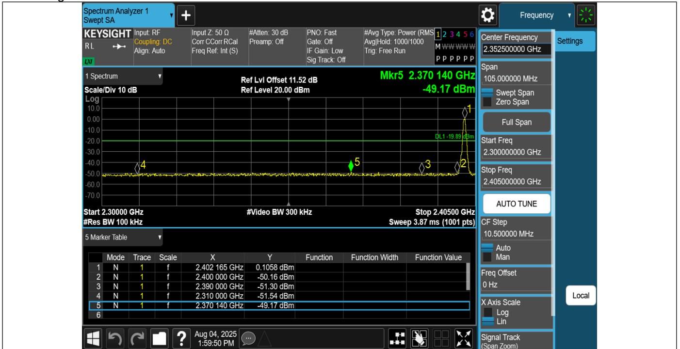
DH5-Ant1-2402-PASS
