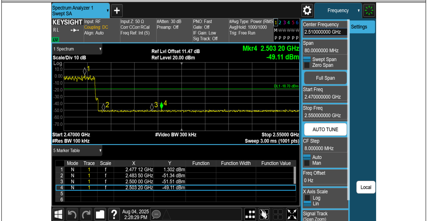
3DH5-Ant1-Hop_2480-PASS
