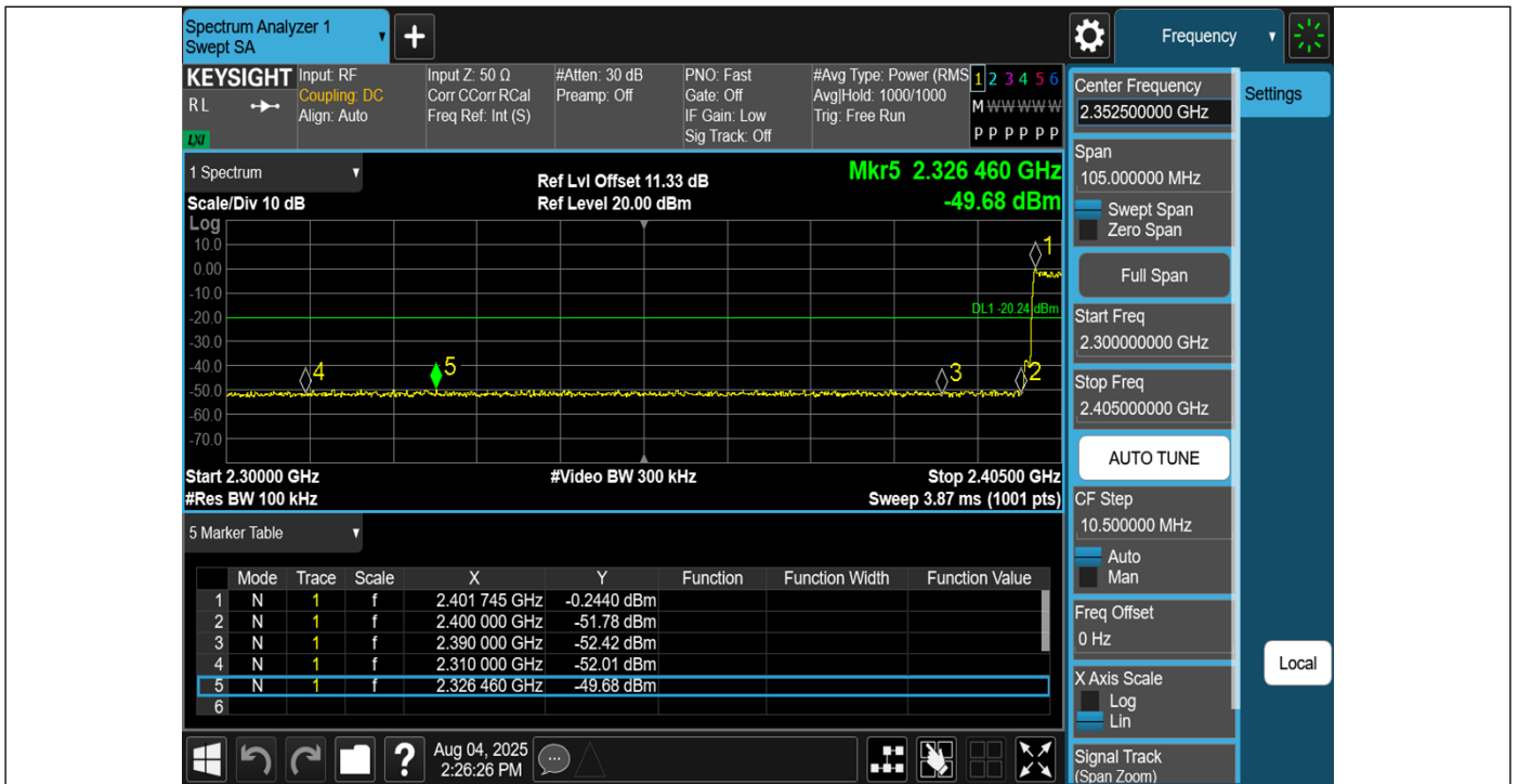
3DH5-Ant1-Hop_2402-PASS
