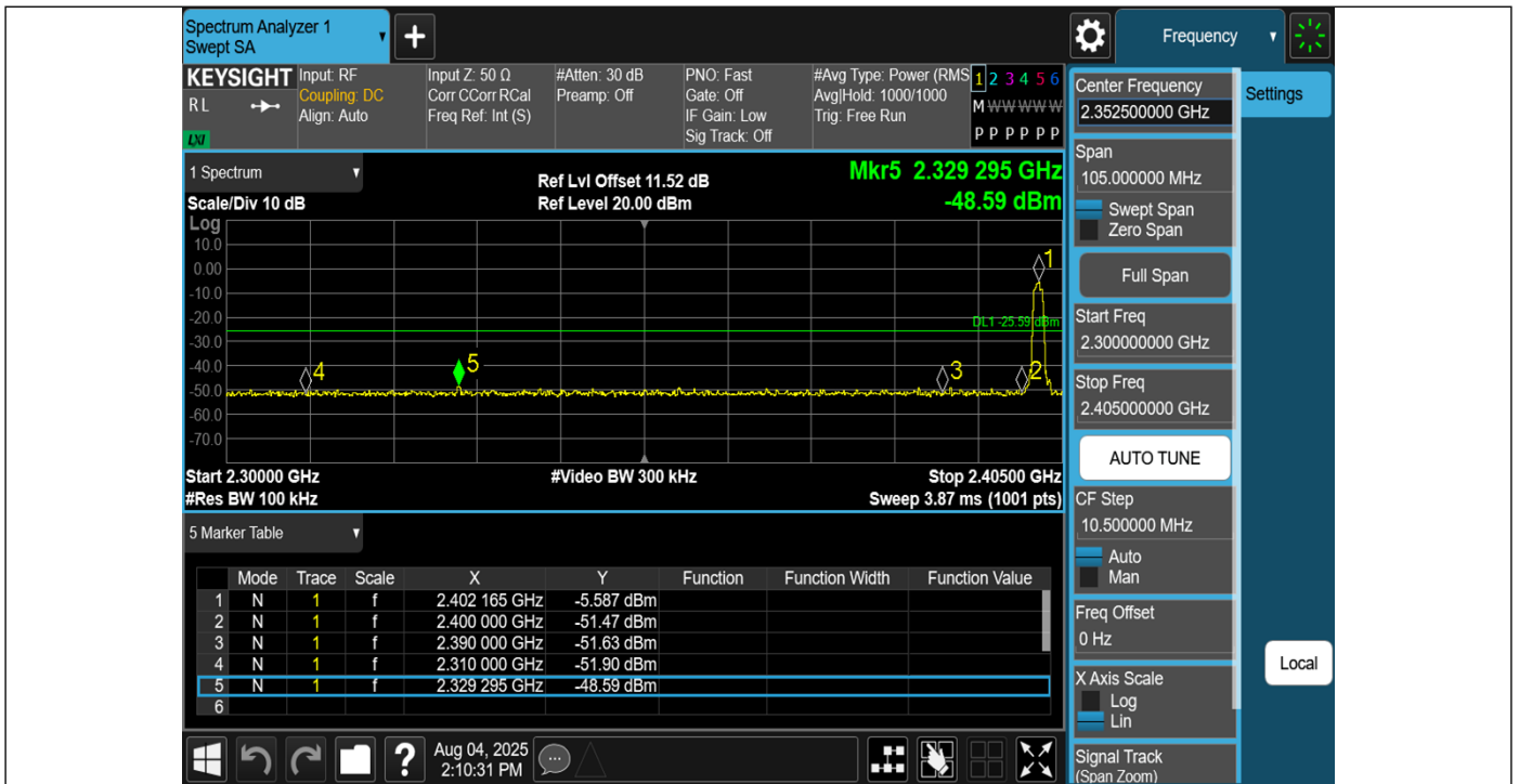
3DH5-Ant1-2402-PASS
