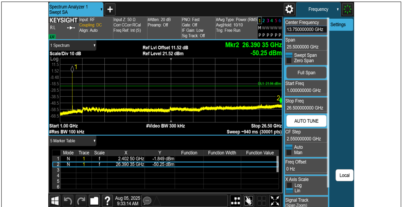
3DH5-Ant1-2402-1000~26500-PASS
