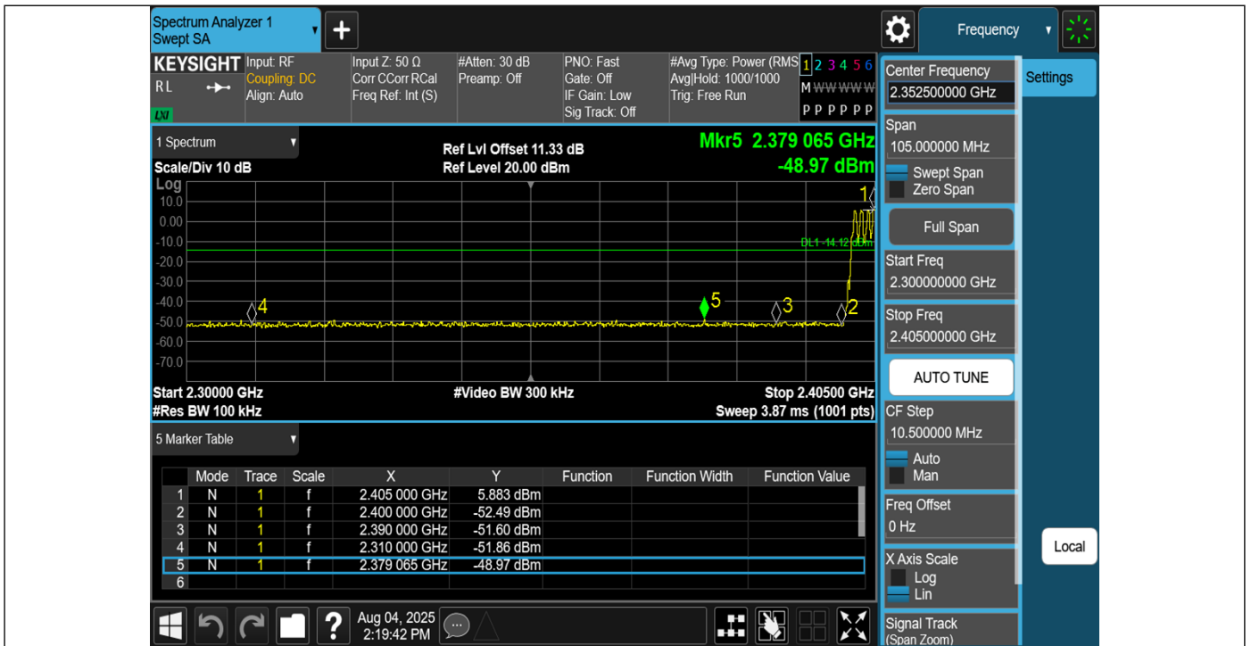
DH5-Ant1-Hop_2402-PASS
