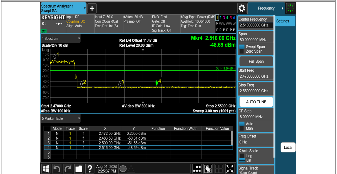
2DH5-Ant1-Hop_2480-PASS
