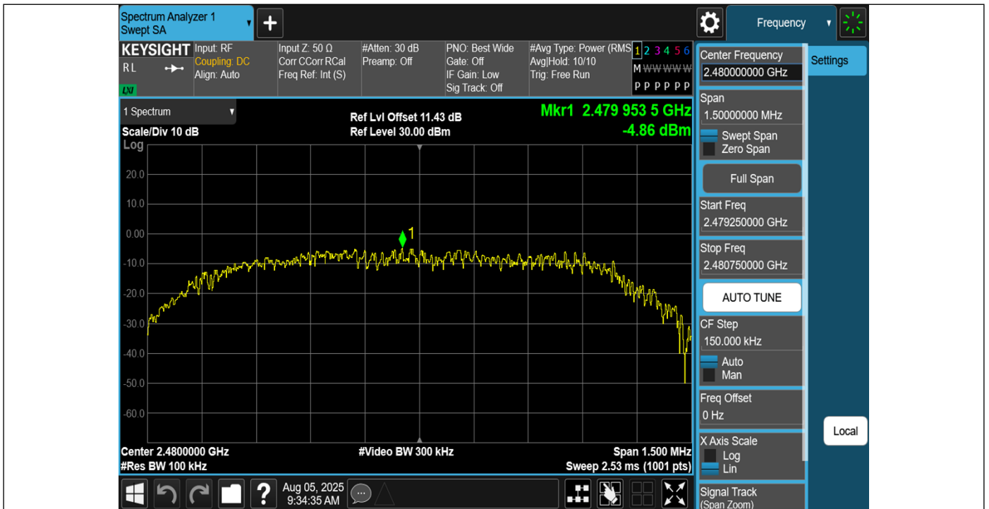
3DH5-Ant1-2480-0~Reference-PASS
