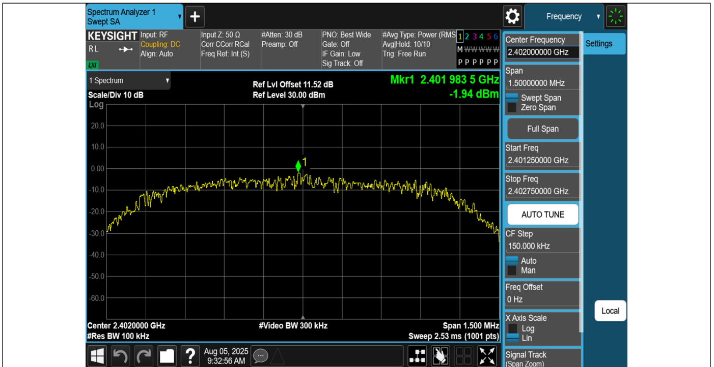
3DH5-Ant1-2402-0~Reference-PASS
