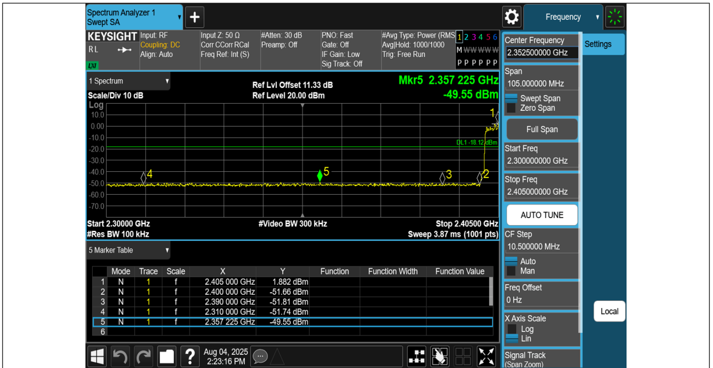
2DH5-Ant1-Hop_2402-PASS
