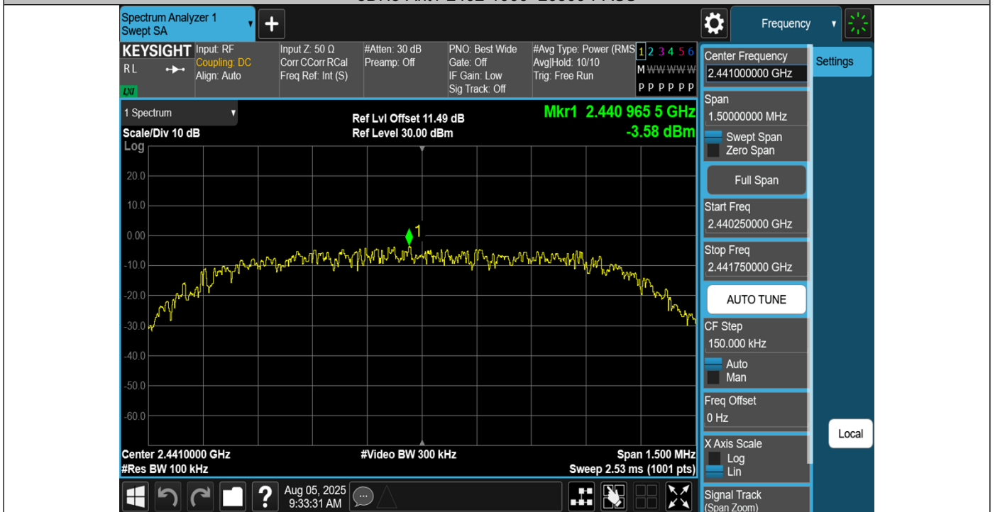
3DH5-Ant1-2441-0~Reference-PASS
