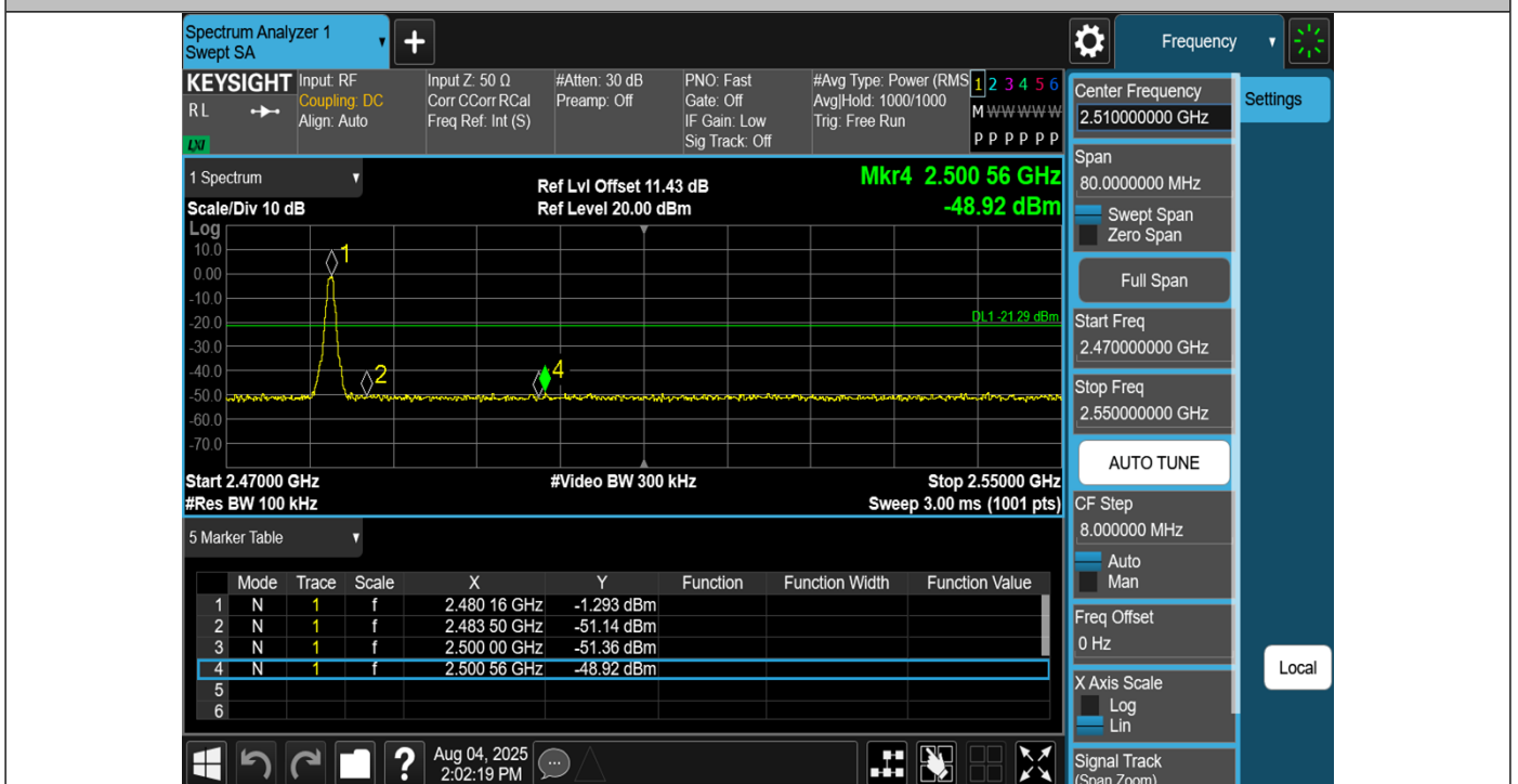
DH5-Ant1-2480-PASS
