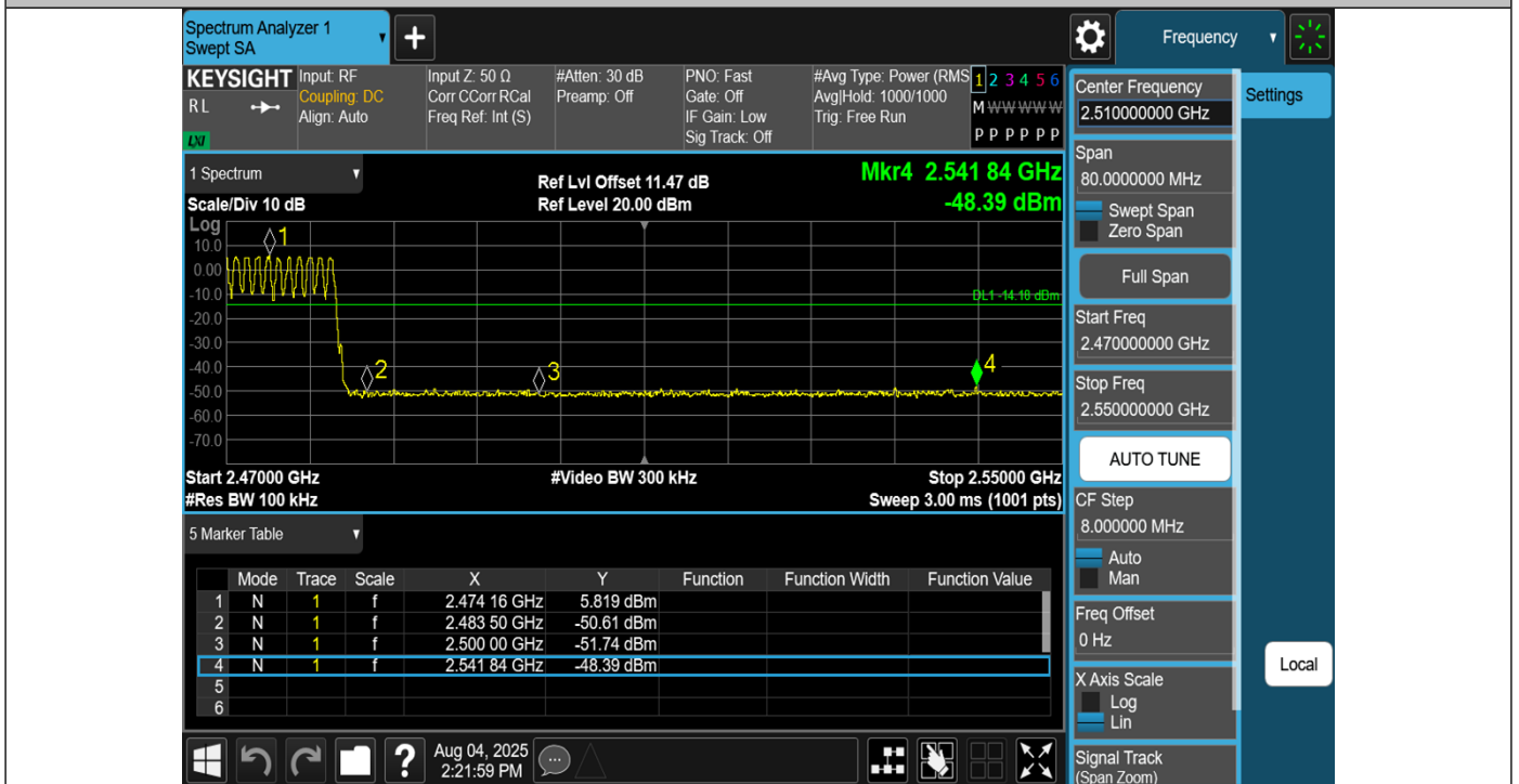
DH5-Ant1-Hop_2480-PASS
