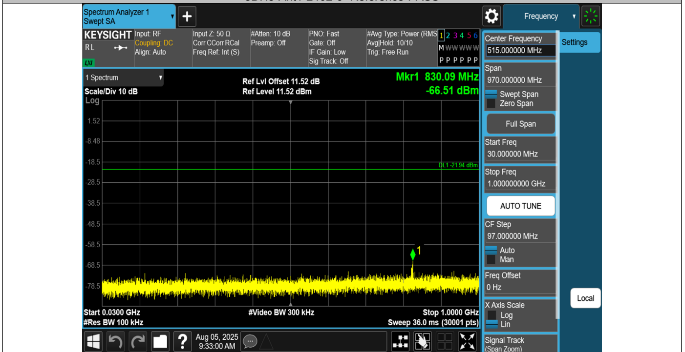
3DH5-Ant1-2402-30~1000-PASS
