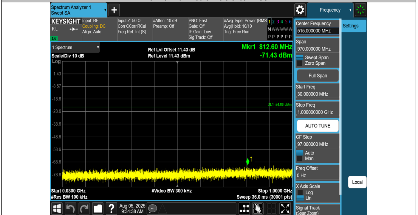
3DH5-Ant1-2480-30~1000-PASS
