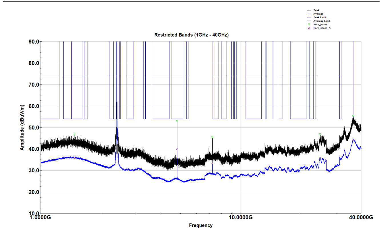
Figure 14. Low Channel, 1GHz – 40GHz Restricted Band Spurious Emissions
