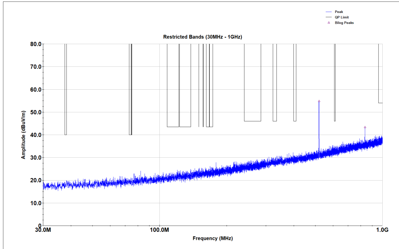
Figure 19. High Channel, 30MHz – 1GHz Restricted Band Spurious Emissions
