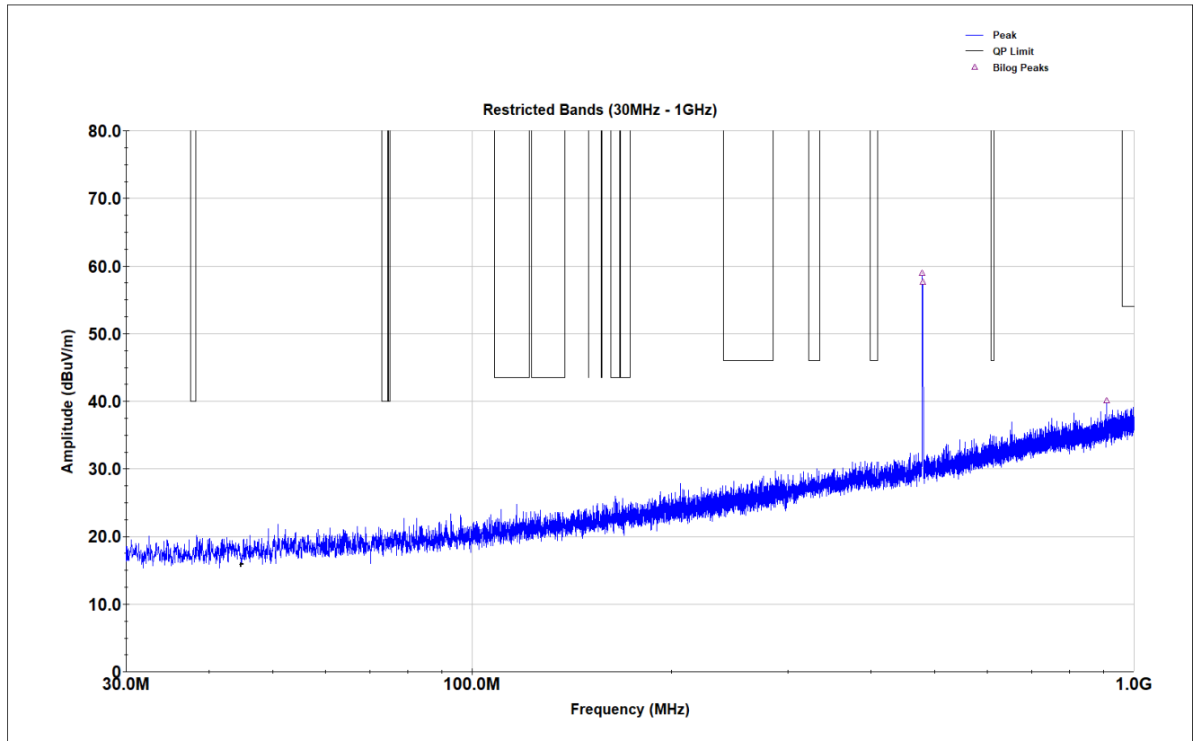
Figure 16. Middle Channel, 30MHz – 1GHz Restricted Band Spurious Emissions
