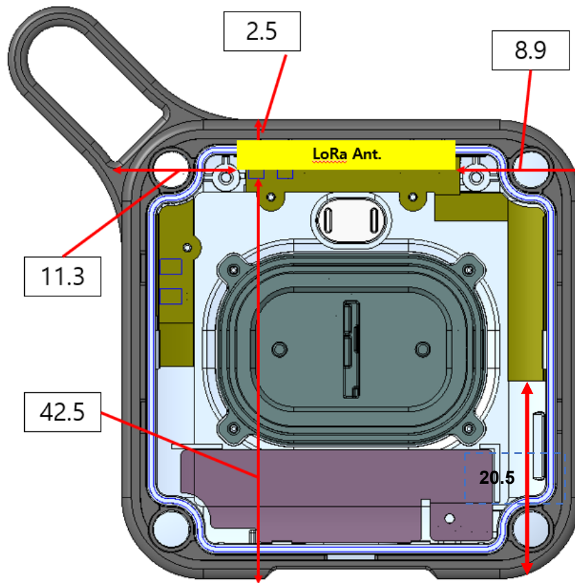
Figure F-1 Antenna Location for LoRa – Rear Side View
