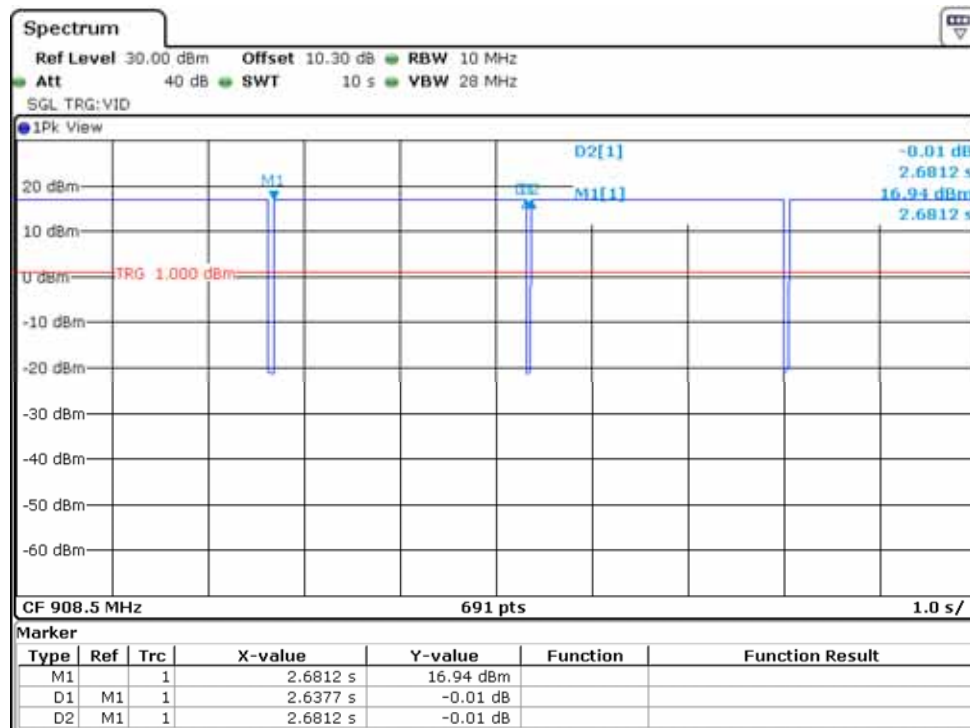
Figure 8-1 LoRa 125 KHz Transmission Plot
