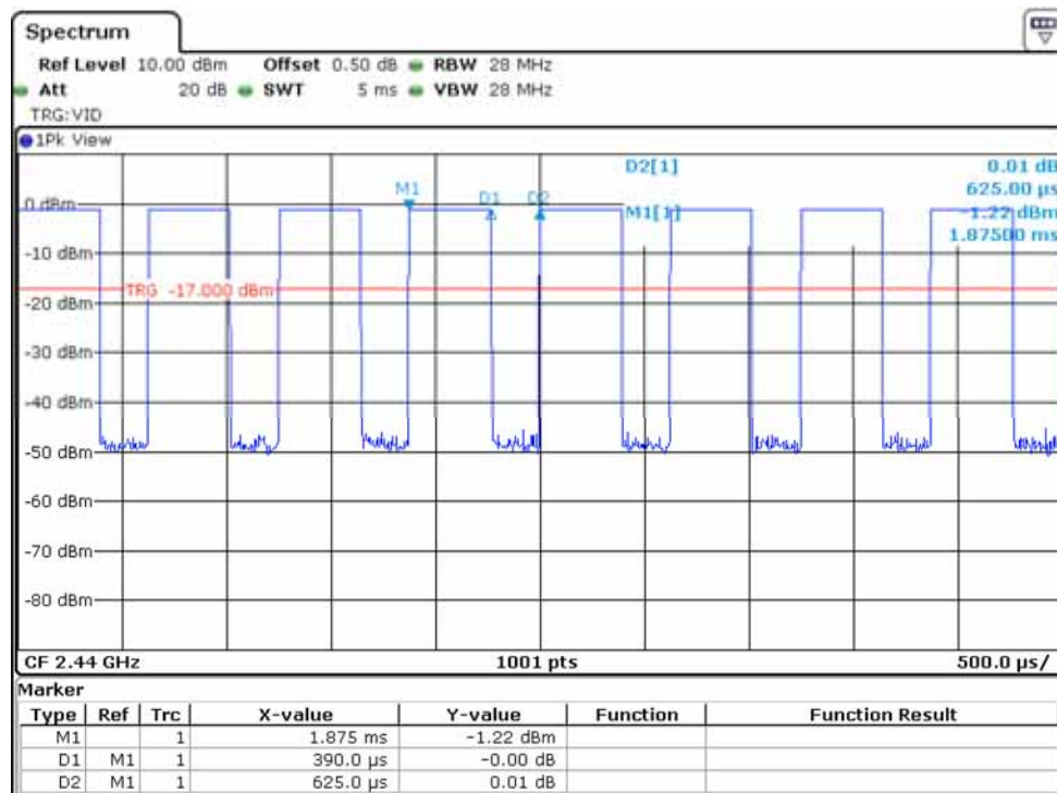
Figure 8-3 Bluetooth LE Transmission Plot
