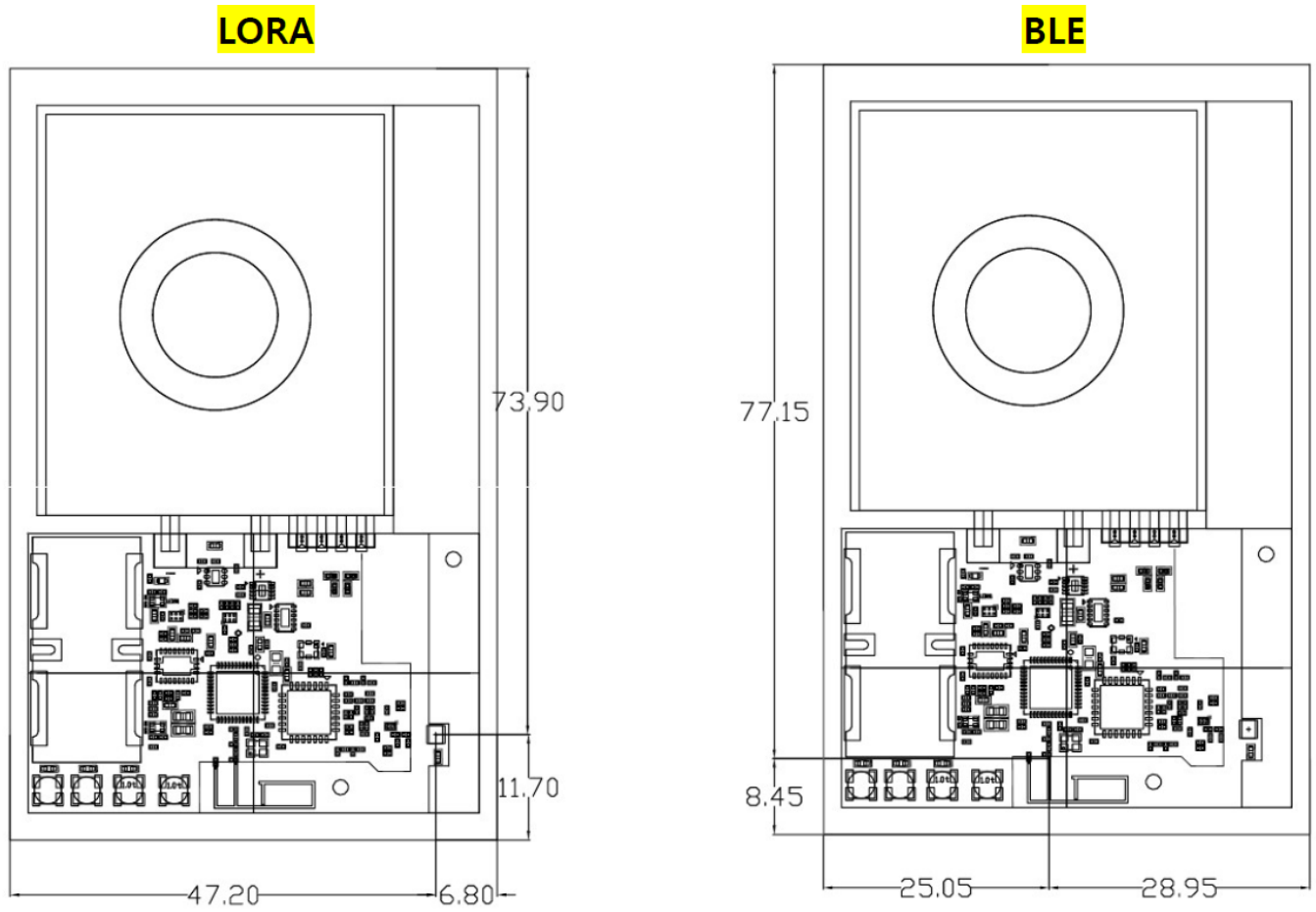
Figure F-1 Antenna Location
