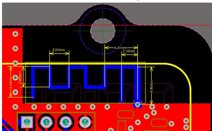
Antenna Photo & Length (mm)
