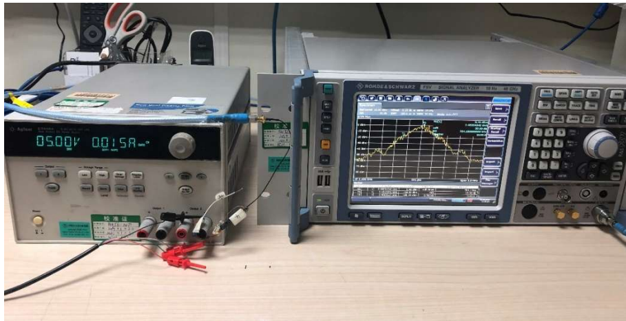
RF Conducted Test Setup
