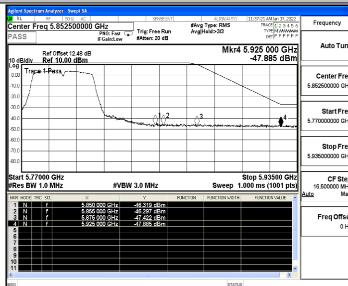
11AC40SISO_Ant_High_5795_Peak
