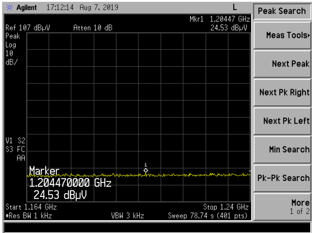
Figure 6. Band 1164 - 1240 MHz (Vertical- worst case)
