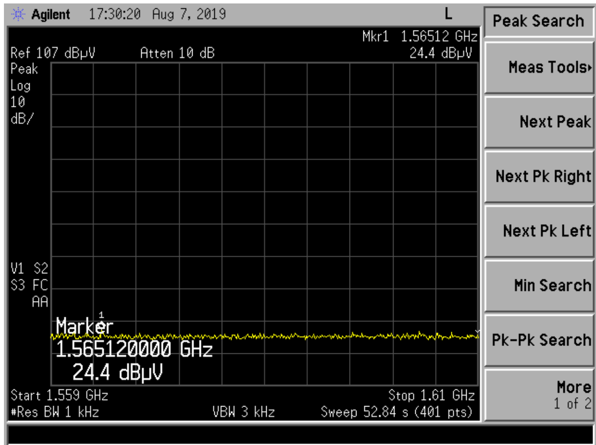
Figure 7. Band 1559 - 1610 MHz (Vertical- worst case)
