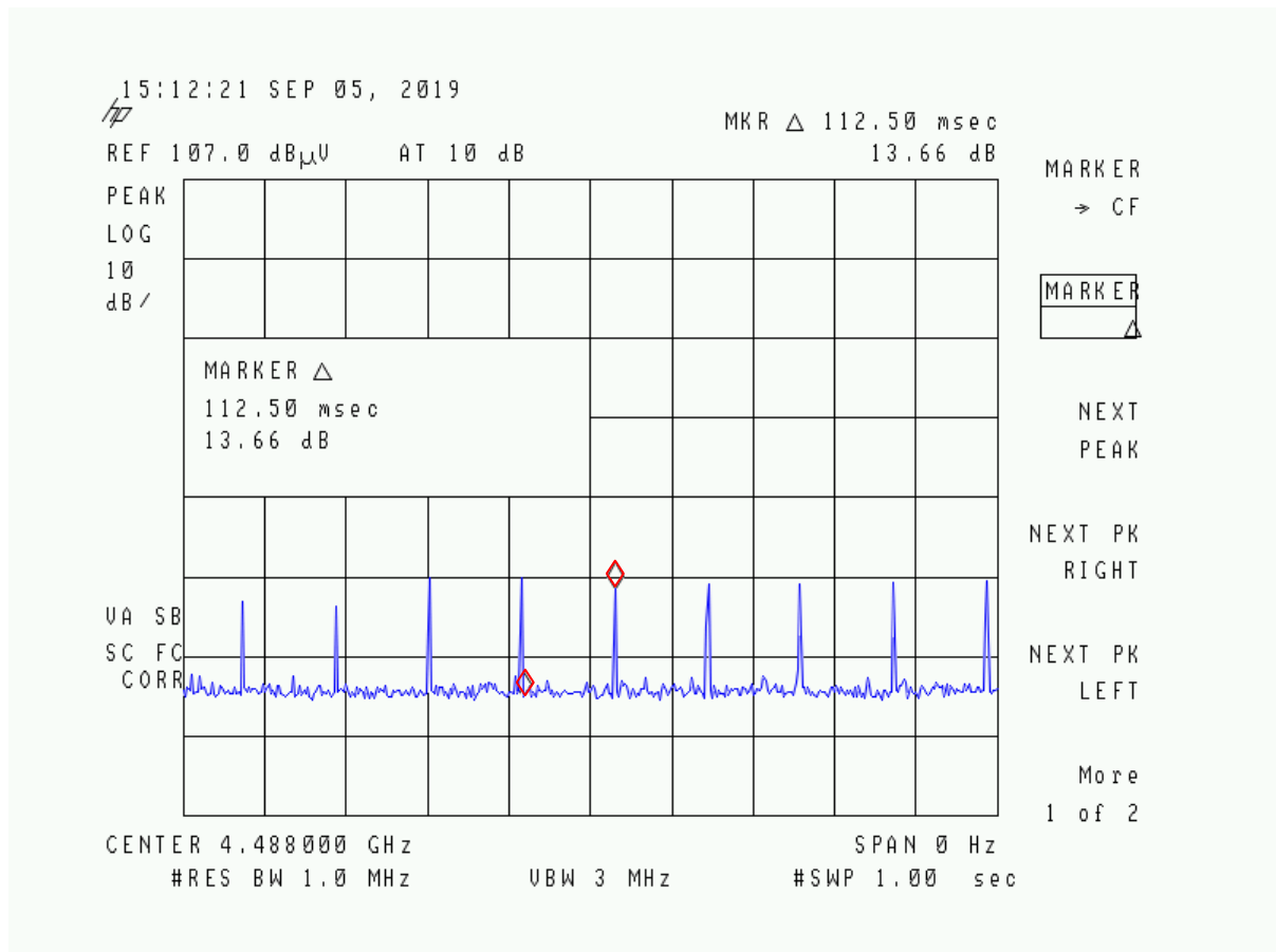
Figure 2. Full Period Measurement
