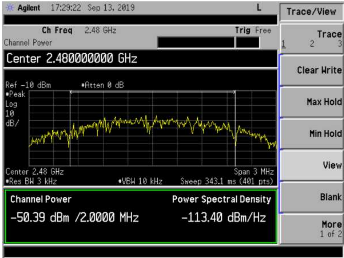
Figure 13. Power Spectral Density, High Channel
