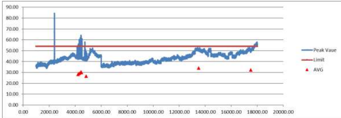
Figure 16. Radiated Emissions Graphical Data, TX, 1 -18GHz - Horizontal
