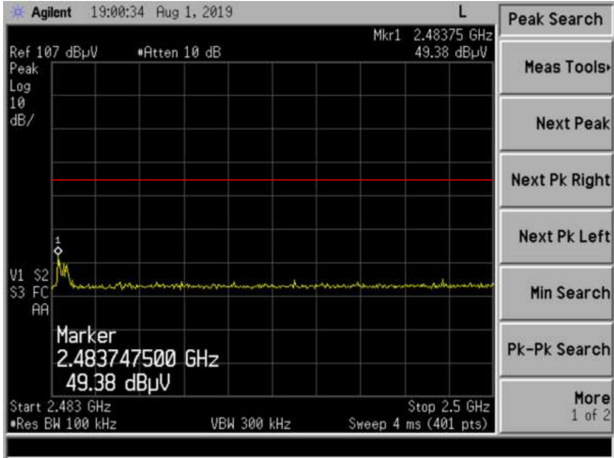
Figure 6. High Channel Restricted Band – Peak
