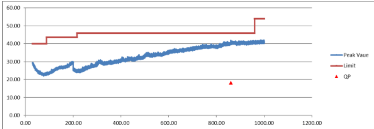
Figure 14. Radiated Emissions Graphical Data, TX, 30-1000 MHz - Horizontal
