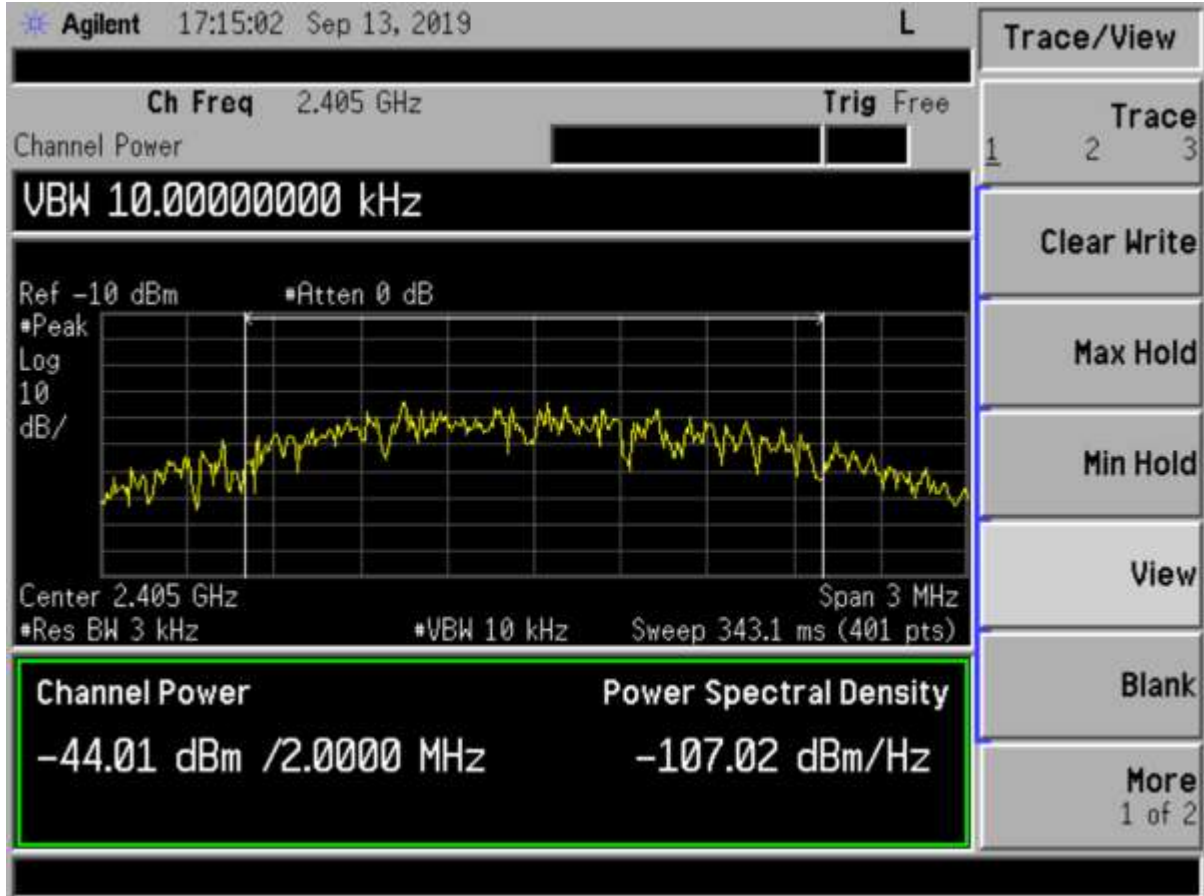
Figure 11. Power Spectral Density, Low Channel
