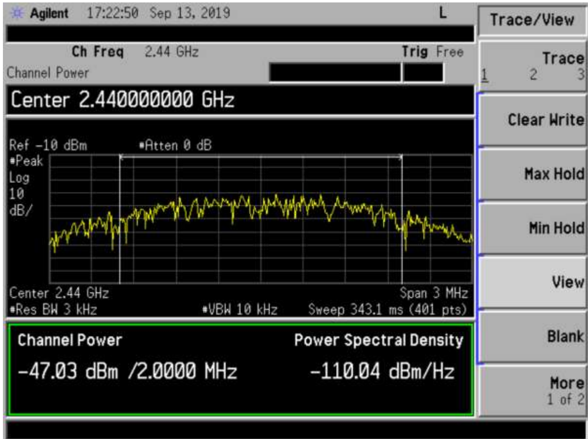
Figure 12. Power Spectral Density, Mid Channel
