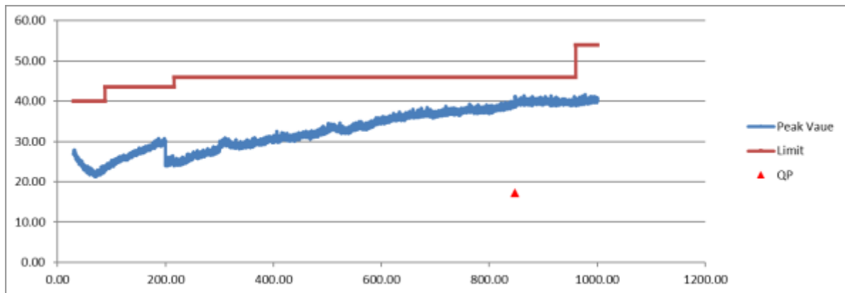
Figure 15. Radiated Emissions Graphical Data, TX, 30-1000 MHz – Vertical
