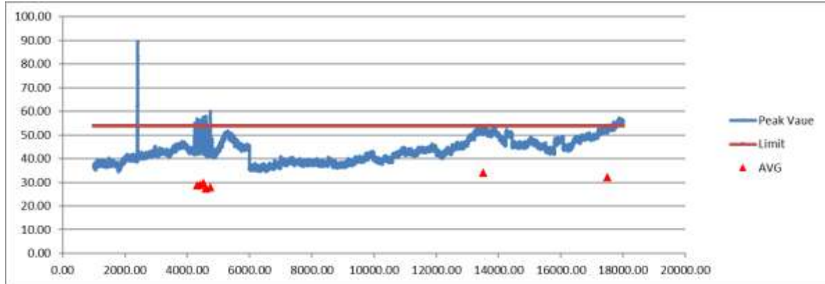
Figure 17. Radiated Emissions Graphical Data, TX, 1 -18GHz - Vertical
