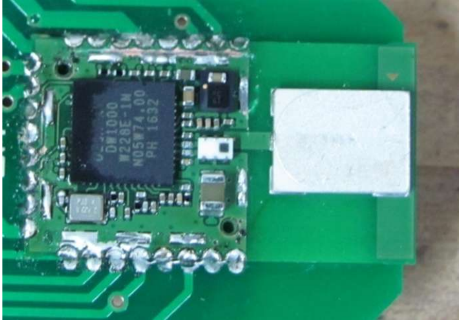
Figure 6. UWB with Shield Removed
