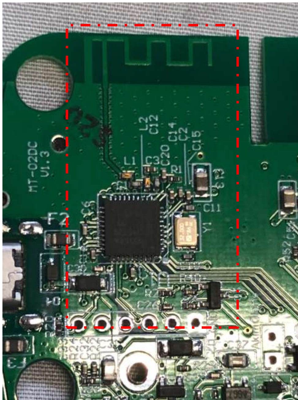
Figure 4. Zigbee Radio Module Circuit
