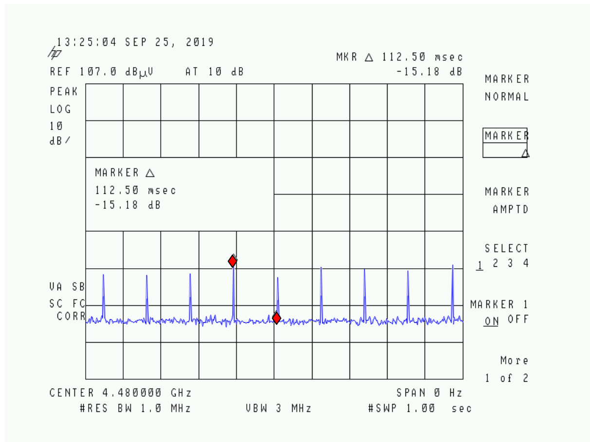
Figure 2. Duty Cycle Plot (TX OFF)
