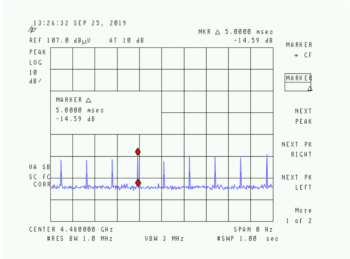
Figure 3. Duty Cycle Plot (TX ON) Single Pulse Width
