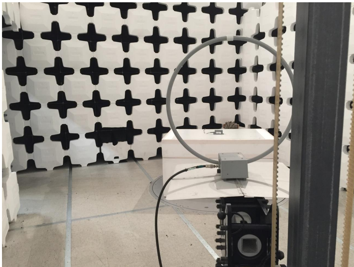
Figure 2. Radiated Emissions Test Configuration (9 kHz – 30 MHz)
