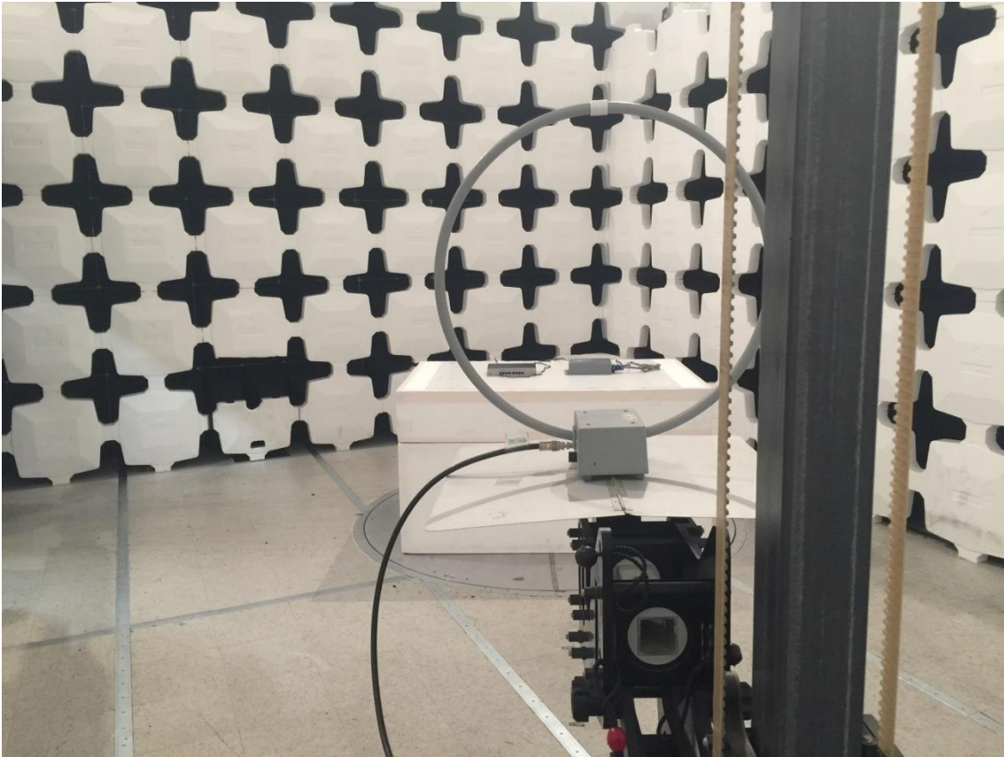
Figure 2. Radiated Emissions Test Configuration (Below 30 MHz)
