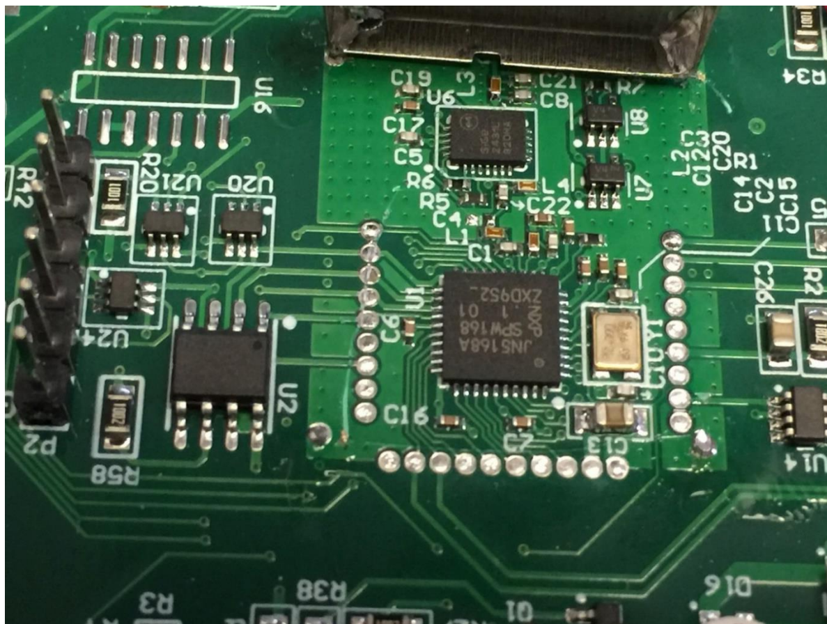
Figure 6. Zigbee Radio Close-up, Cover Removed
