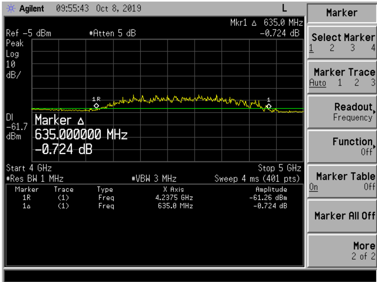
Figure 5. UWB f_L , f_M , f_H Measurement Plot
