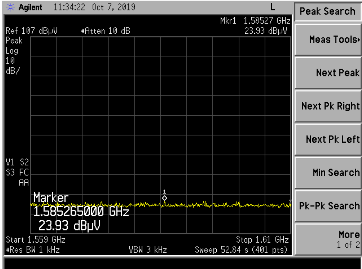
Figure 8. 1559 - 1610 MHz GPS Band
