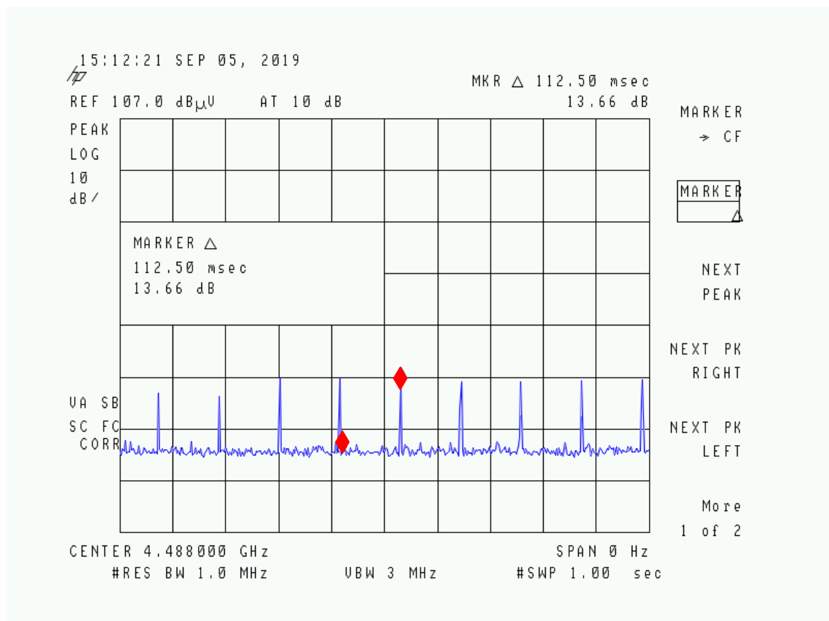
Figure 3. Duty Cycle Plot (TX OFF)
