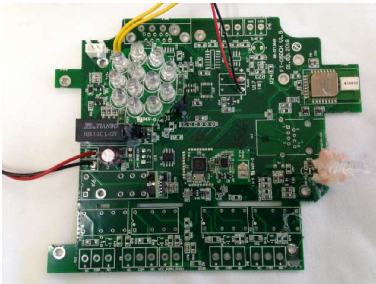
Figure 3. EUT, Top of PCB
