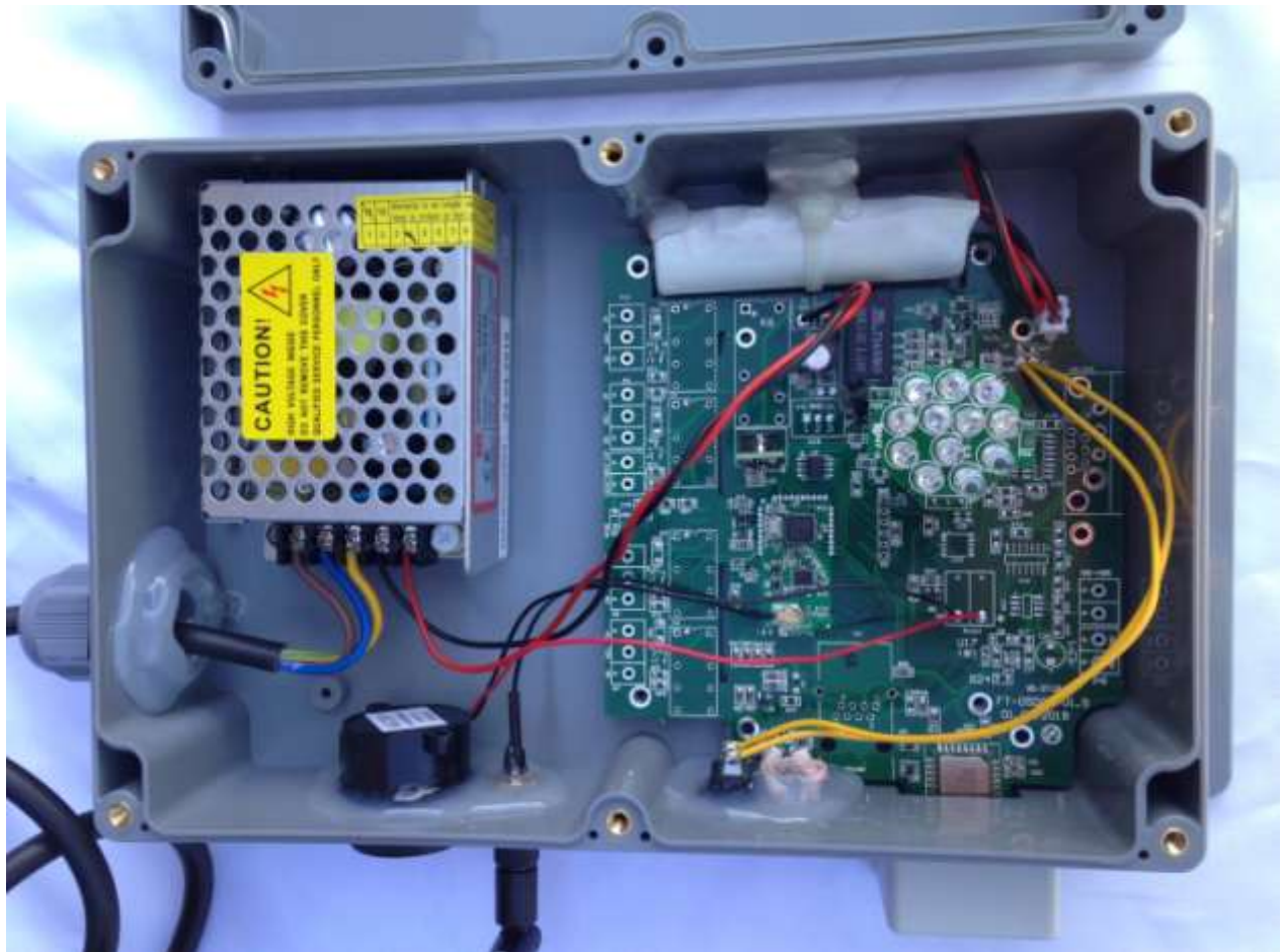
Figure 2. EUT, Internal Electronics
