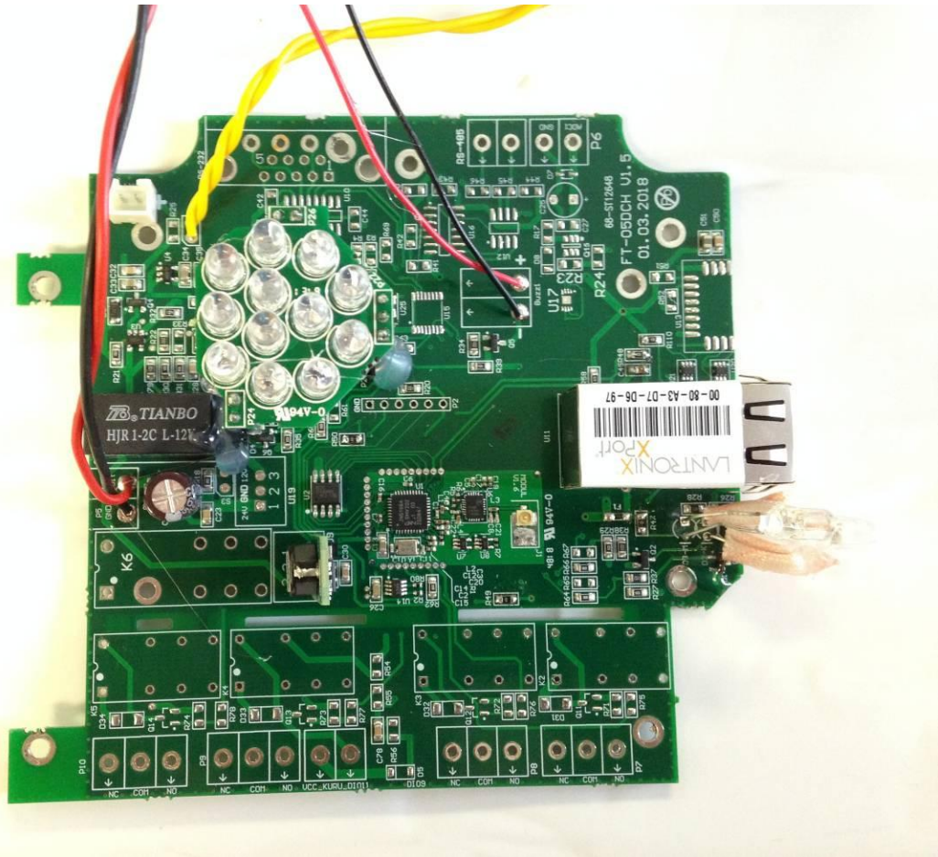
Figure 2. Top of PCB
