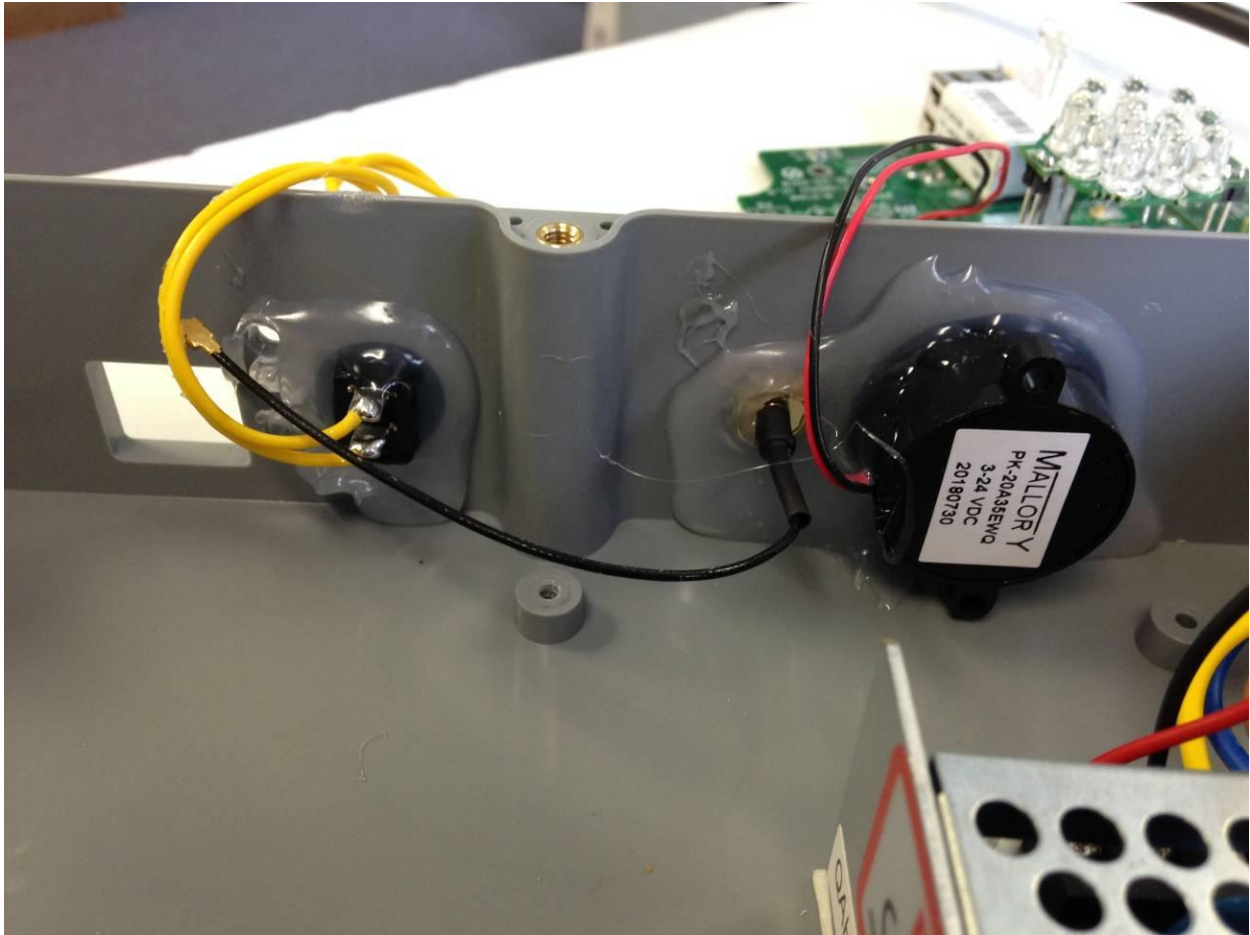
Figure 7. Buzzer, Battery Power Switch and RF Connector
