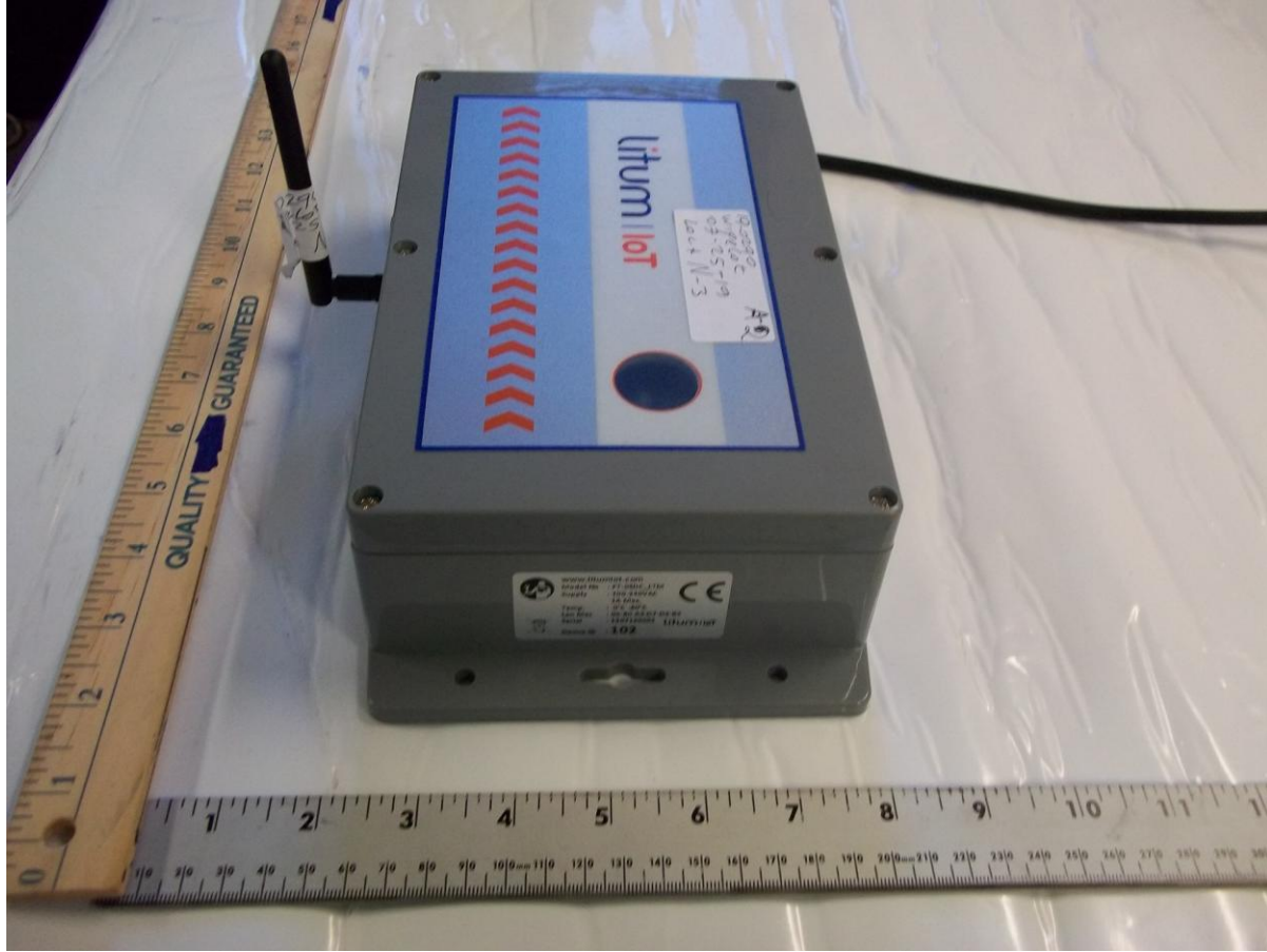
Figure 5. EUT, Side 1 View
