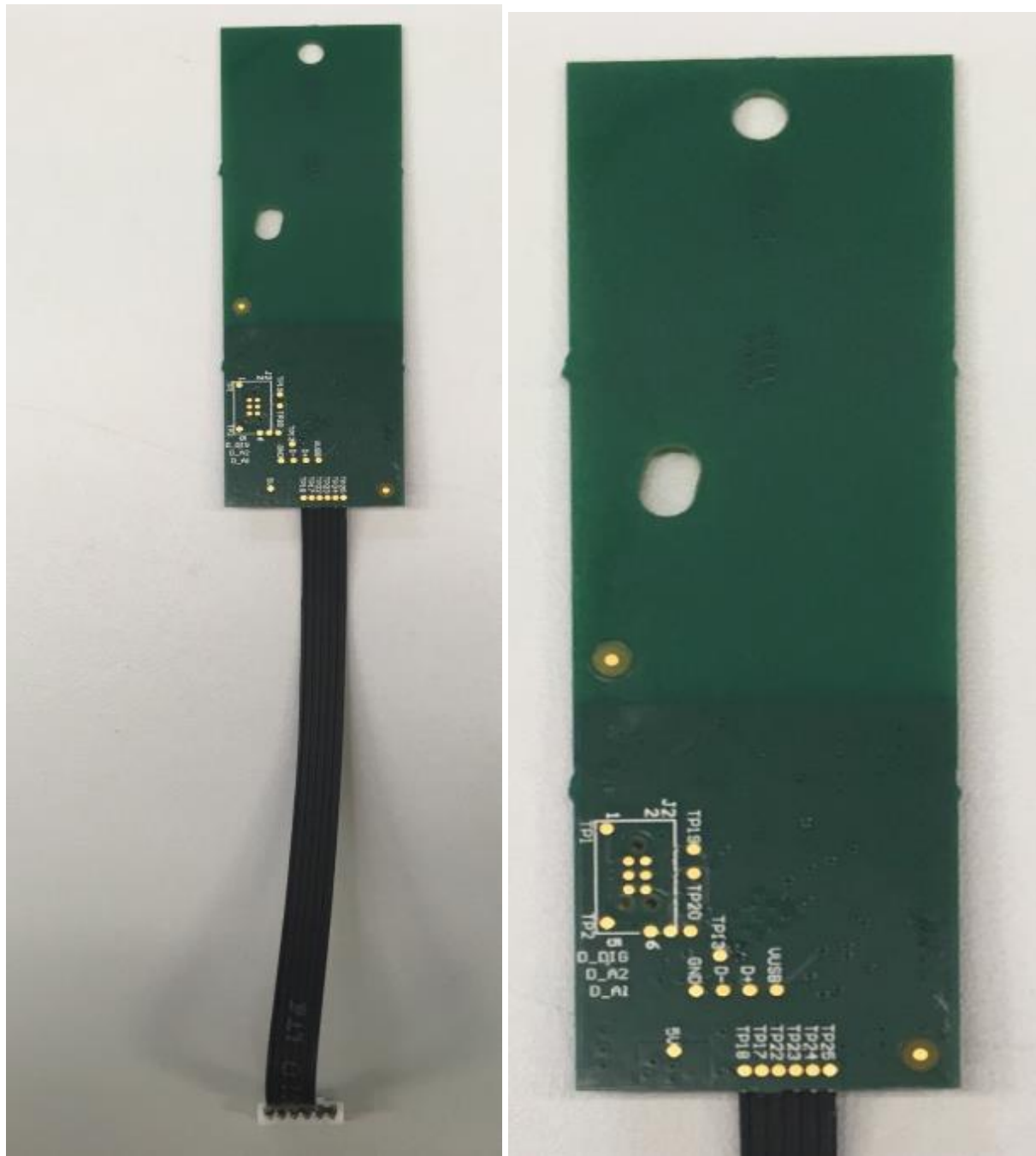
NFC Base Station Board Bottom Side View + detail
