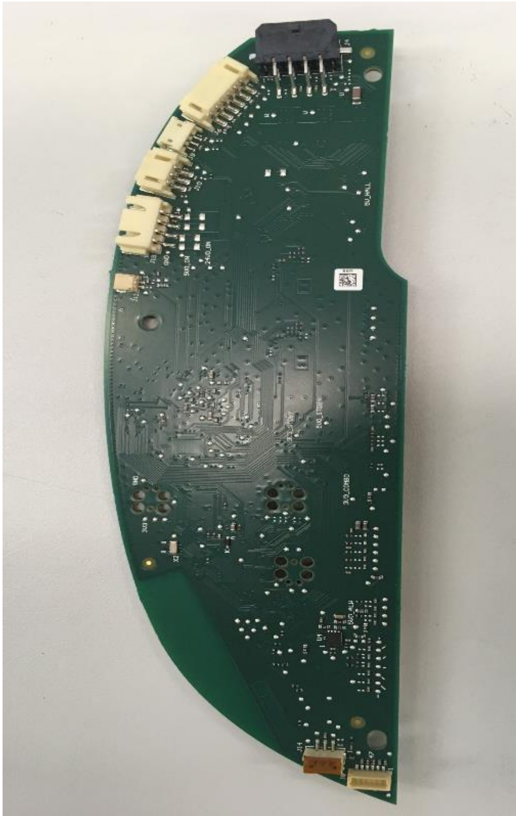
Main Board Bottom Side View
