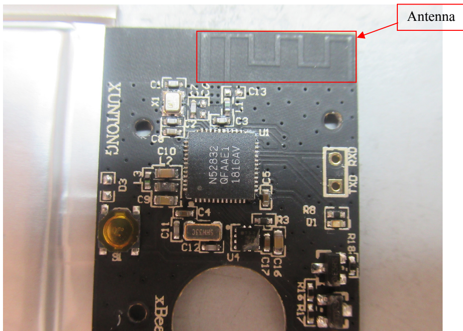
EUT –IC Chip View
