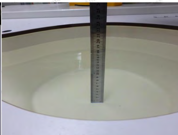
Photo of 5000MSL Liquid Height for Body SAR
