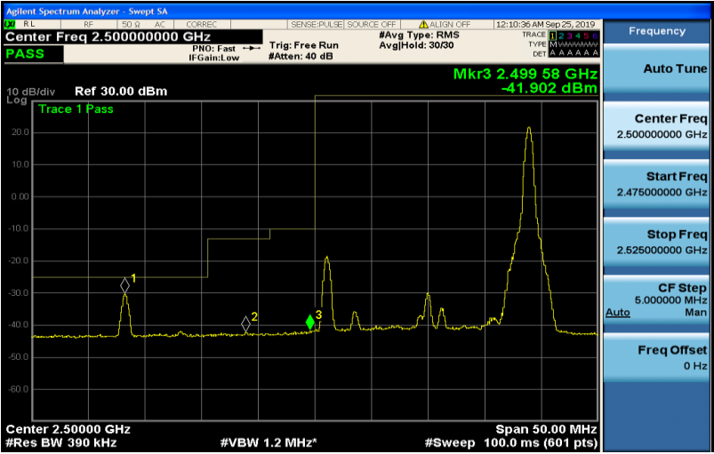
Band7-20MHz-QPSK-20850-100RB#0
