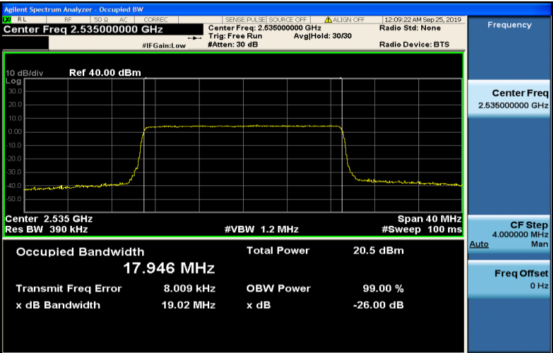
Band7-20MHz-16QAM-21350-100RB#0-17.946
