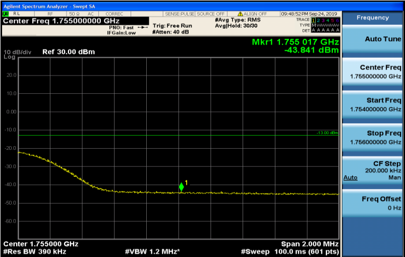
Band4-20MHz-16QAM-20300-1RB#99
