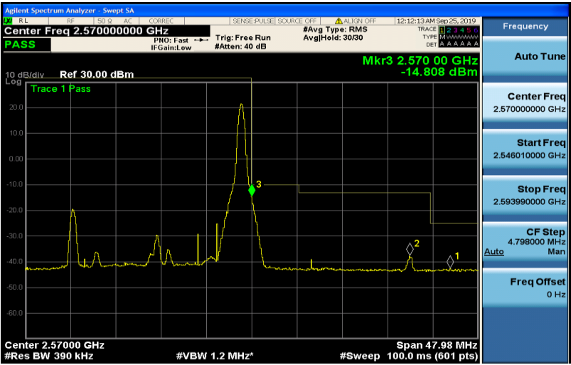
Band7-20MHz-QPSK-21350-100RB#0
