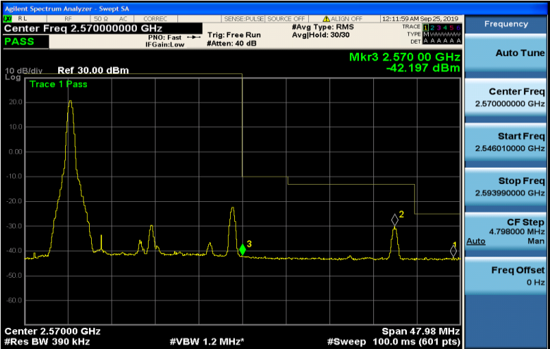
Band7-20MHz-16QAM-21350-1RB#99
