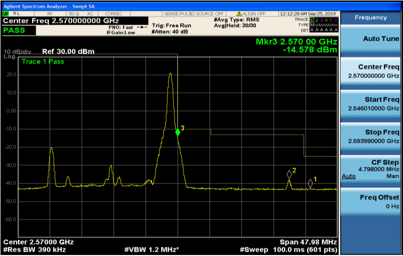
Band7-20MHz-16QAM-21350-100RB#0
