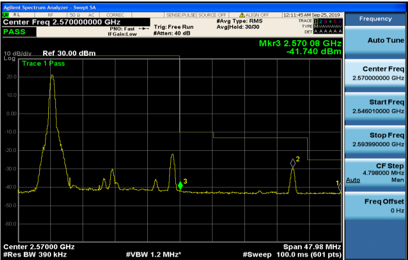
Band7-20MHz-QPSK-21350-1RB#99
