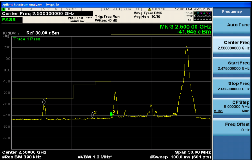
Band7-20MHz-16QAM-20850-100RB#0
