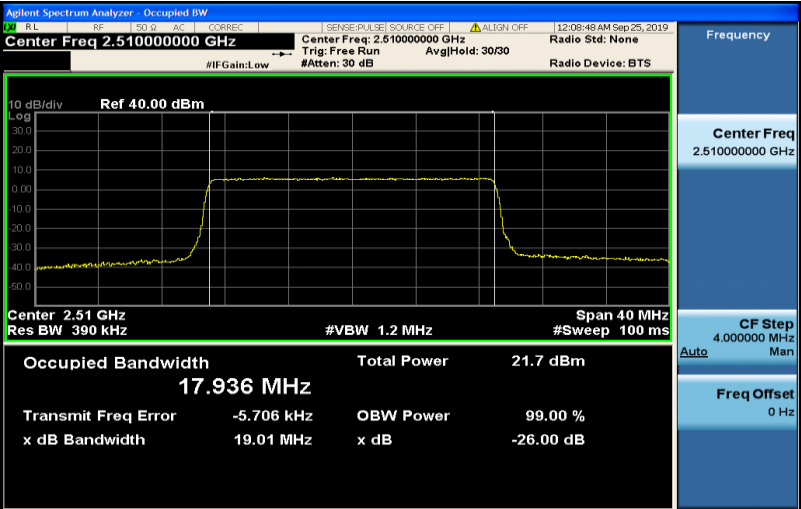
Band7-20MHz-QPSK-21100-100RB#0-17.936
